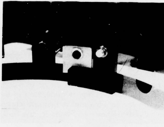
Figure 6. Infra-red retro reflective sensor Hall effect sensor metal target with magnet plastic target.
