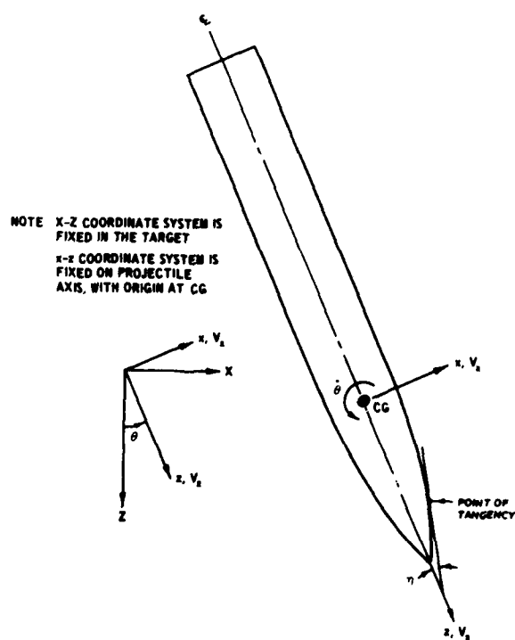
Figure 2.1 Projectile motion in two dimensions.
