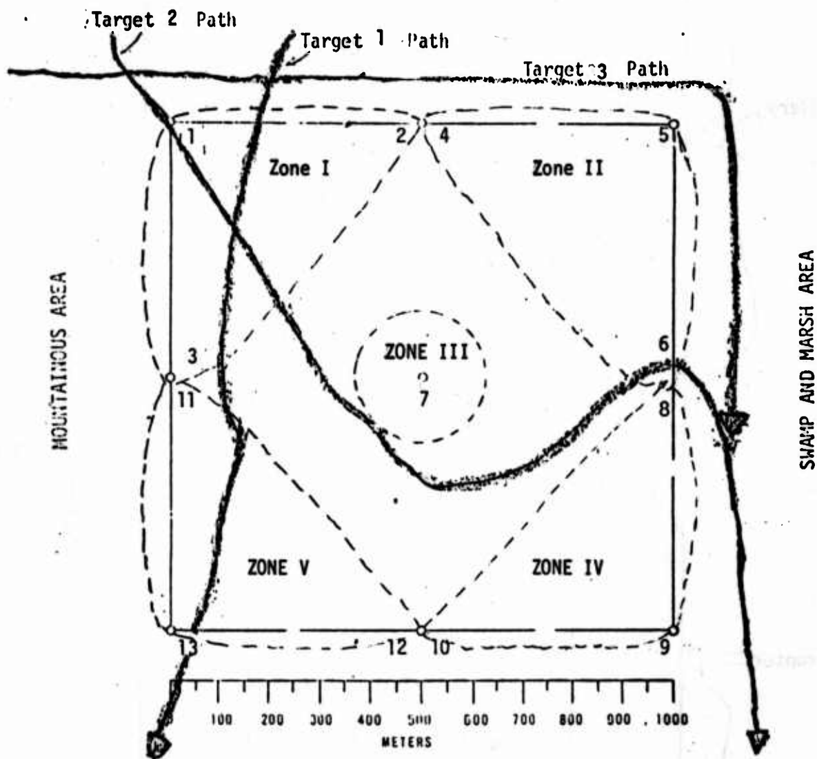
Figure A-13. Sketch map for zone patching using a 9-sensor grid.
