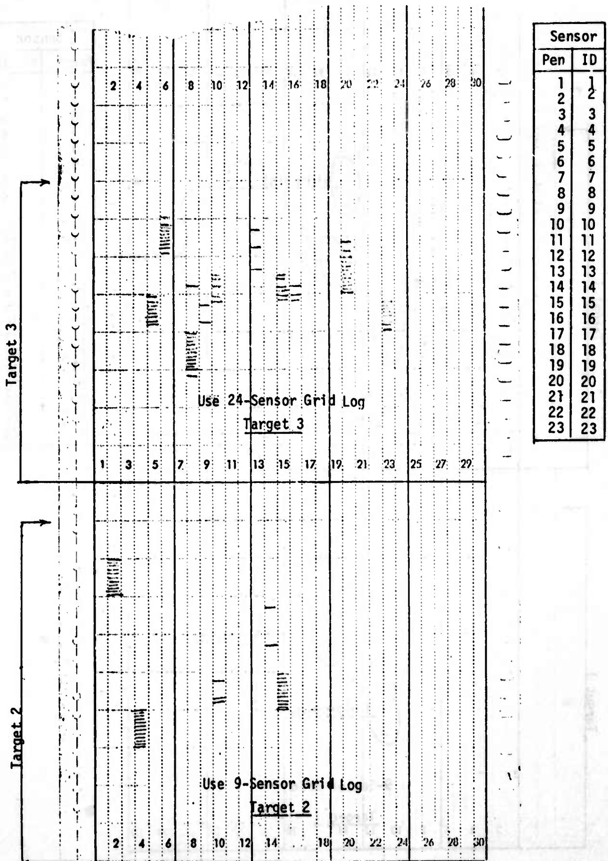
Figure 4. X-T plots of target 2 activations.
