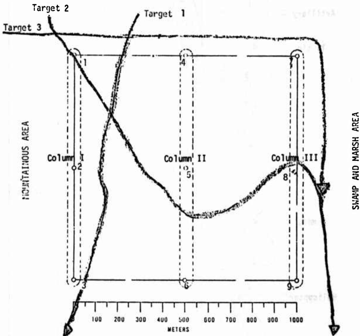
Figure A-1. Sketch map for column patching using a 9-sensor grid.
