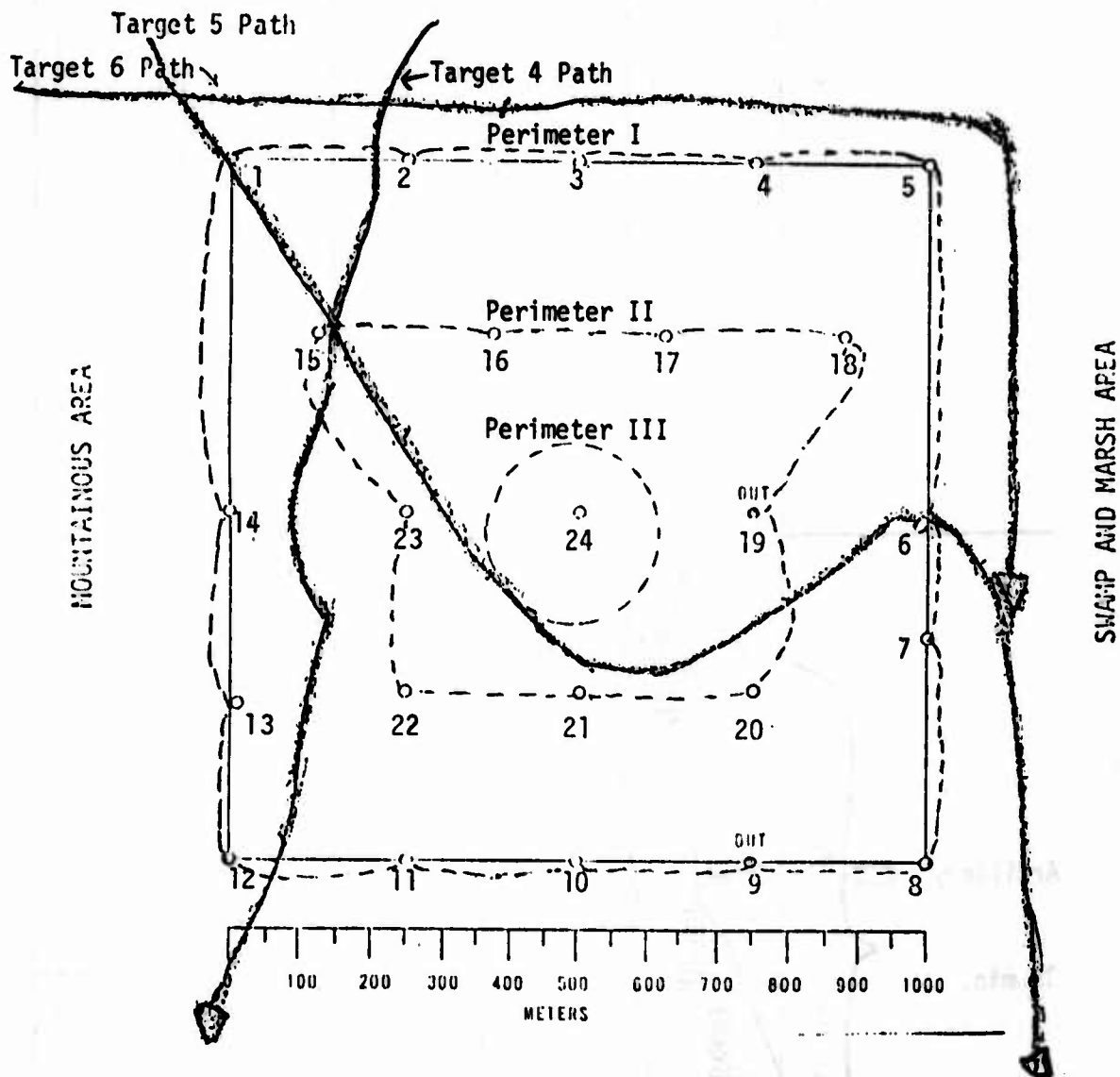
Figure A-7. Sketch map for perimeter patching using a 24-sensor grid.
