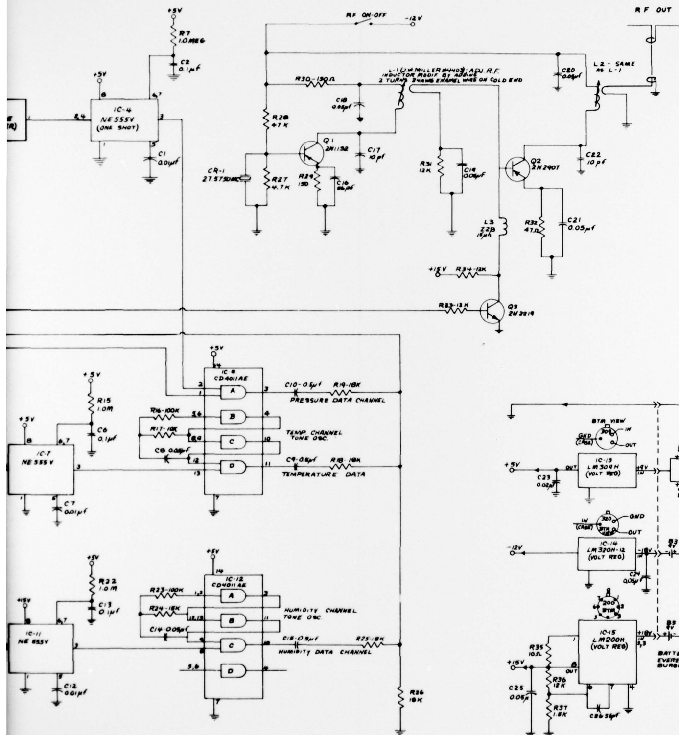
Diagram of boundary layer sonde sensing and transmitting system
