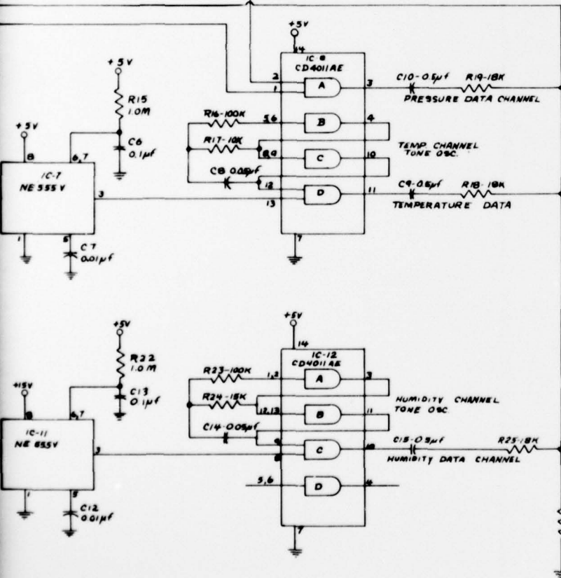
Diagram of boundary layer sonde sensing and transmitting system
