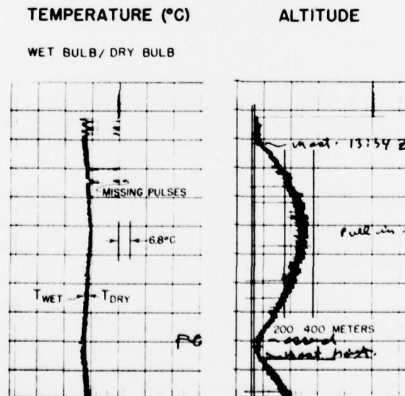
Fig. 10—Reproduction of the actual analog stripchart recording of dry-bulb temperature, wet-bulb temperature, and altitude from a boundary layer sonde operating from USNS Hayes during a cruise in 1977
