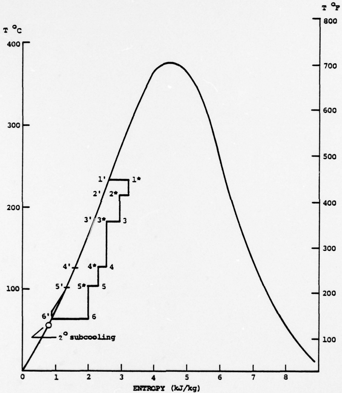
Figure 2. Single Component Biphasic Cycle
