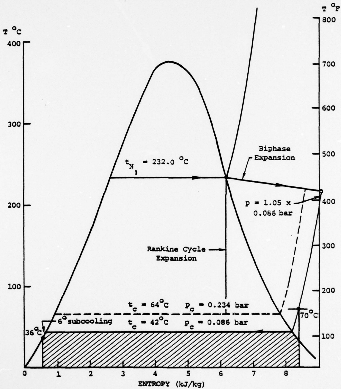
Figure 1. Comparison of Rankine Cycle and Two-Component Biphase Cycle
