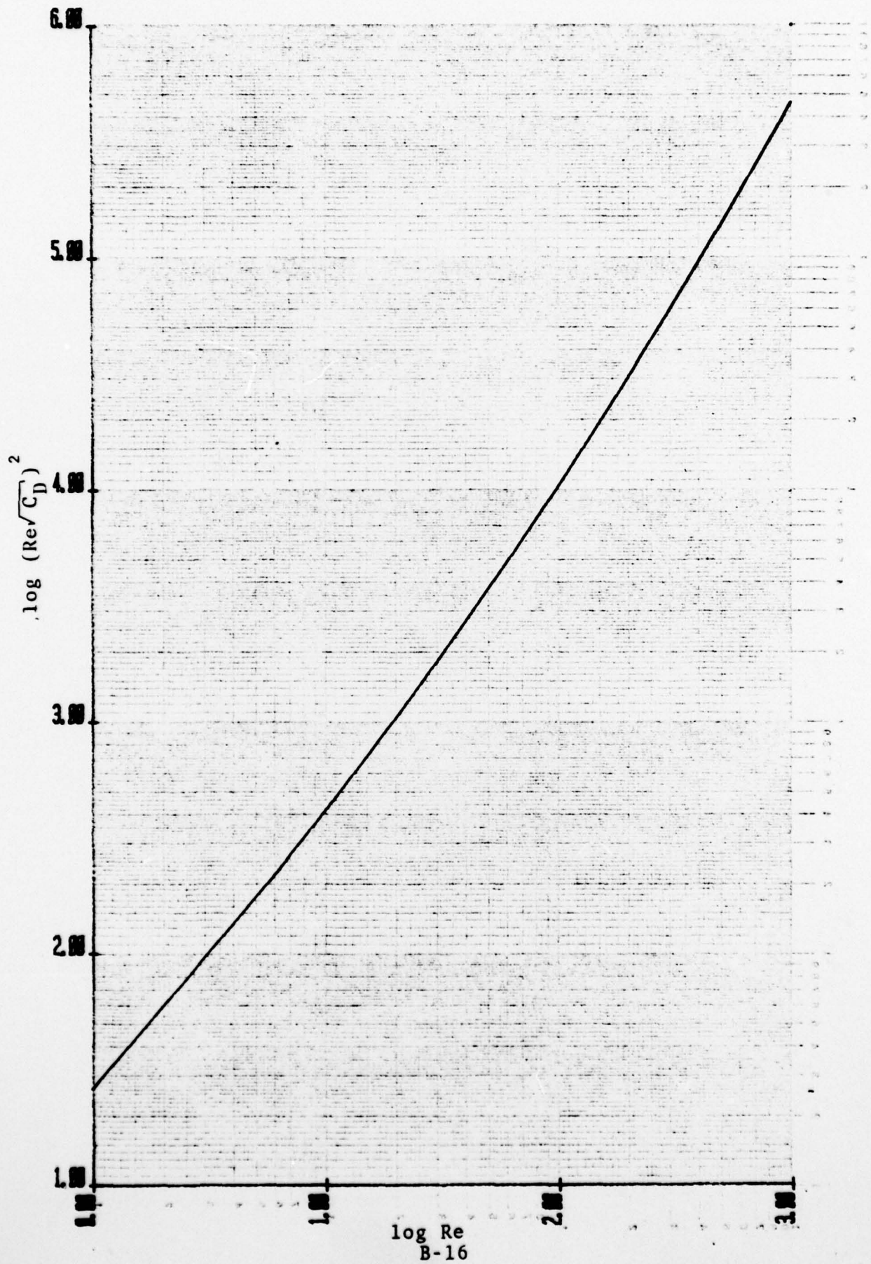
Figure B-3. Dwell Characteristics of Spherical Droplets (Rotating Heat Exchangers)
