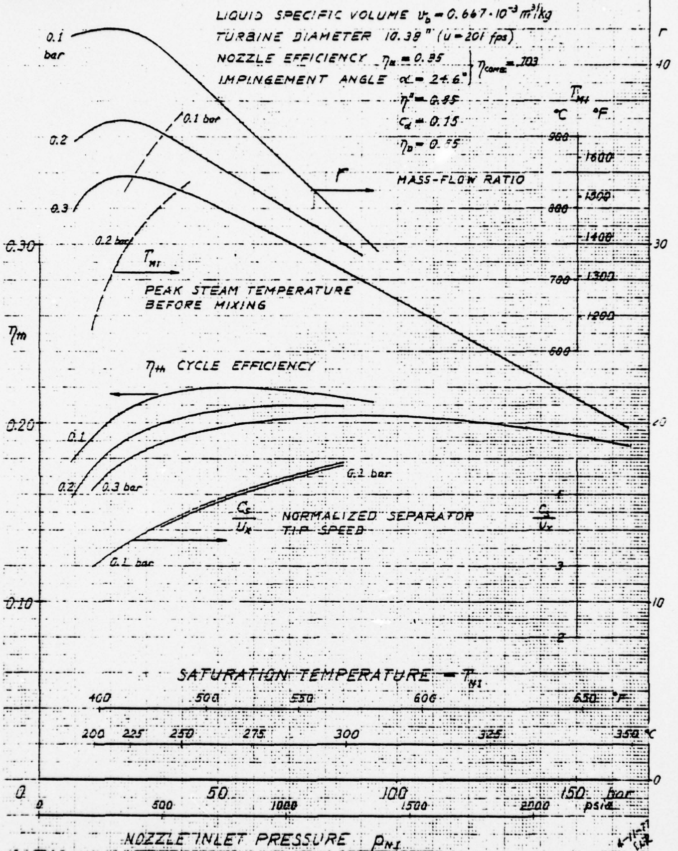
Figure 20. Cycle Performance of Basic Biphasic System (Roto-Pitot)
