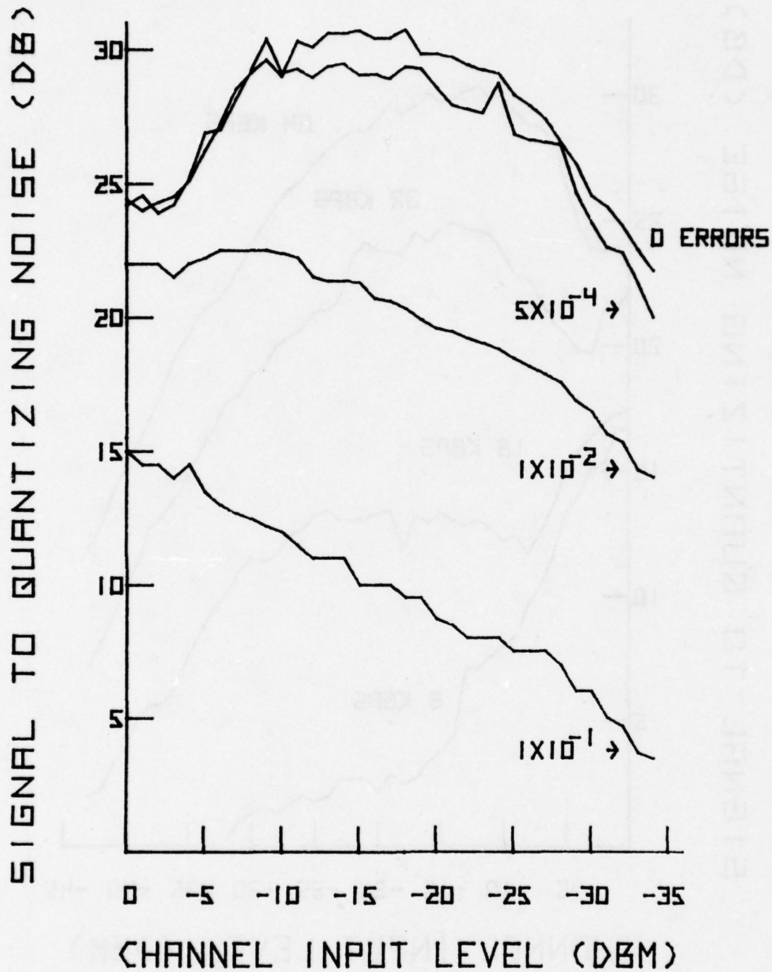
FIGURE 27A. SIGNAL TO QUANTIZING NOISE CHARACTERISTICS (64 KBPS)
