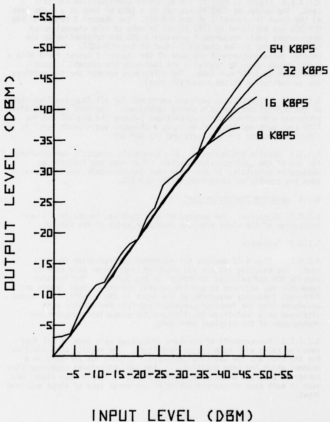
FIGURE 10. LINEARITY LOGCVSD
