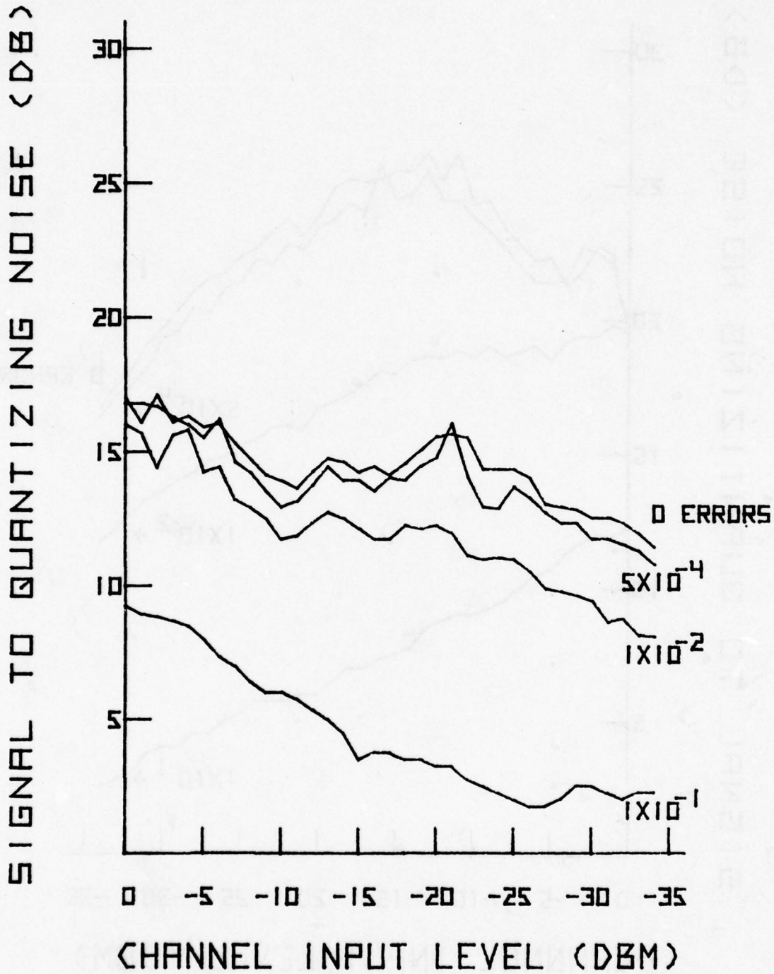
FIGURE 27C. SIGNAL TO QUANTIZING NOISE CHARACTERISTICS (16 KBPS)
