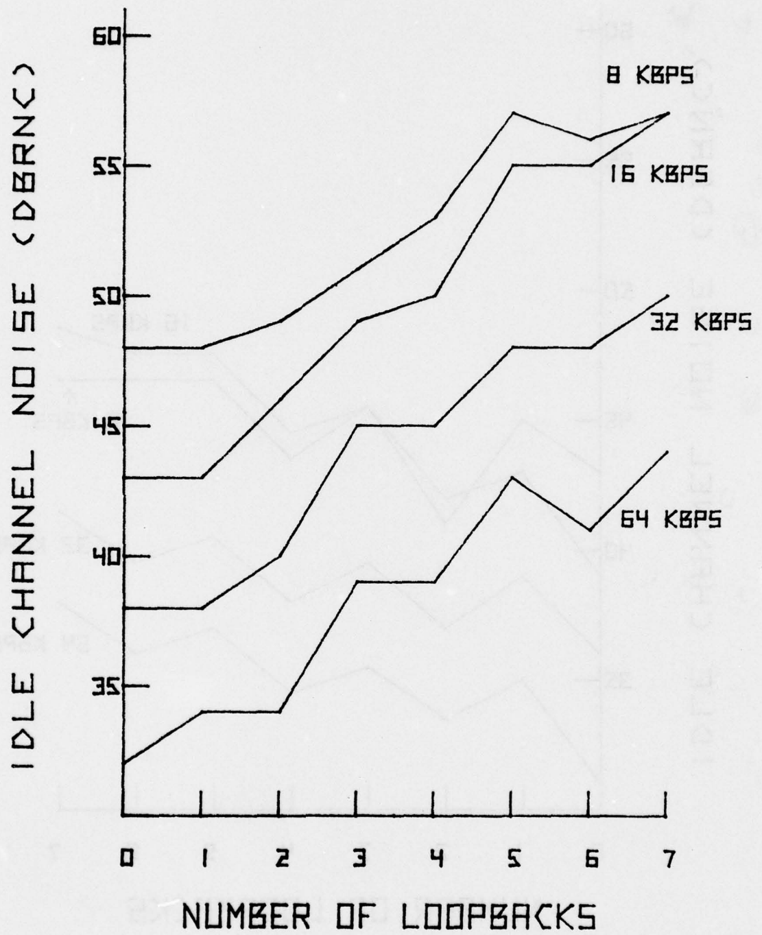
FIGURE 24. LOOP TEST RESULTS, (VSD)
