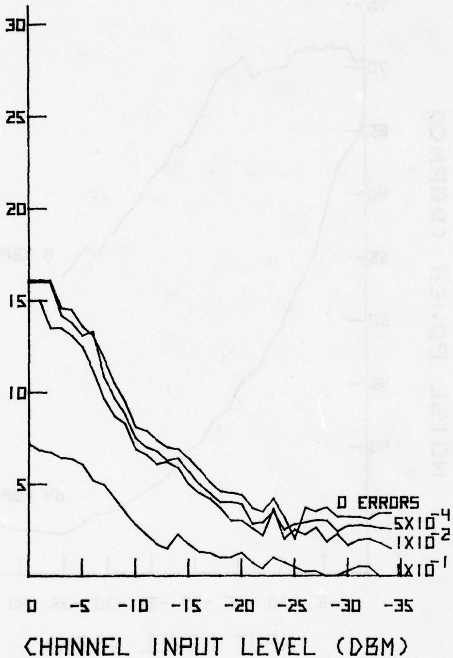
FIGURE 27D. SIGNAL TO QUANTIZING NOISE CHARACTERISTICS ( 8 KBPS)
