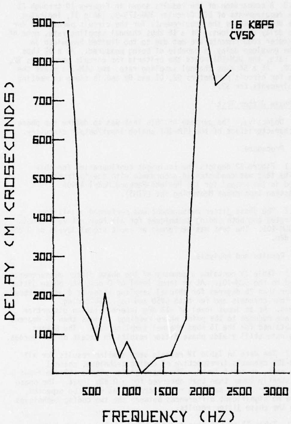
FIGURE 21. ENVELOPE DELAY VS FREQUENCY
