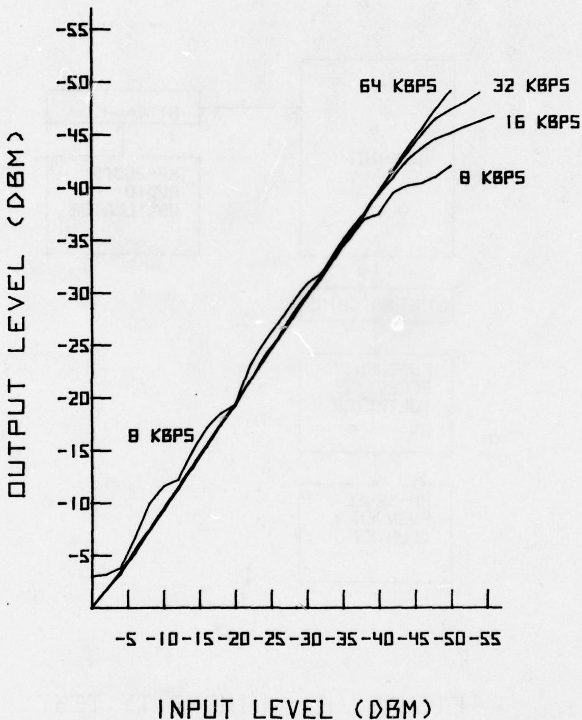
FIGURE 9. LINEARITY (VSD)
