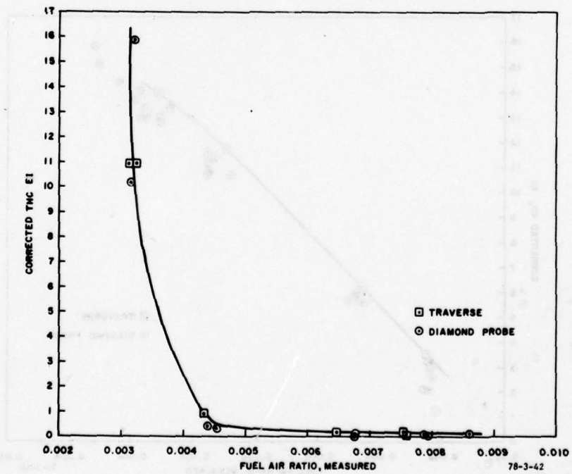
FIGURE 42. THC EI--DIAMOND PROBE--2-INCH LOCATION
