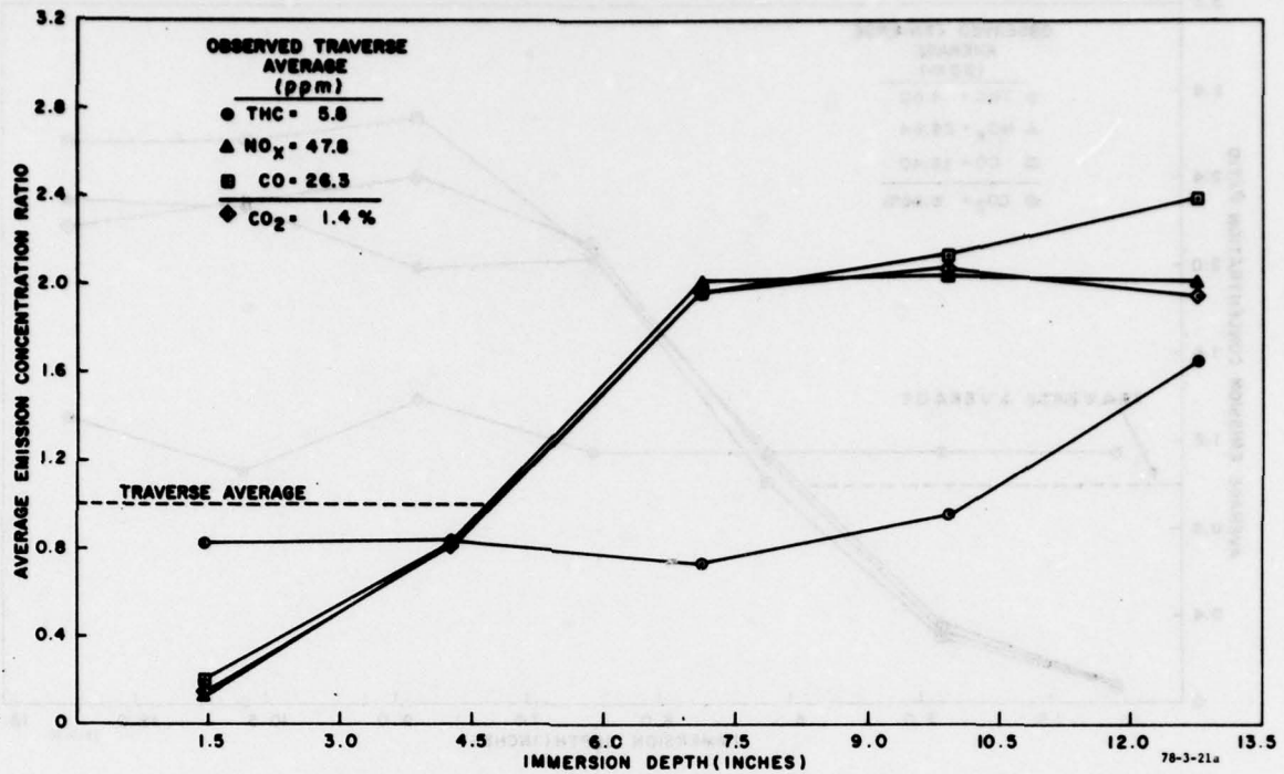
FIGURE 21(a). EMISSION CONCENTRATION DISTRIBUTION--45°-- MAXIMUM CONTINUOUS POWER
