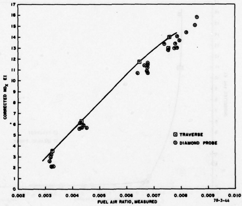
FIGURE 44. NO x EI--DIAMOND PROBE--2-INCH LOCATION
