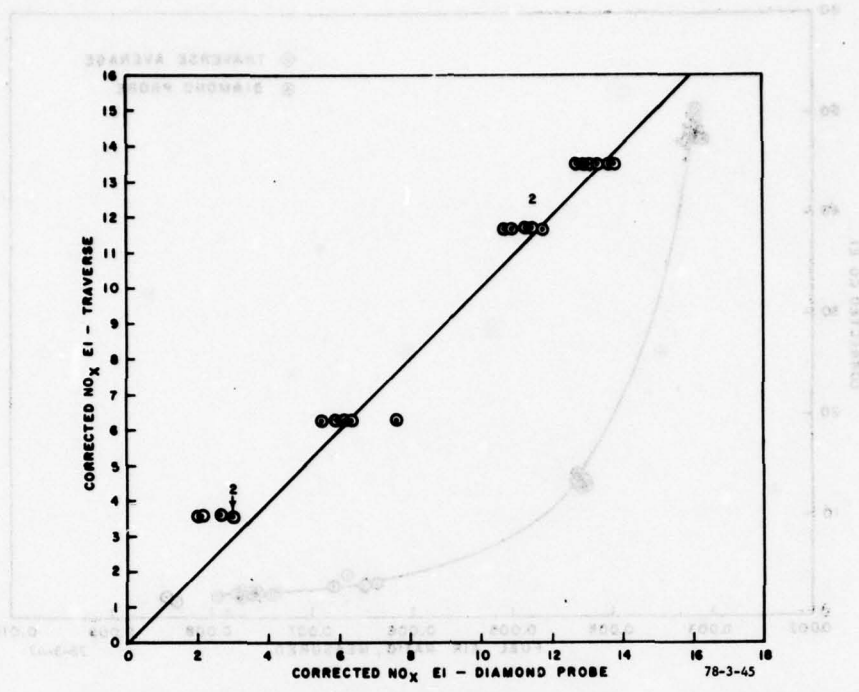
FIGURE 45. NO x EI--RELATION BETWEEN TRAVERSE AND DIAMOND PROBE--2-INCH LOCATION
