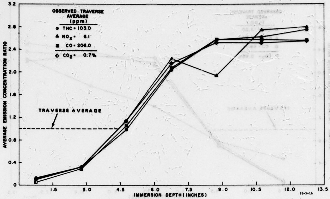
FIGURE 16(a). EMISSION CONCENTRATION DISTRIBUTION--90°--IDLE POWER
