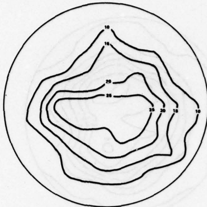
A. AVERAGE THC = 13.2 ppm CORRECTED THC = 0.93 EI
