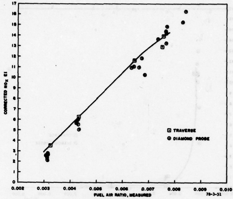
FIGURE 51. NO x EI—DIAMOND PROBE—7-INCH LOCATION
