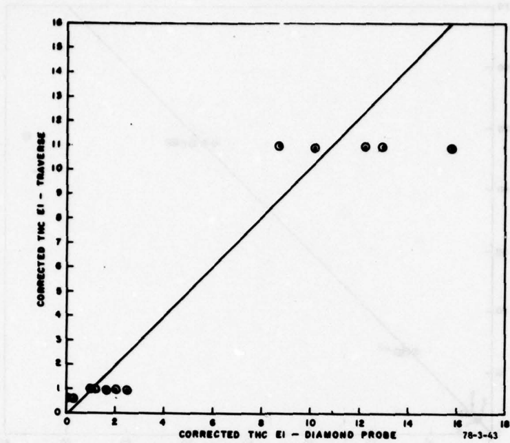
FIGURE 43. THC EI--RELATION BETWEEN TRAVERSE AND DIAMOND PROBE--2-INCH LOCATION
