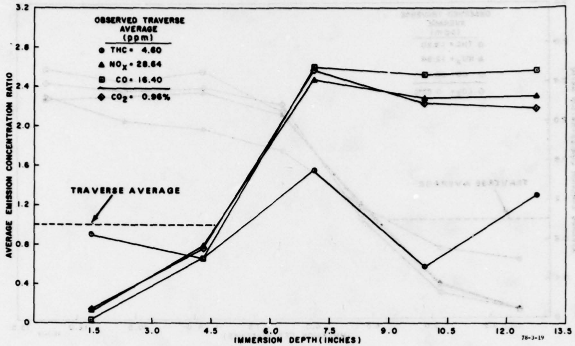
FIGURE 19(a). EMISSION CONCENTRATION DISTRIBUTION--45°--CRUISE POWER
