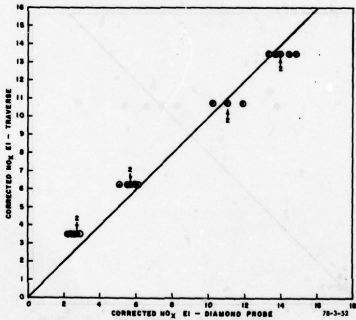
FIGURE 52. NO x EI—RELATION BETWEEN TRAVERSE AND DIAMOND PROBE—7-INCH LOCATION
