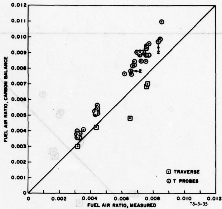
FIGURE 35. FUEL-TO-AIR RATIOS--T PROBES--63-PERCENT RADIUS--2-INCH LOCATION
