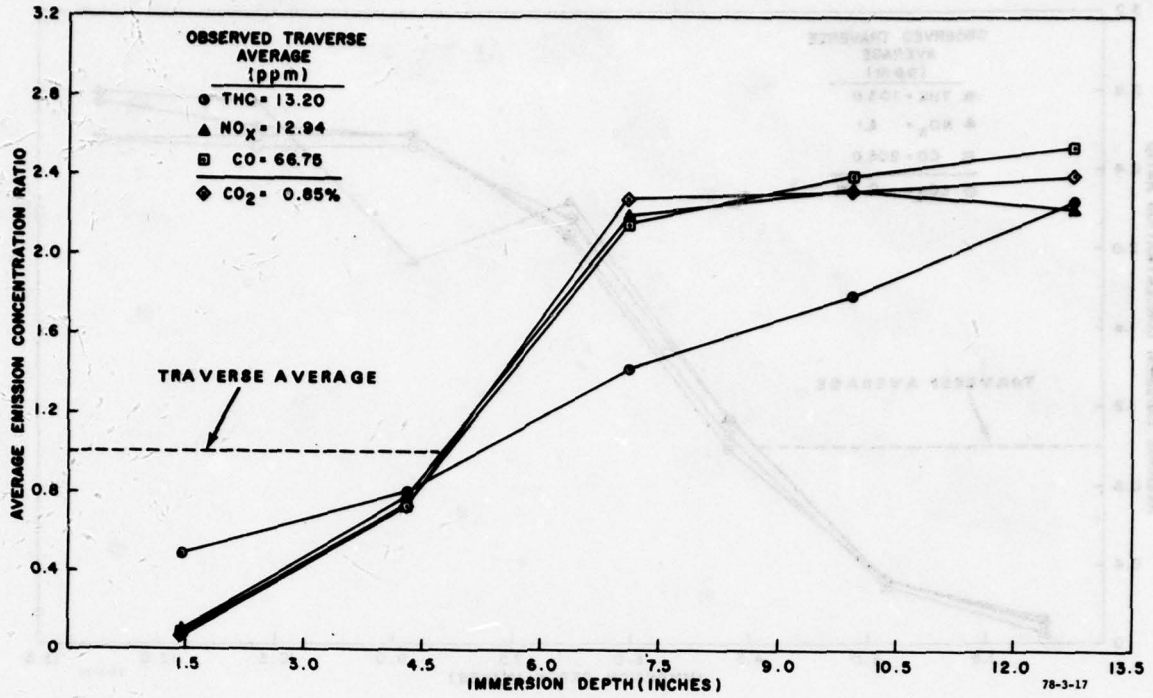
FIGURE 17(a). EMISSION CONCENTRATION DISTRIBUTION--45°--APPROACH POWER
