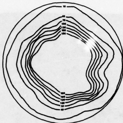
A. AVERAGE THC = 103 ppm CORRECTED THC = 10.90 EI
