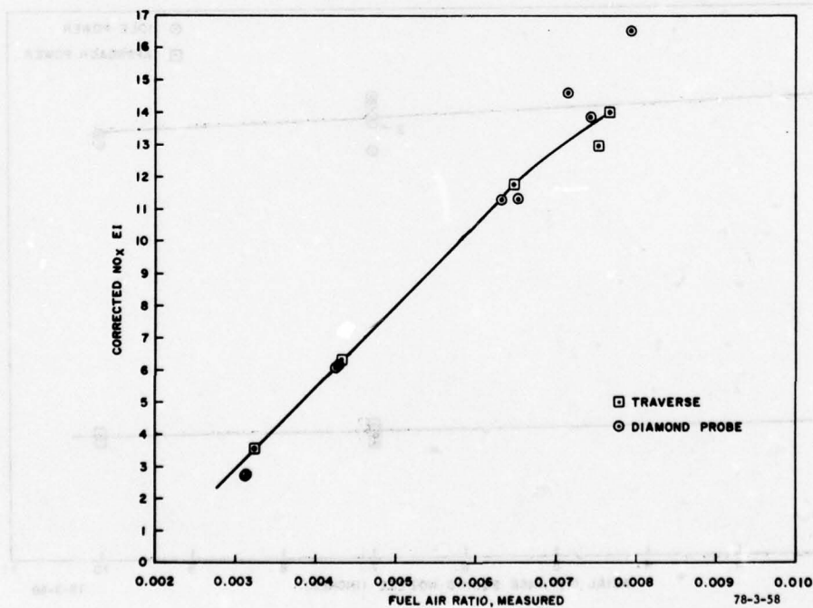
FIGURE 58. NO x EI--DIAMOND PROBE--10-INCH LOCATION
