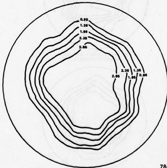
FIGURE 11. EXHAUST EMISSION TRAVERSE MAPS--MAXIMUM CONTINUOUS POWER
