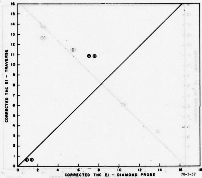
FIGURE 57. THC EI--RELATION BETWEEN TRAVERSE AND DIAMOND PROBE--10-INCH LOCATION
