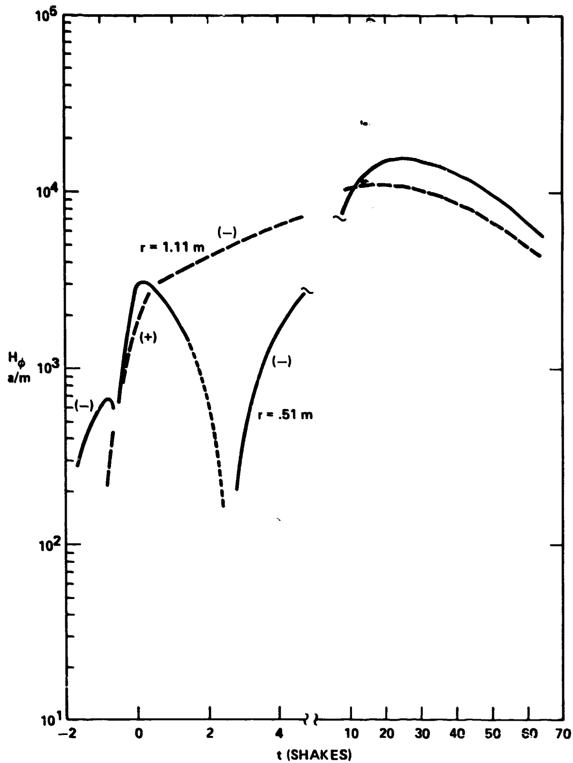
Figure 7. Time histories of the magnetic field at z = 3 m and the indicated radial depths
