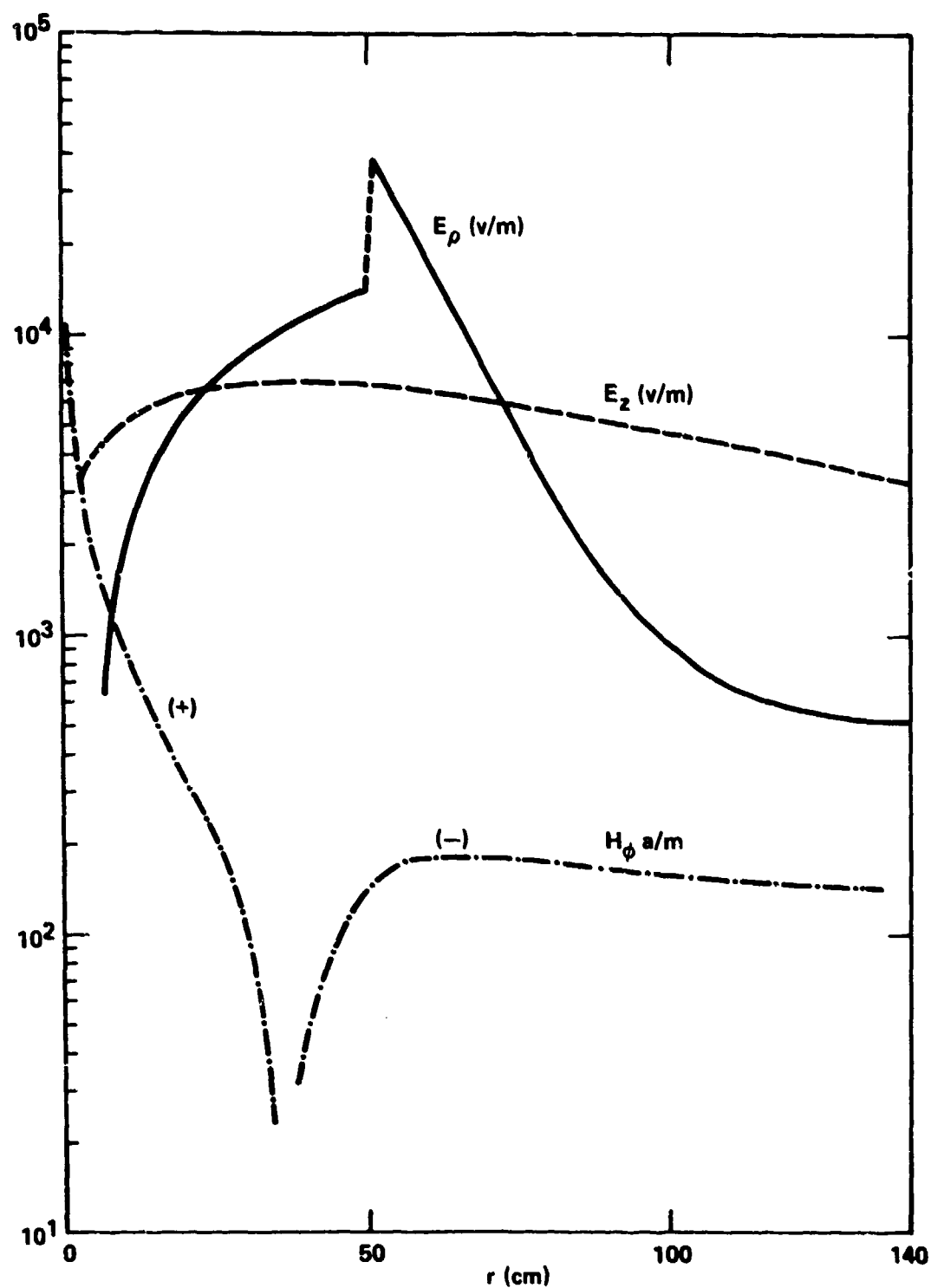
Figure 5. Fields as a function of radius at t = 1 \times 10^{-7} sec and z = 10 m
