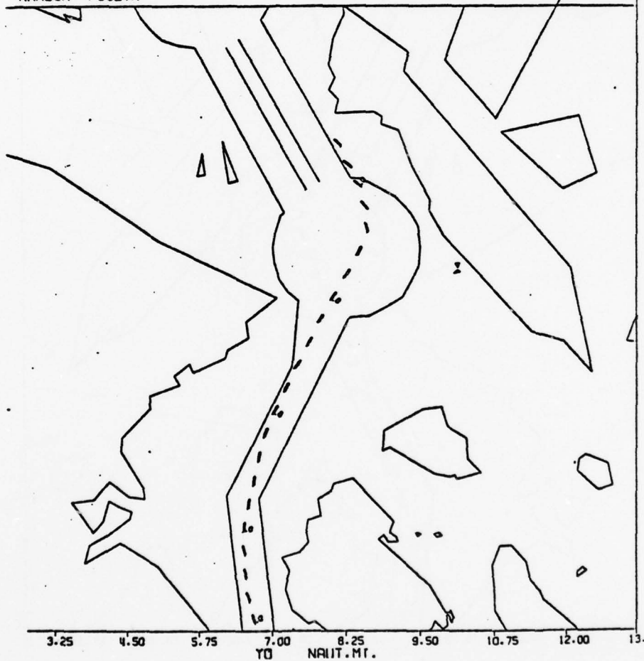
Figure 5-6. Ship Track Plots of Man-In-The-Loop Runs Through Rosario Strait (Part 8, 6 Knots)
