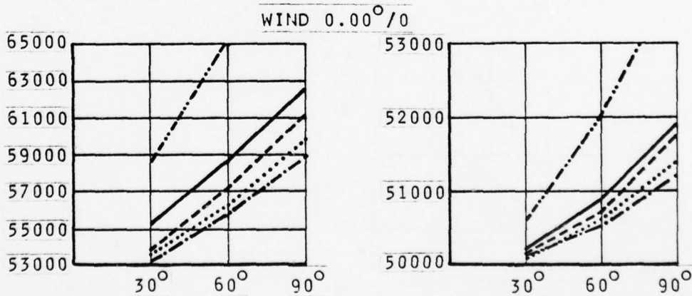
Figure 4-5. Advance and Transfer During Hard Right Rudder Turns, Failed Engine Runs, Initial Speed 4 kts
