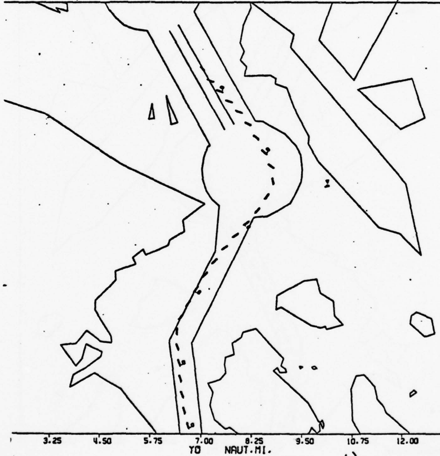
Figure 5-6. Ship Track Plots of Man-In-The-Loop Runs Through Rosario Strait (Part 2, 6 Knots)
