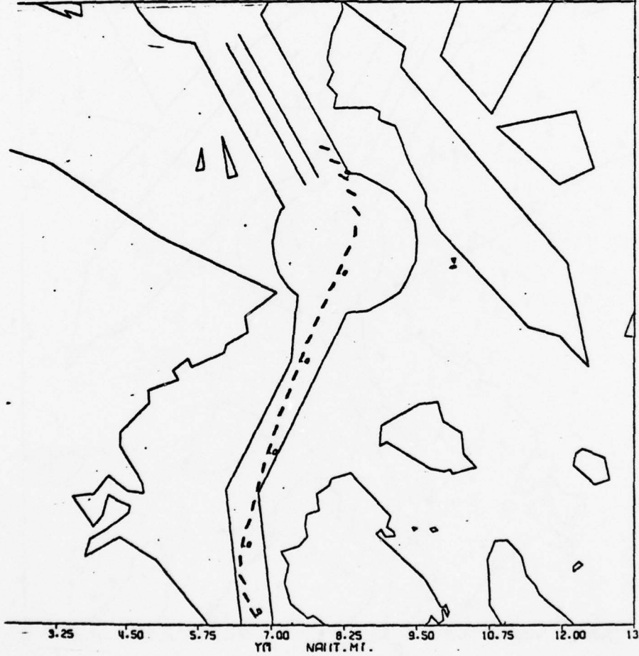
Figure 5-6. Ship Track Plots of Man-In-The-Loop Runs Through Rosario Strait (Part 7, 4 Knots)
