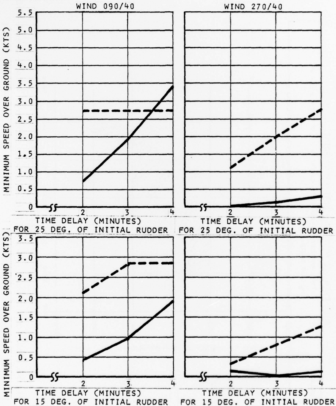
Figure 4-16. Minimum Speed Attained as a Function of Time Delay, Failed Engine Runs
