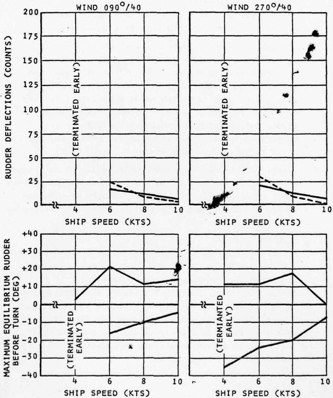
Figure 3-7. Rudder Data for Bellingham Channel (Part 2)
