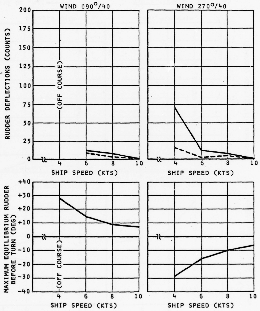
Figure 3-6. Rudder Data for Rosario Strait (Part 1)
