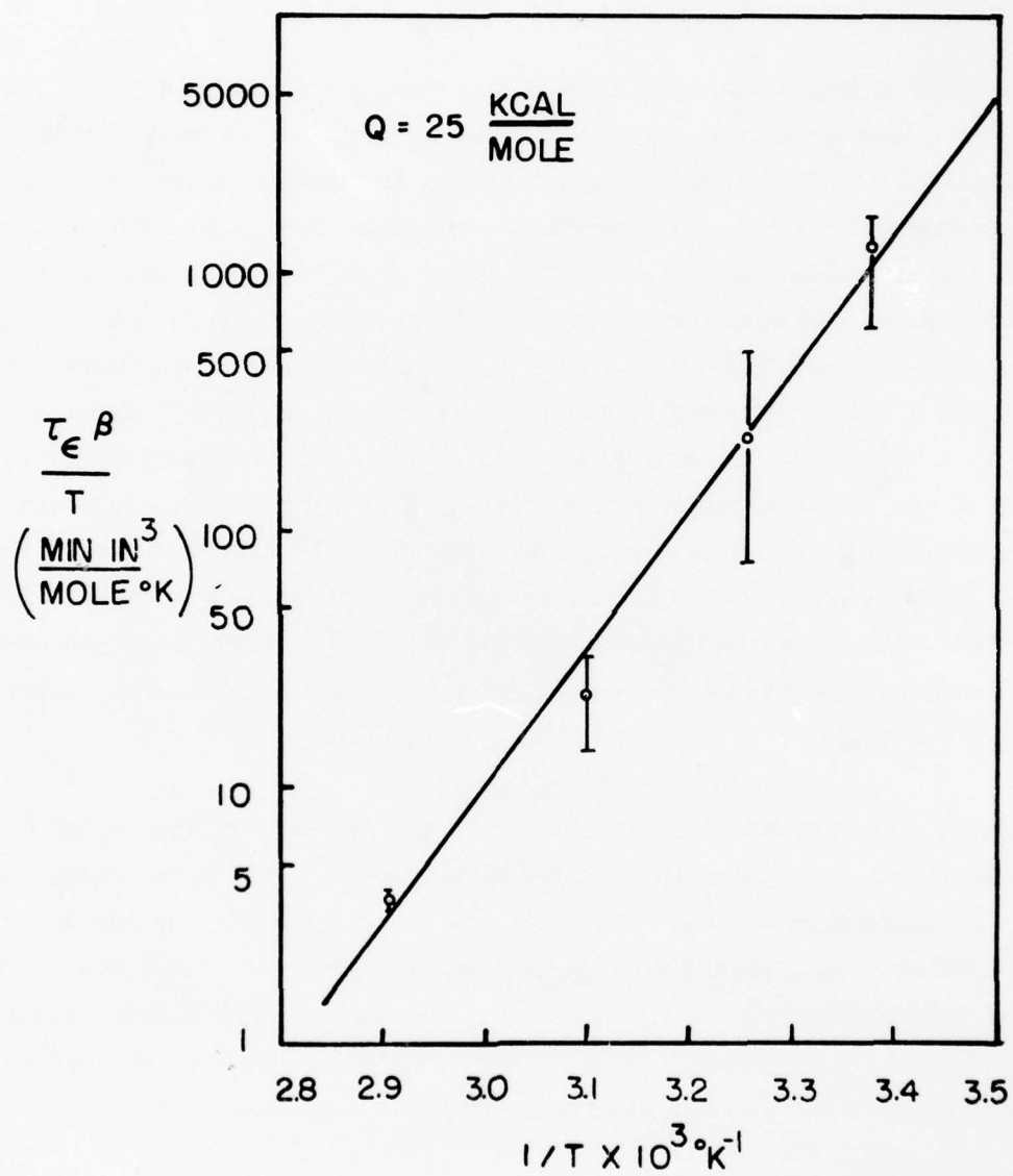
Figure 10. \text{Log } \frac{\tau \epsilon \beta}{T} Plotted versus \frac{1}{T} for PZT. The experimental activation energy is \approx 25 \text{ kcal/mole} .
