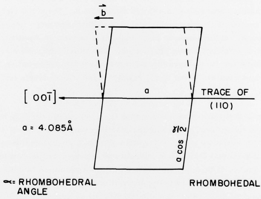
Figure 11. Schematic Showing the Geometry of Twinning in PZT
