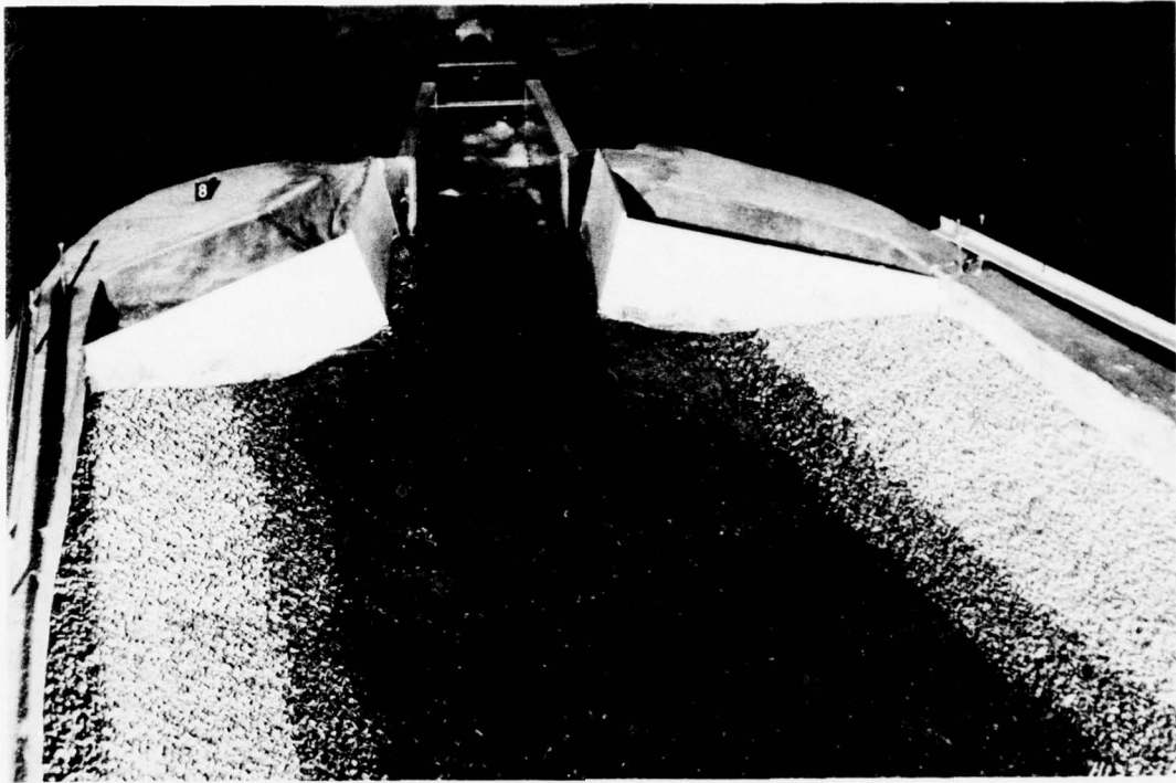
Photo 9. Flow conditions in exit channel, recommended design; pool el 675, tailwater el 577, discharge 2,000 cfs
