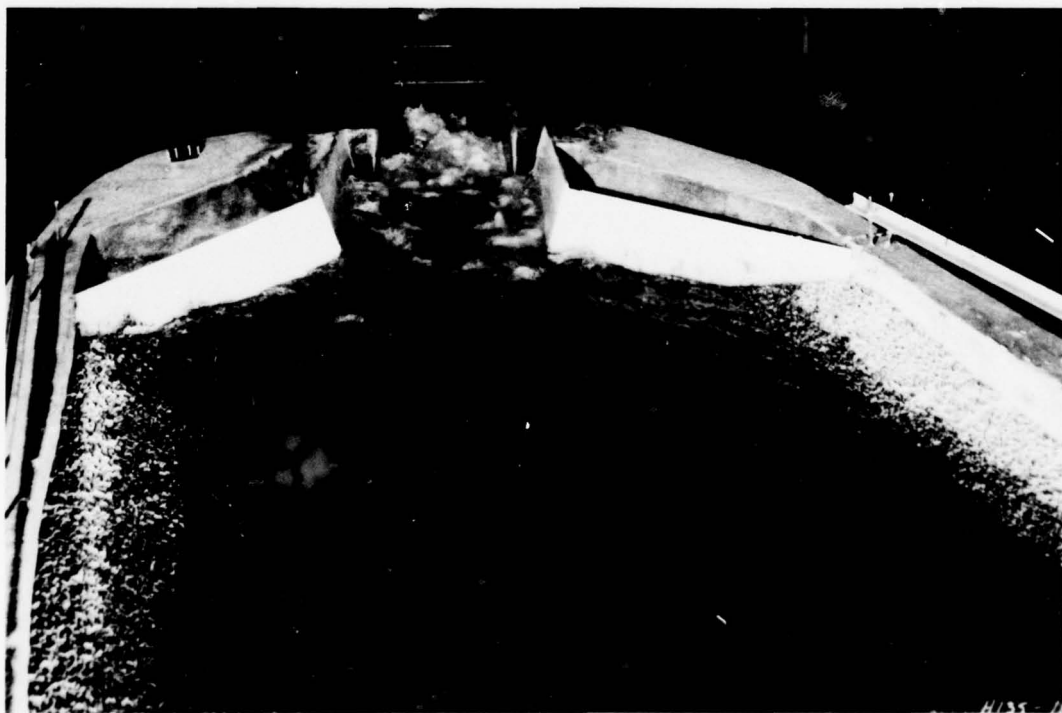
Photo 12. Flow conditions in exit channel, recommended design; pool el 709, tailwater el 584, discharge 9,400 cfs
