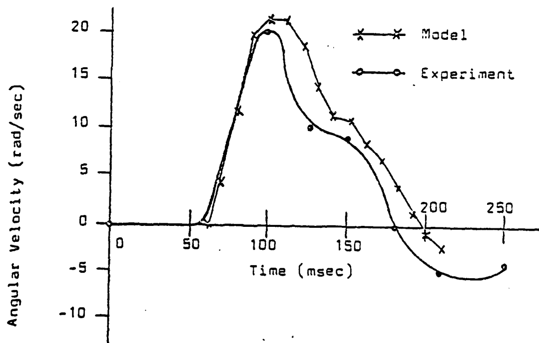
Figure 12. Comparison of Model and Ewing Experiment for Head Angular Velocity
