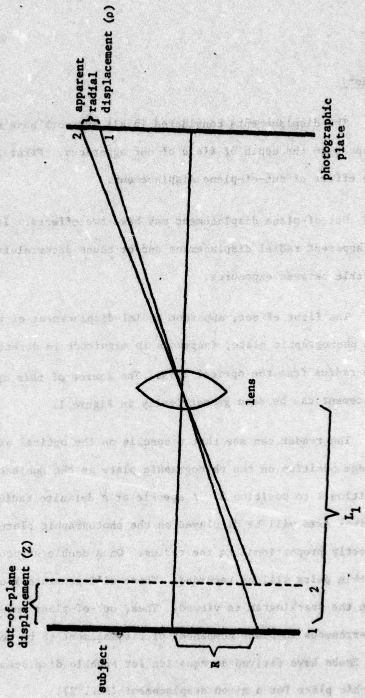
FIGURE 1 Source of radial displacement
