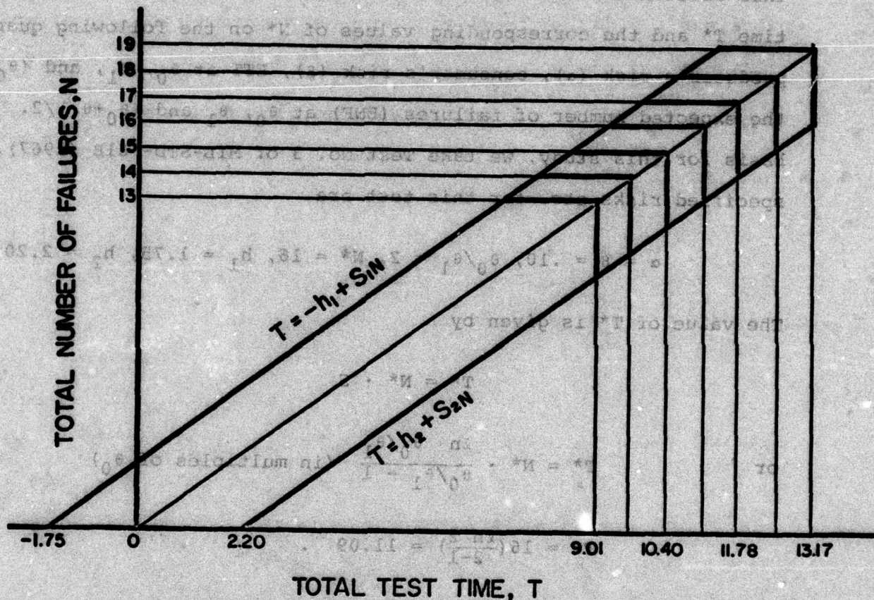
FIG. 2 DECISION BOUNDARIES WITH A VARYING TRUNCATION POINT (S_1 = S_2 = 0.693, h_1 = 1.75, h_2 = 2.20)
