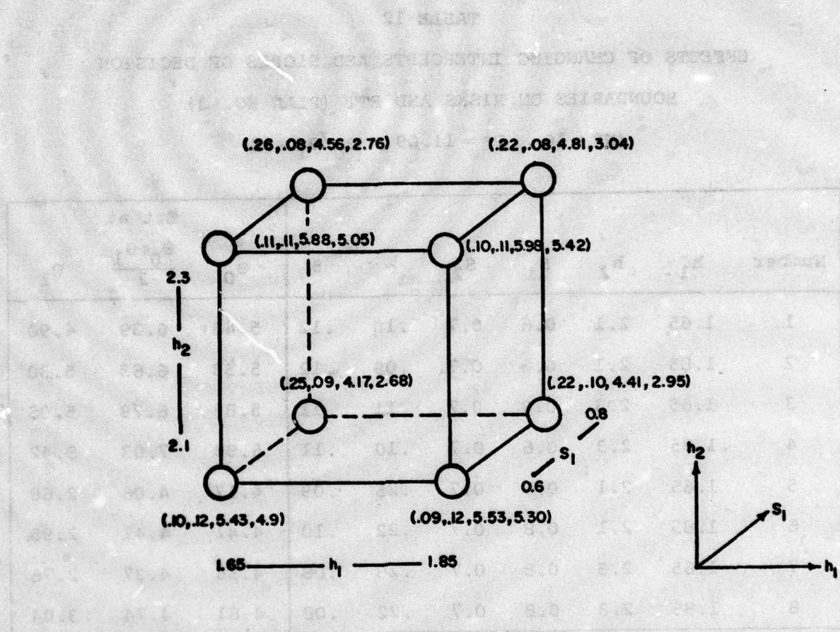
FIG. 7 VALUES OF (\alpha, \beta, \text{ETT at } \theta_0, \text{ETT at } \theta_1) FOR VARIOUS COMBINATIONS OF h_1, h_2 AND S_1 ( S_2 = 0.7 )
