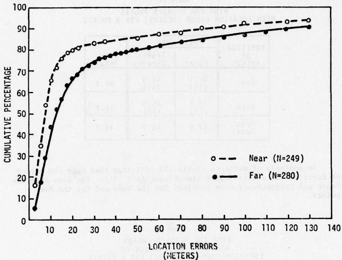
Figure 13. Cumulative percentage of location errors: high pan mission photos/A points; Position.
