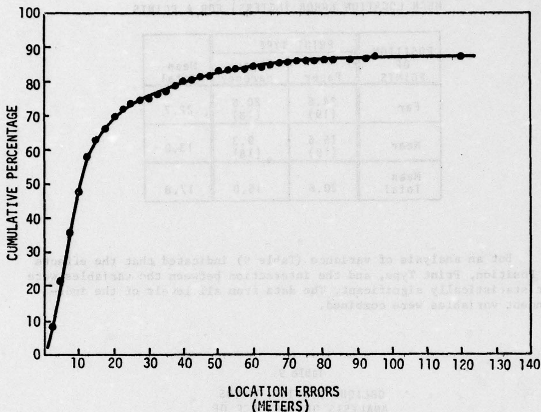
Figure 10. Cumulative percentage of location errors: oblique mission photos/A points (N=529).
