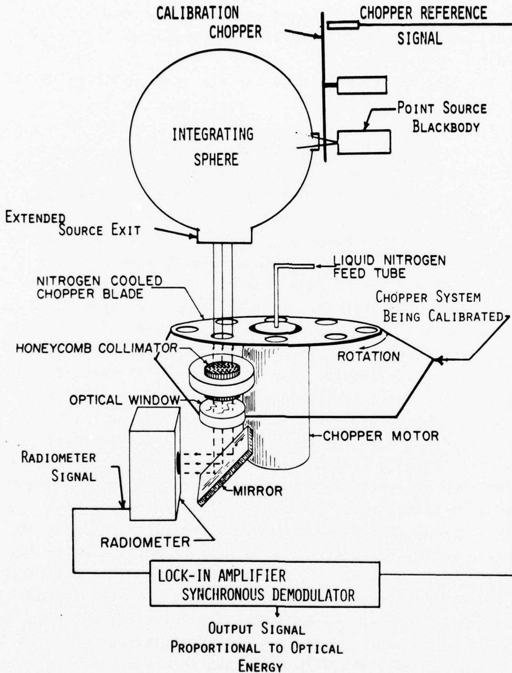
Figure 12. Calibration set up for the liquid nitrogen cooled chopper-collimator.
