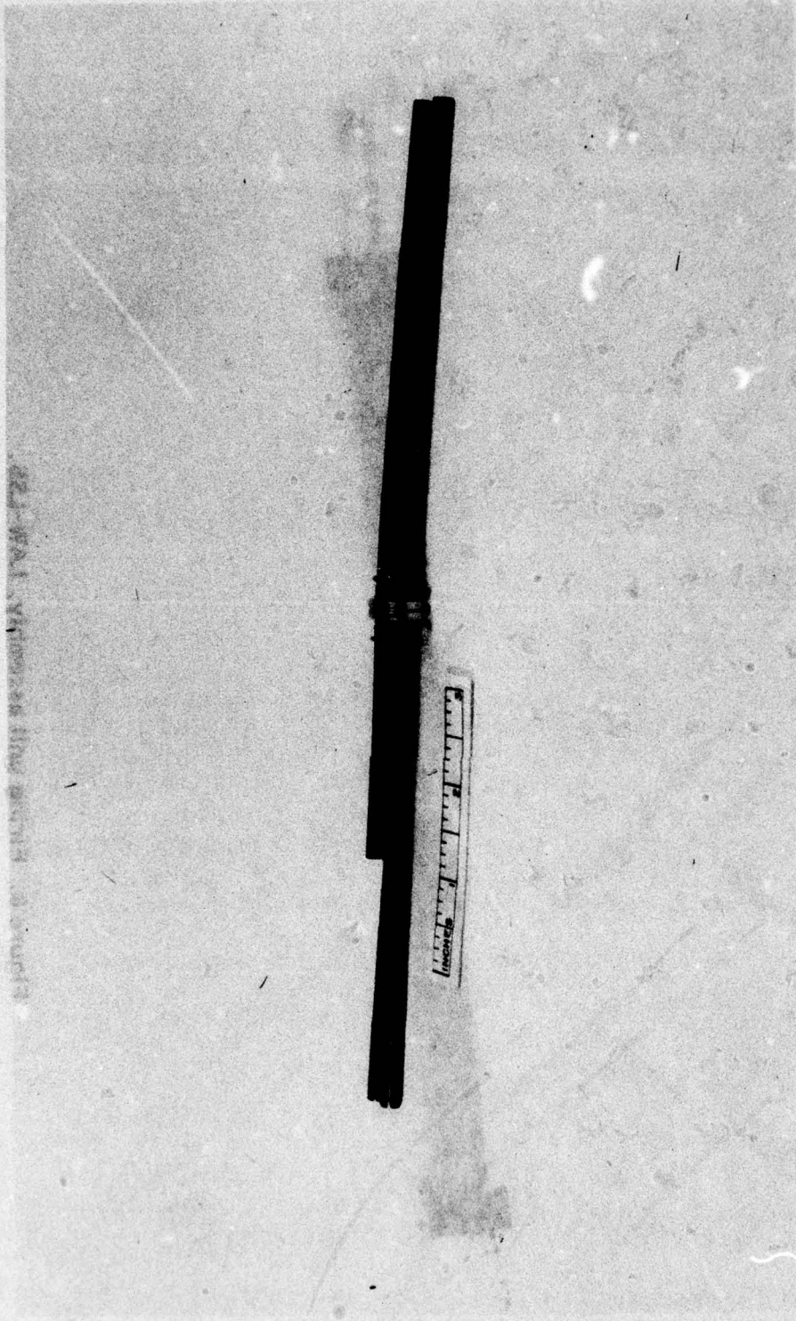
Figure 7. Propellant charge assembly, LAW-LSS.
