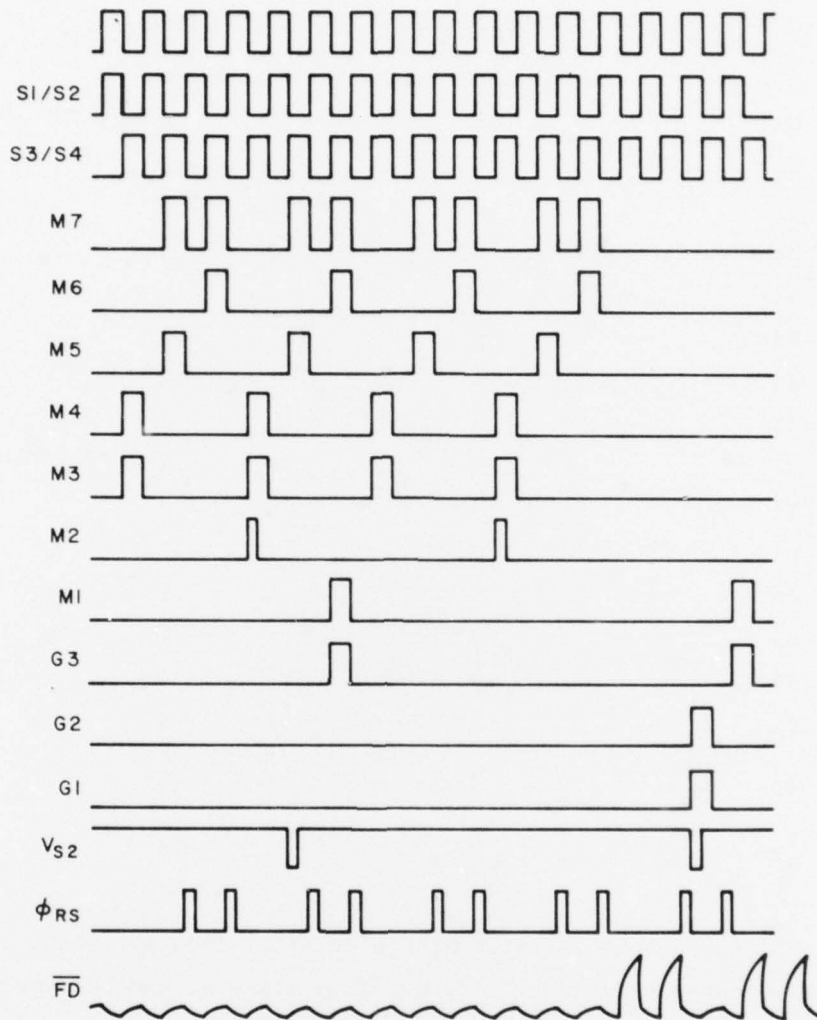
Figure 34. Timing diagram for the 4:1 multiplexer test chip.
