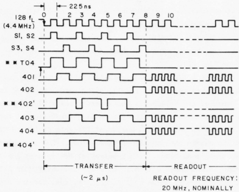
Figure 25. Timing diagram for the transfer and readout clocks of the output register.
