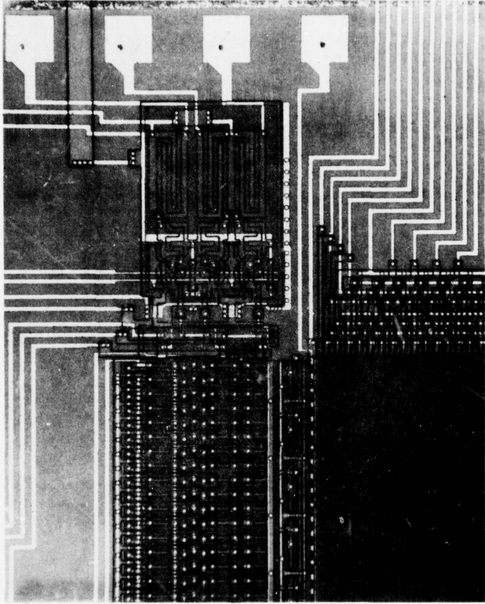
Figure 14. The right-hand part of the double 2:1 multiplexed output registers (shown in Section E, Fig. 9(e)).
