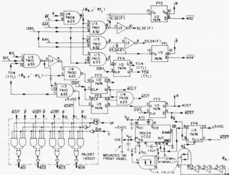
Figure 26. Circuit schematic for the output register clock generation.
