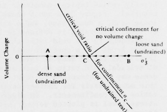
(e) Volume change - confining stress.
