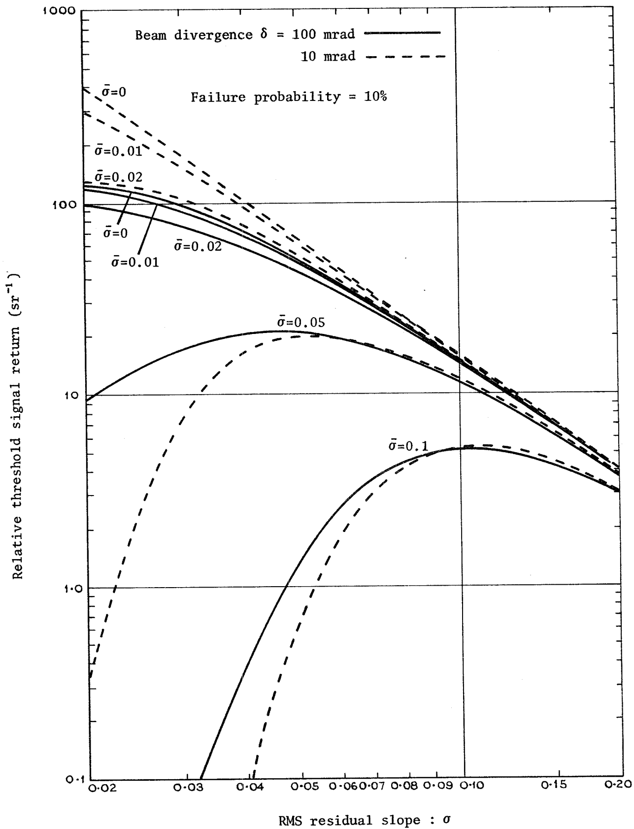
Figure 11. Dependence of the relative threshold signal return on the rms residual slope for a failure probability of 10%
