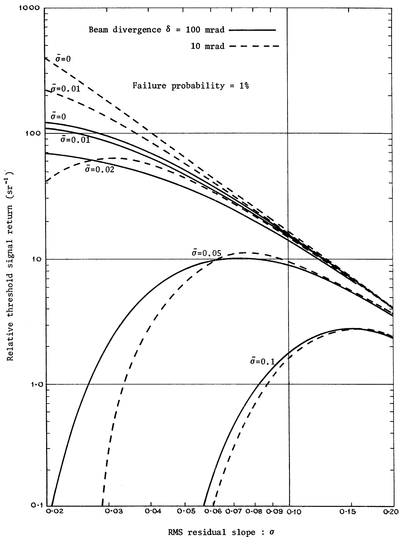
Figure 10. Dependence of the relative threshold signal return on the rms residual slope for a failure probability of 1%
