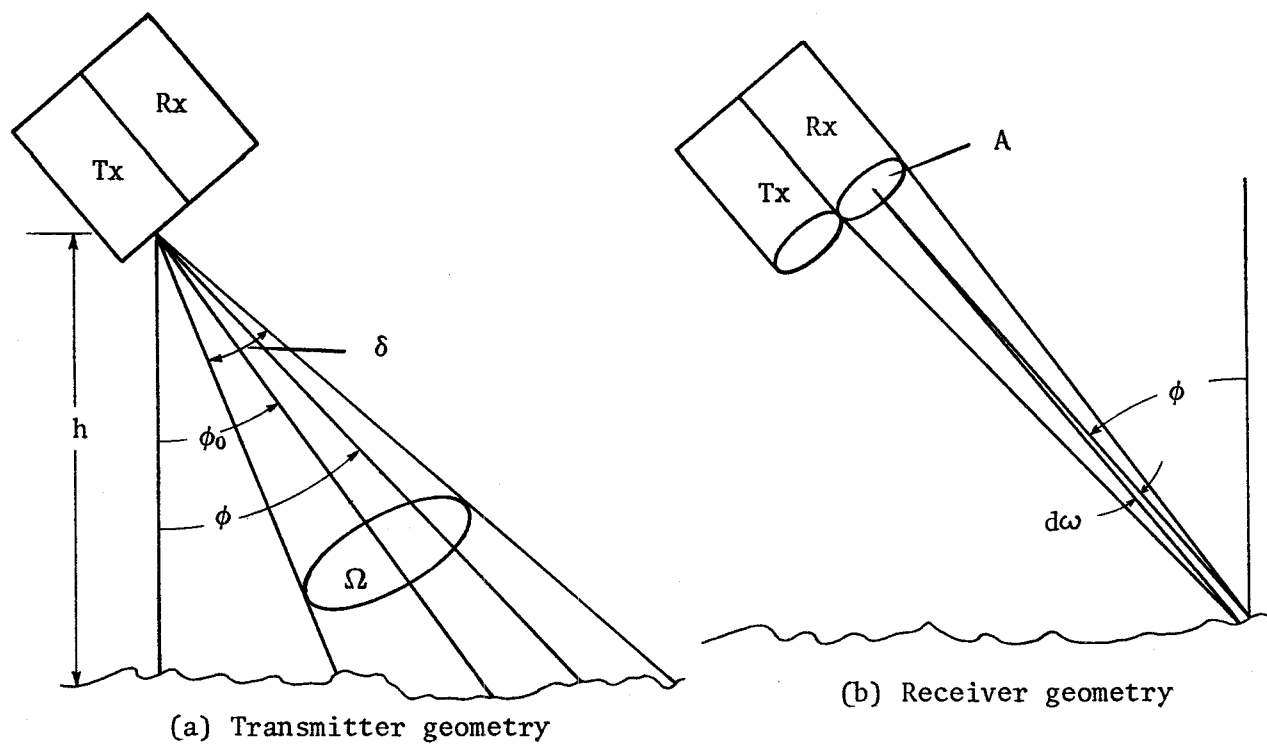
Figure 6. Schematic diagram of laser beam reflection from the sea surface
