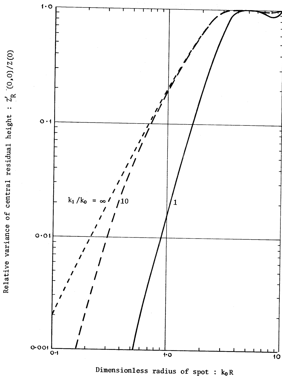
Figure 3. Dependence of the relative variance of the central residual height on the dimensionless radius of the spot
