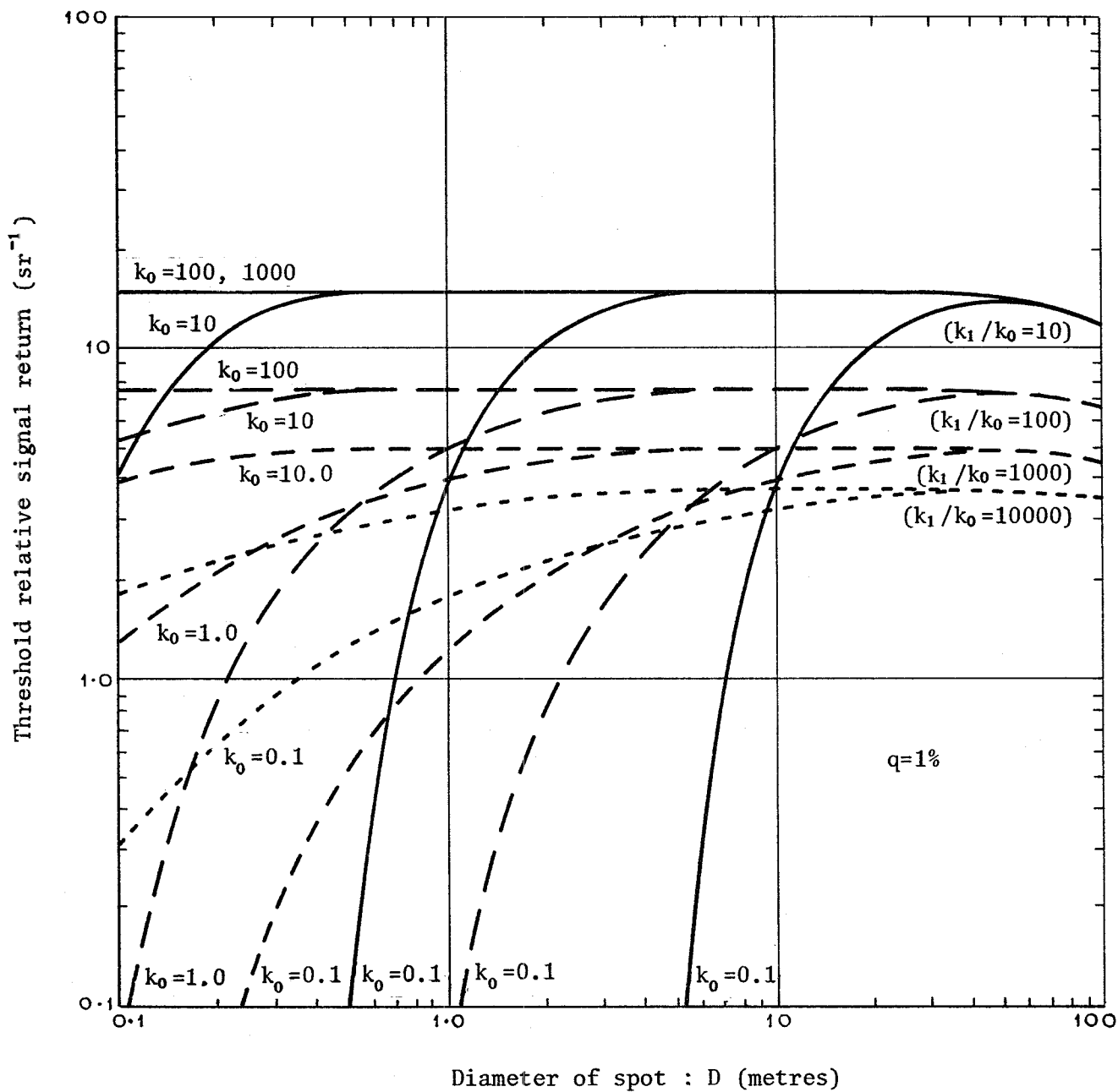
Figure 13. Dependence of the relative threshold signal return on the spot diameter for a failure probability of 1% and a variety of sea states
