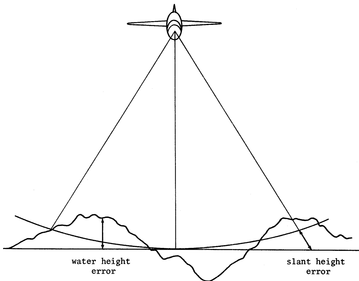
Figure 16. Variation of water height and slant height errors over illuminated spot
