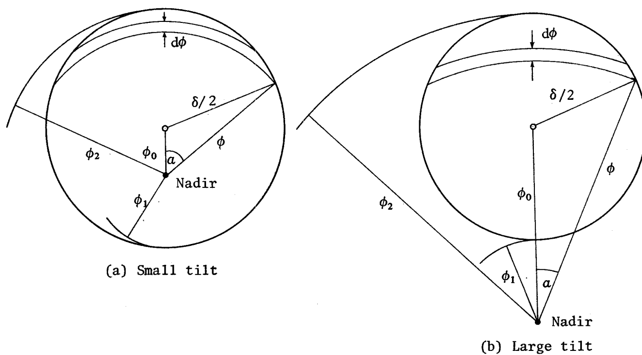
Figure 7. Geometry of tilted laser beam and receiver field of view
