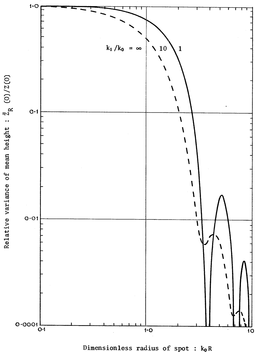
Figure 1. Dependence of the relative variance of the mean height on the dimensionless radius of the spot
