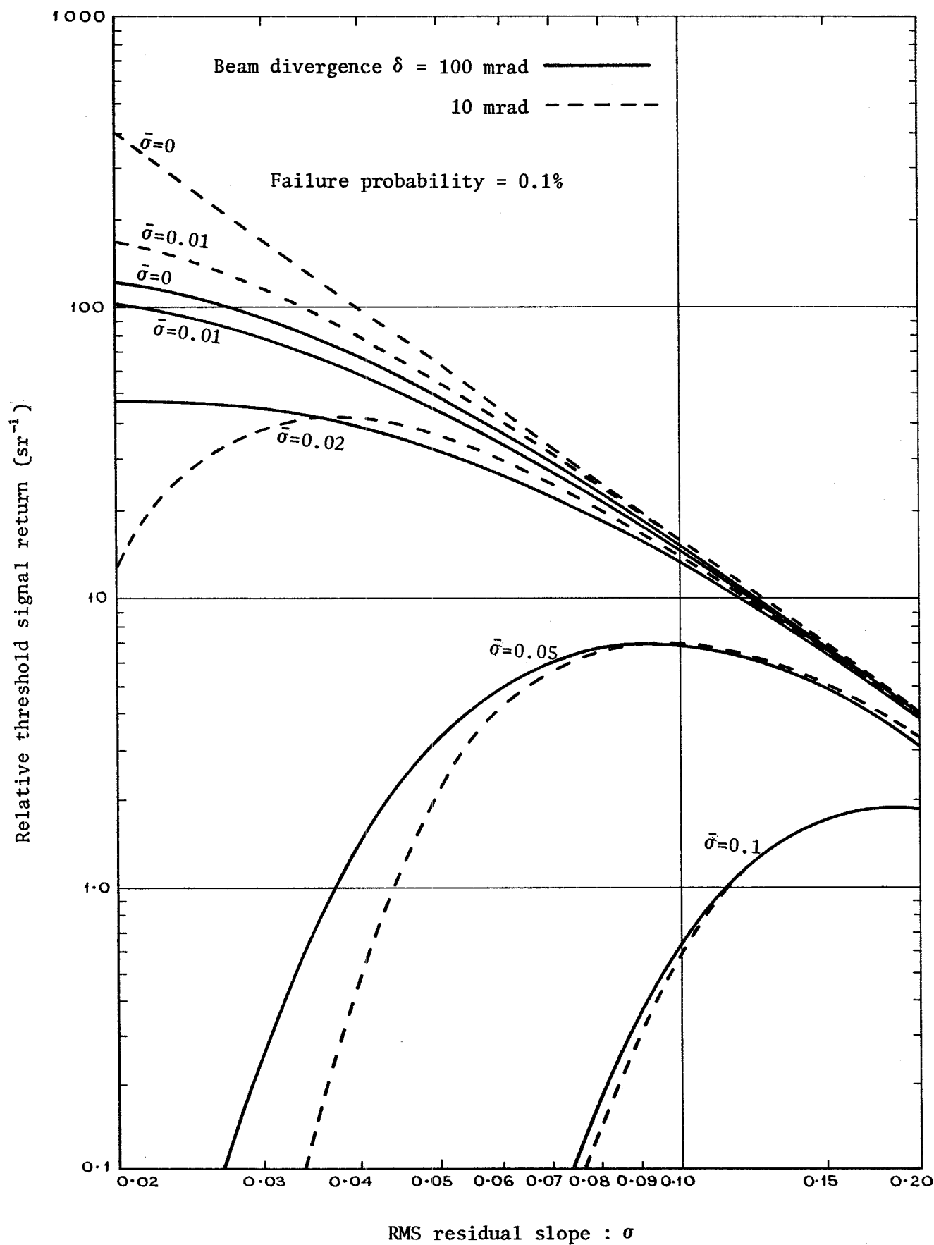
Figure 9. Dependence of the relative threshold signal return on the rms residual slope for a failure probability of 0.1%
