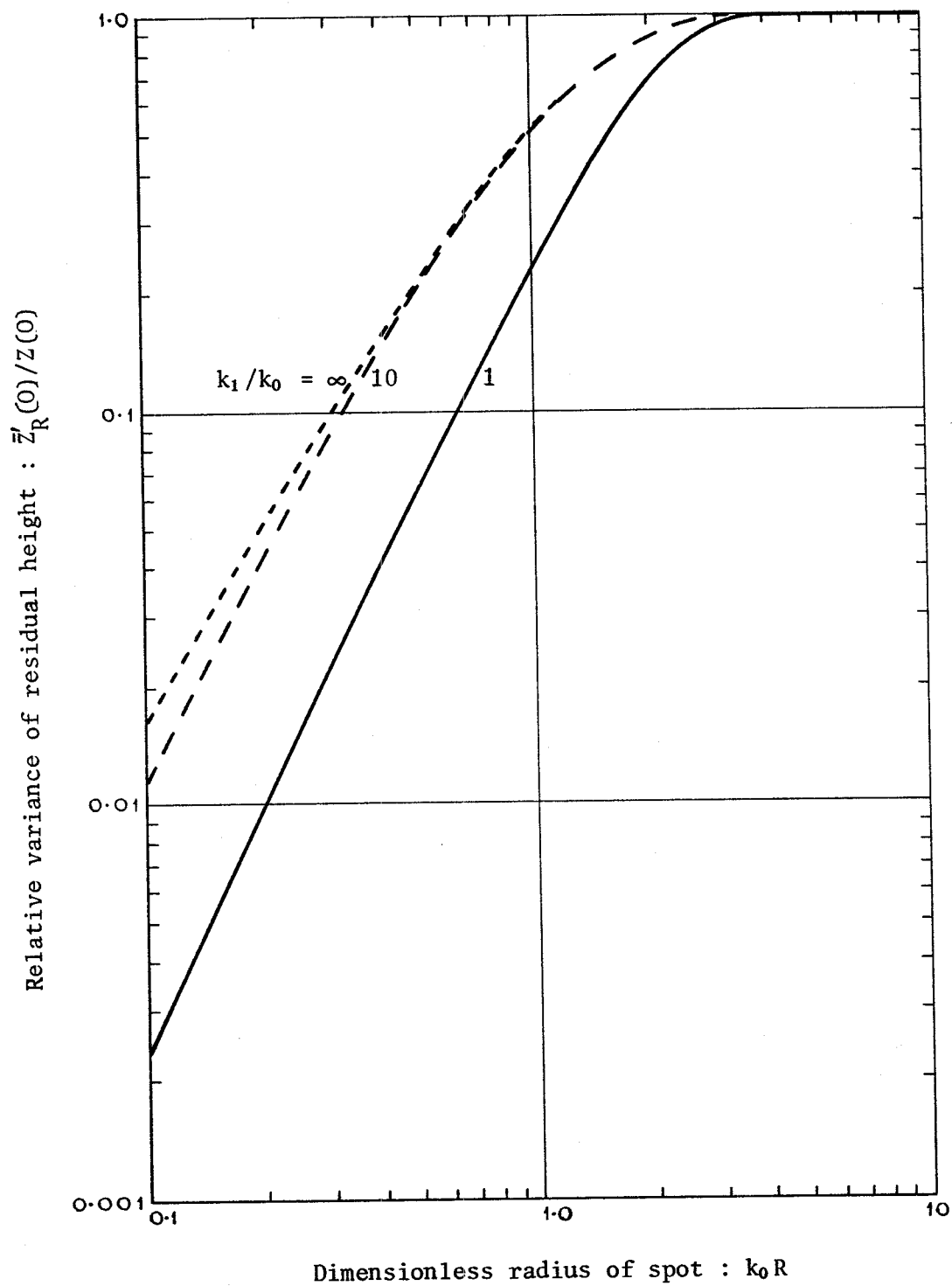
Figure 2. Dependence of the relative variance of the residual height on the dimensionless radius of the spot
