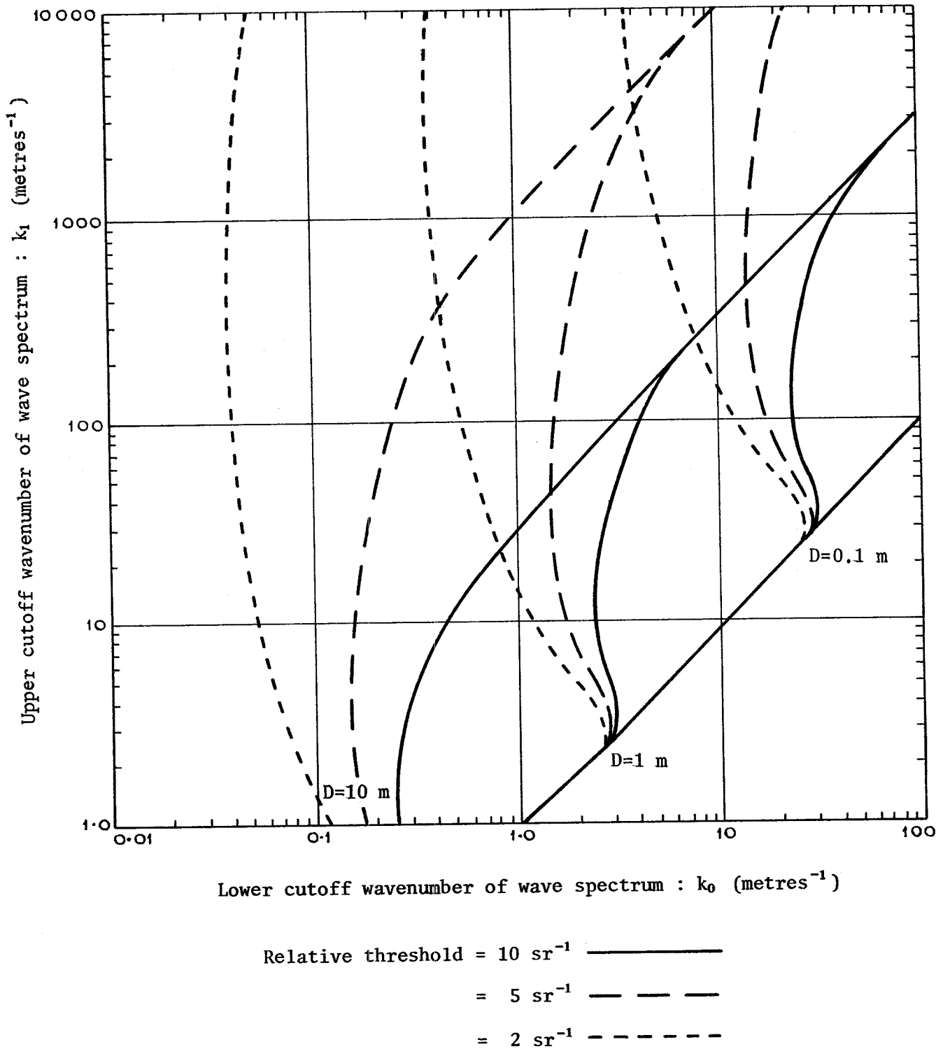
Figure 15. Range of sea states for which given spot diameters and relative thresholds achieve a failure probability below 0.1%
