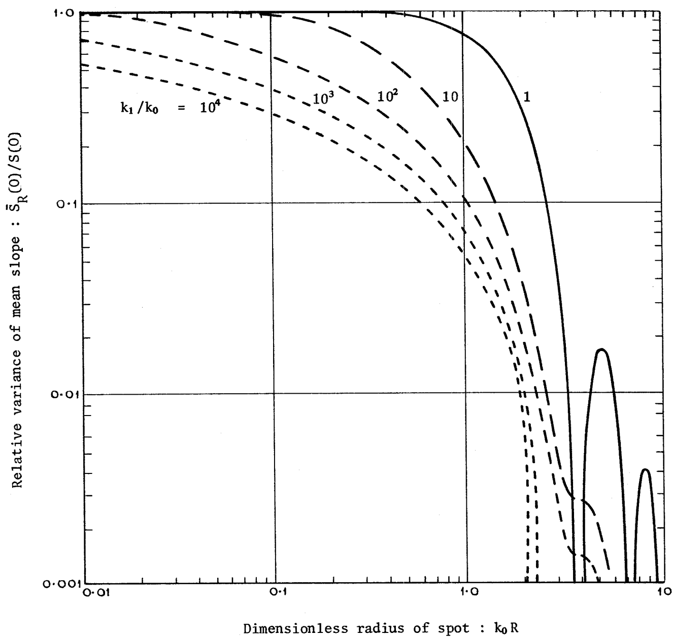
Figure 4. Dependence of the relative variance of the mean slope on the dimensionless radius of the spot
