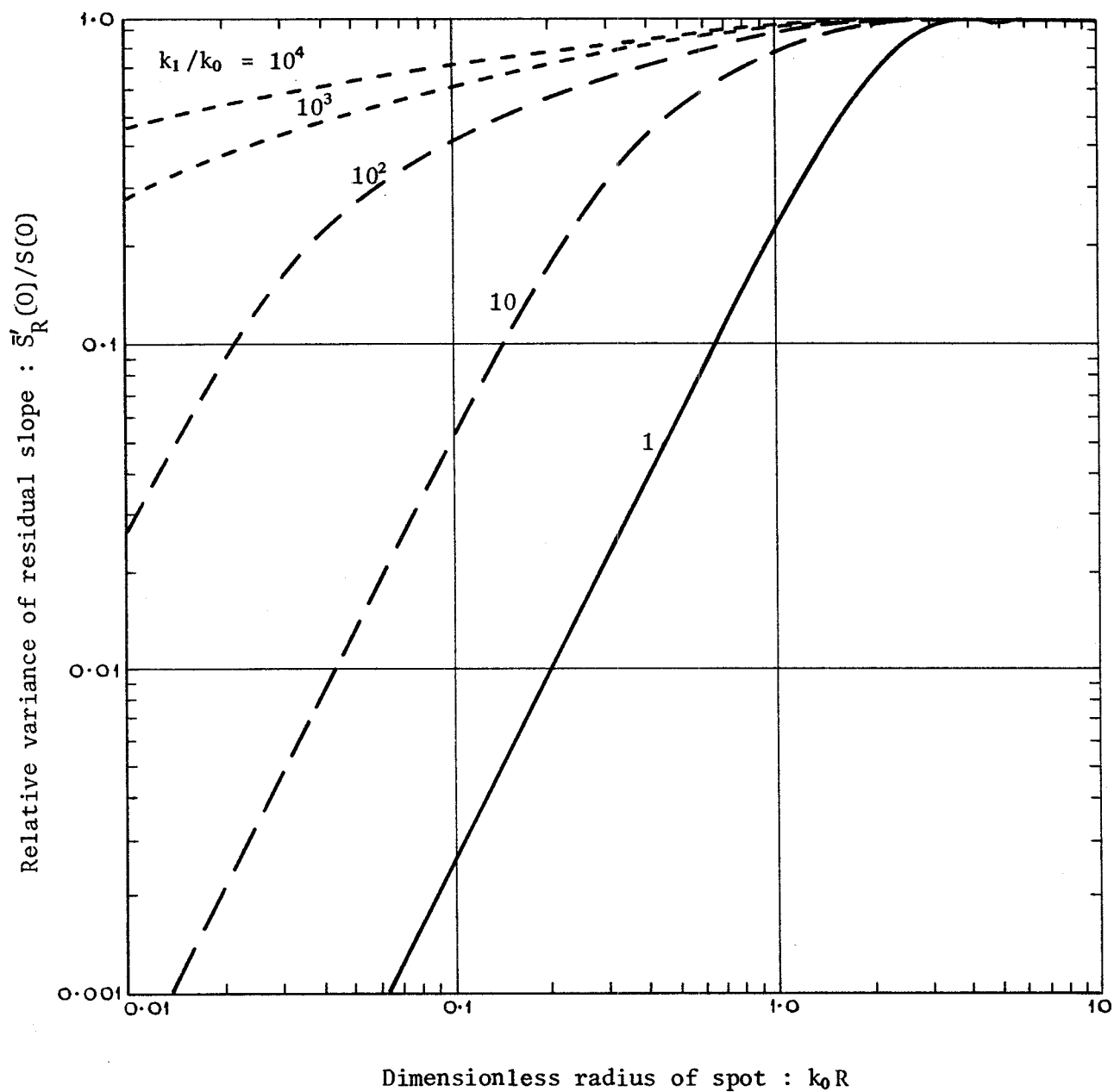
Figure 5. Dependence of the relative variance of the residual slope on the dimensionless radius of the spot
