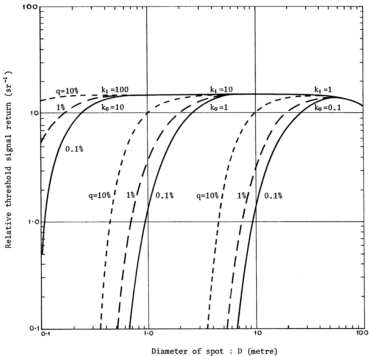
Figure 12. Dependence of the relative threshold signal return on the spot diameter for three failure probabilities
