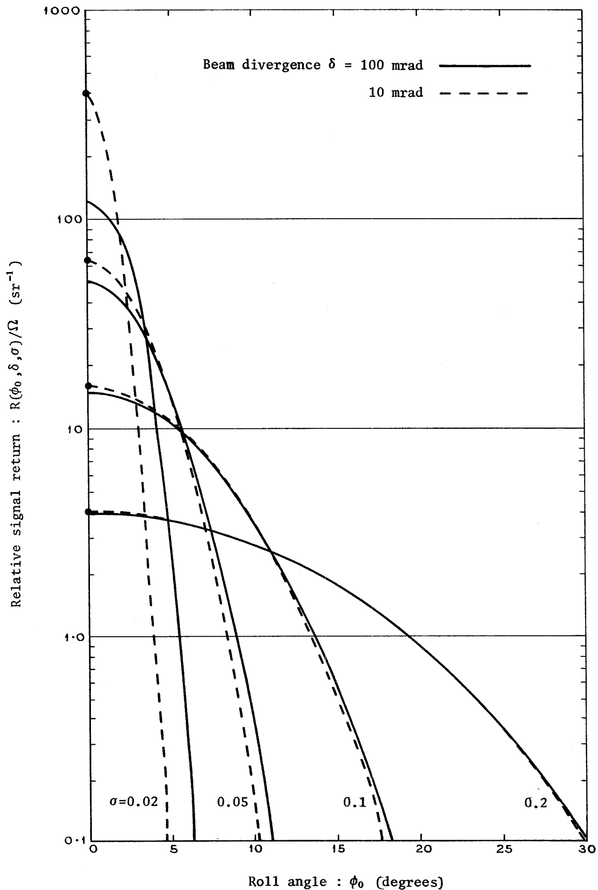
Figure 8. Dependence of the relative signal return on roll angle and beam divergence
