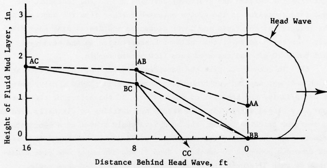
Figure 23. Fluid mud layer profiles, test 37
