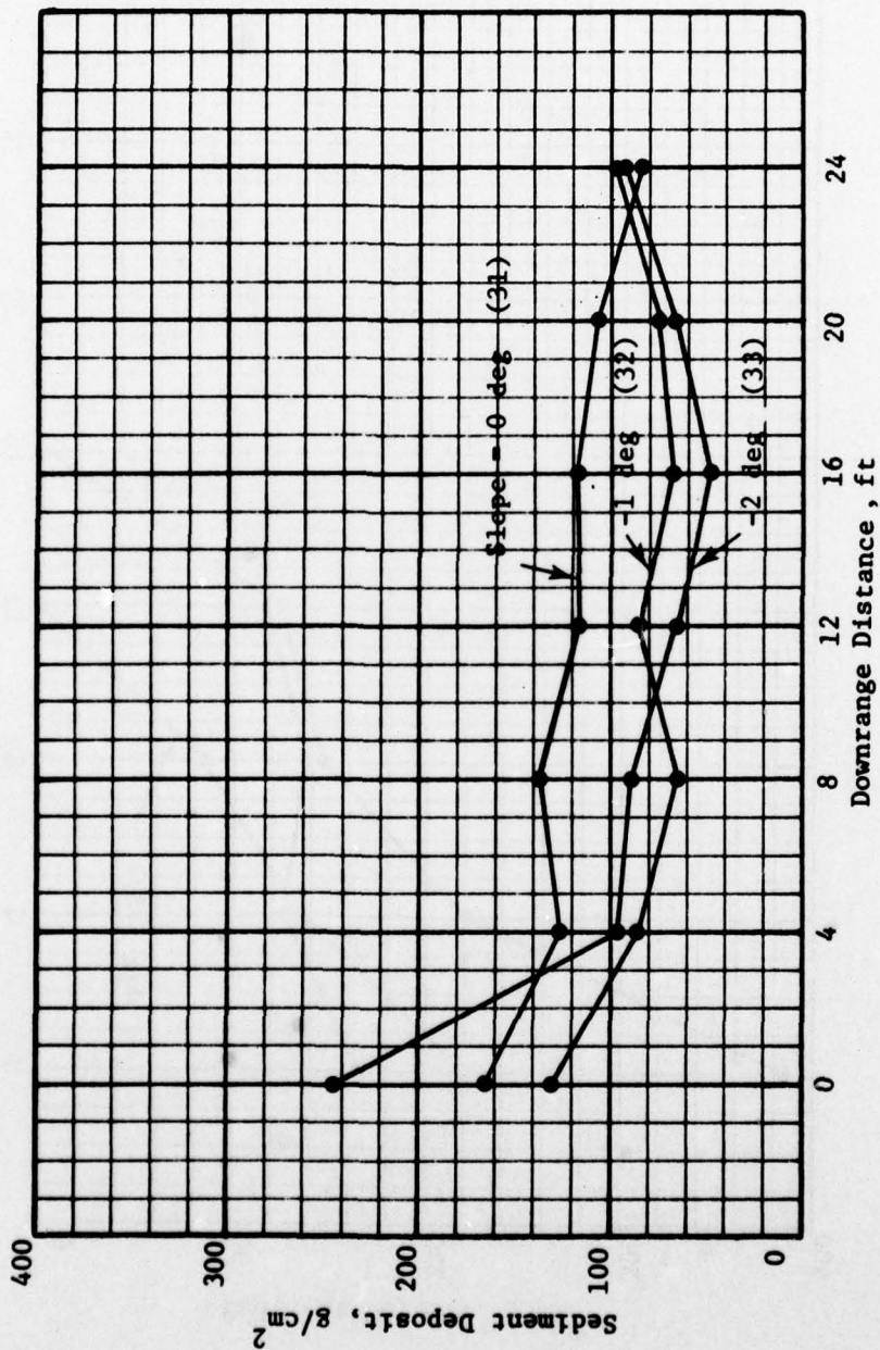
Figure B5. Sediment deposit profiles for negative slopes, 10-pcs slurry
