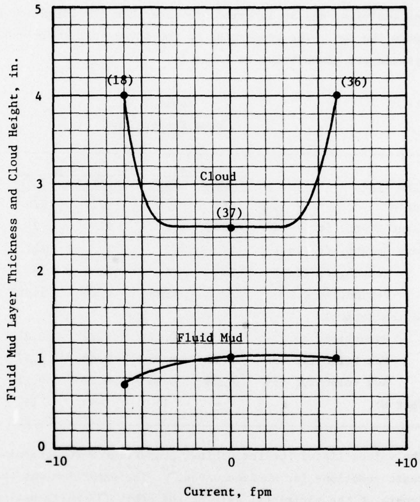
Figure 44. Cloud height and fluid mud layer thickness versus current
