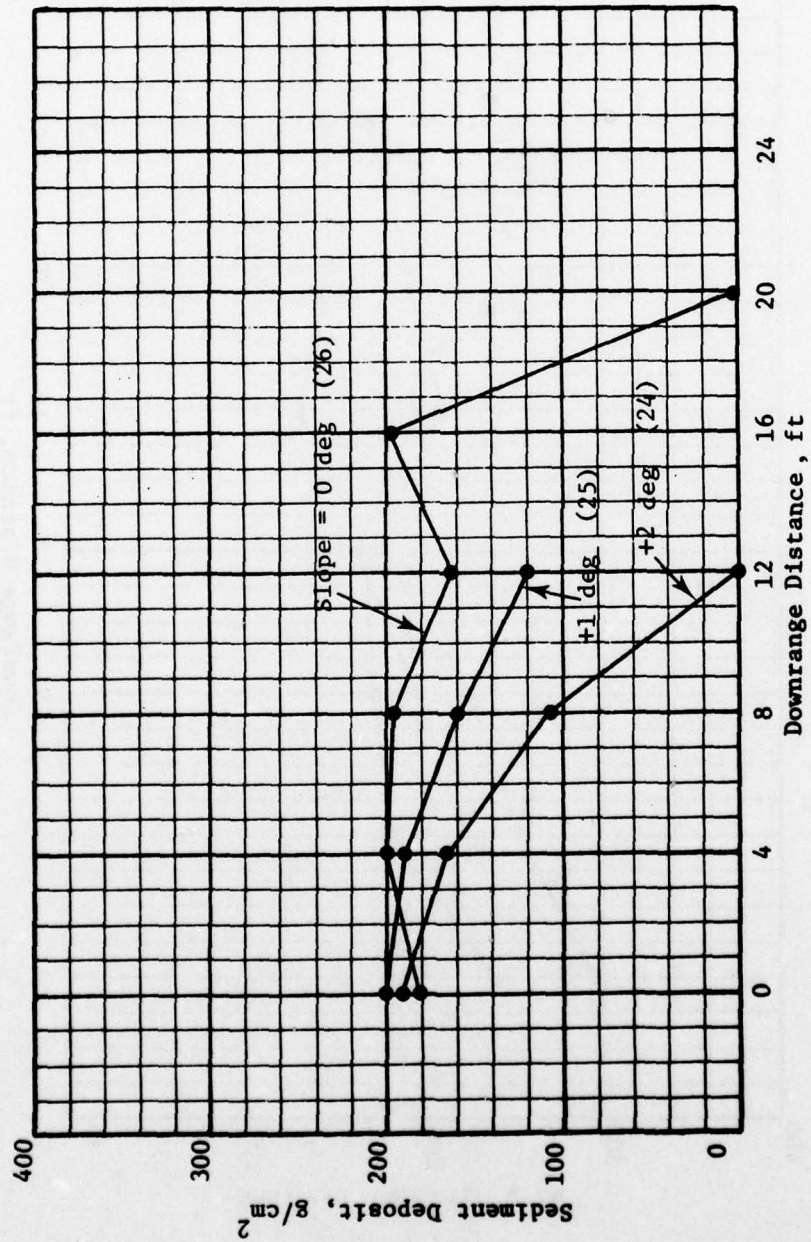
Figure B8. Sediment deposit profiles for positive slopes, 20-pcs slurry
