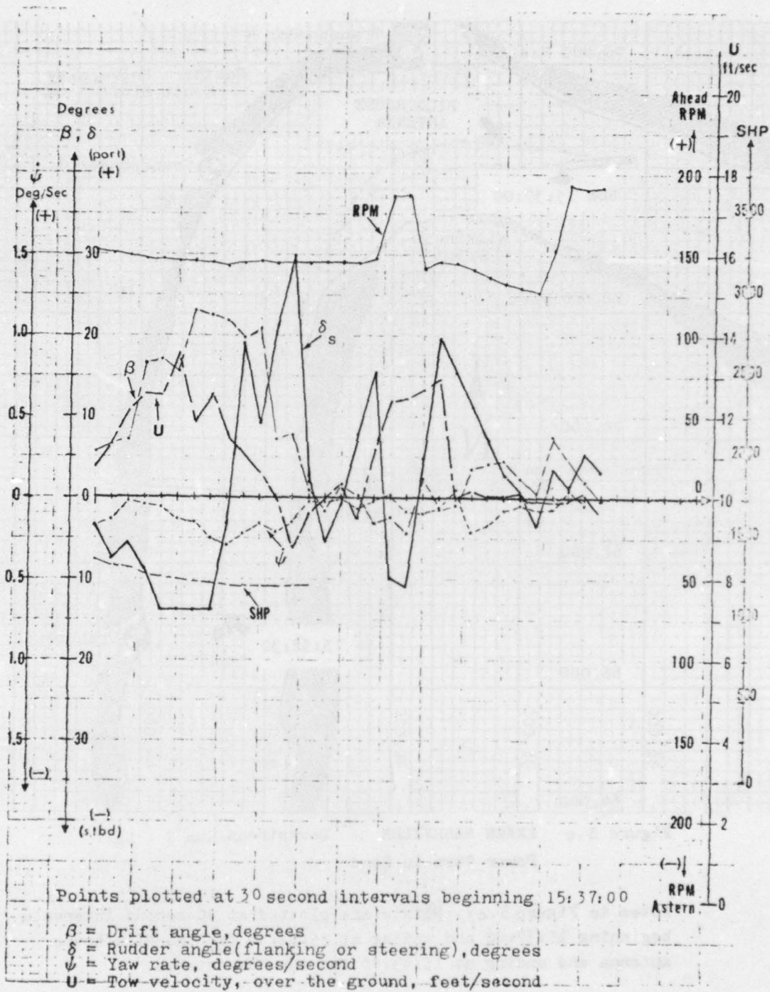
Figure 5.d EXXON NASHVILLE - Downstream Run 2 - Half Power Turn in Bend
