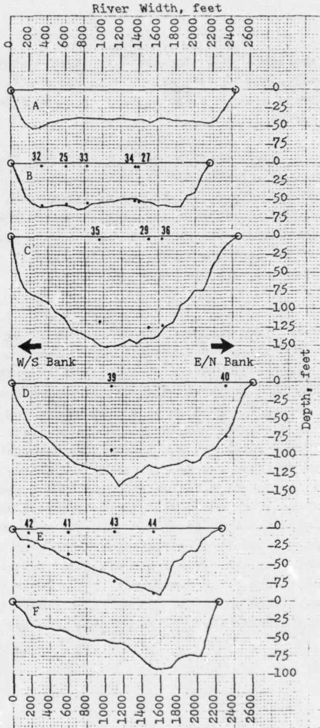
Figure 3.1 River Cross-Sections
