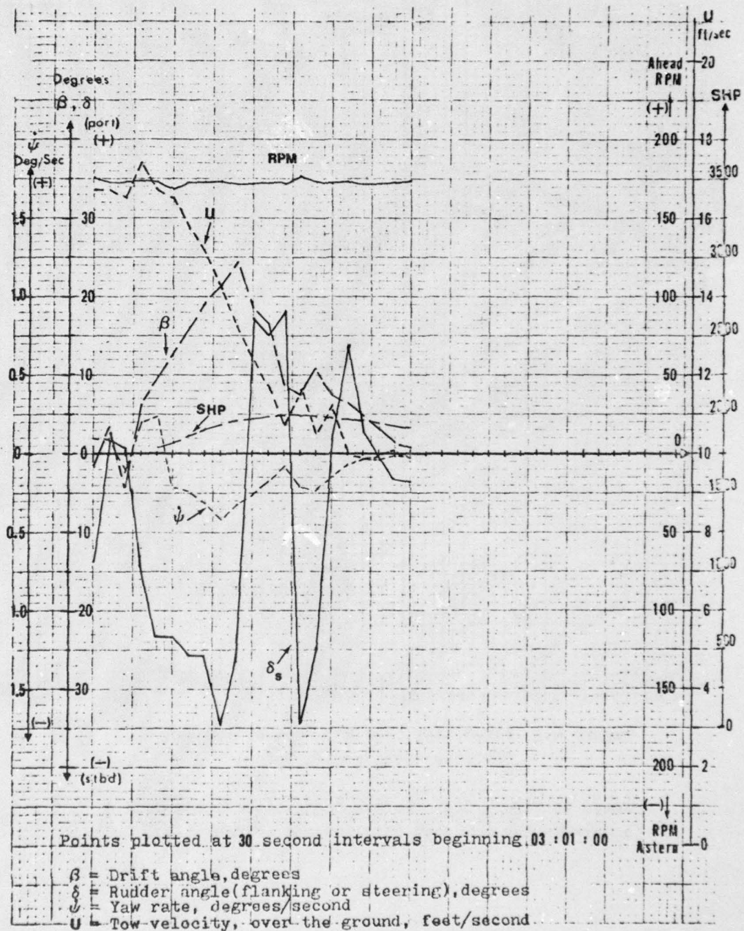
Figure 6.h EXXON LAKE CHARLES - Downstream Run 4 - 3/4 Power Turn Around Bend
