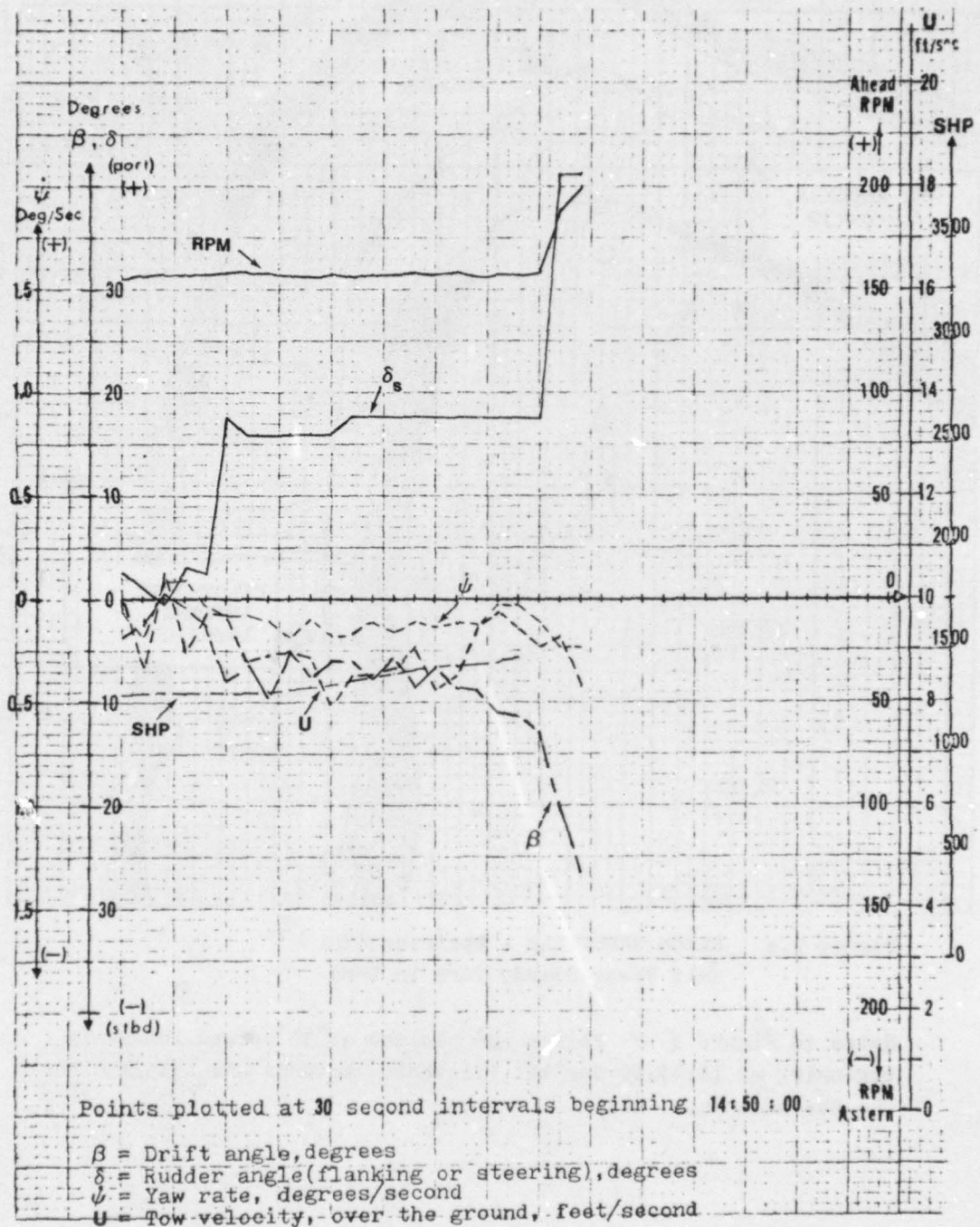
Figure 5.b EXXON NASHVILLE - Upstream Run 1 - Half Power Turn in Bend
