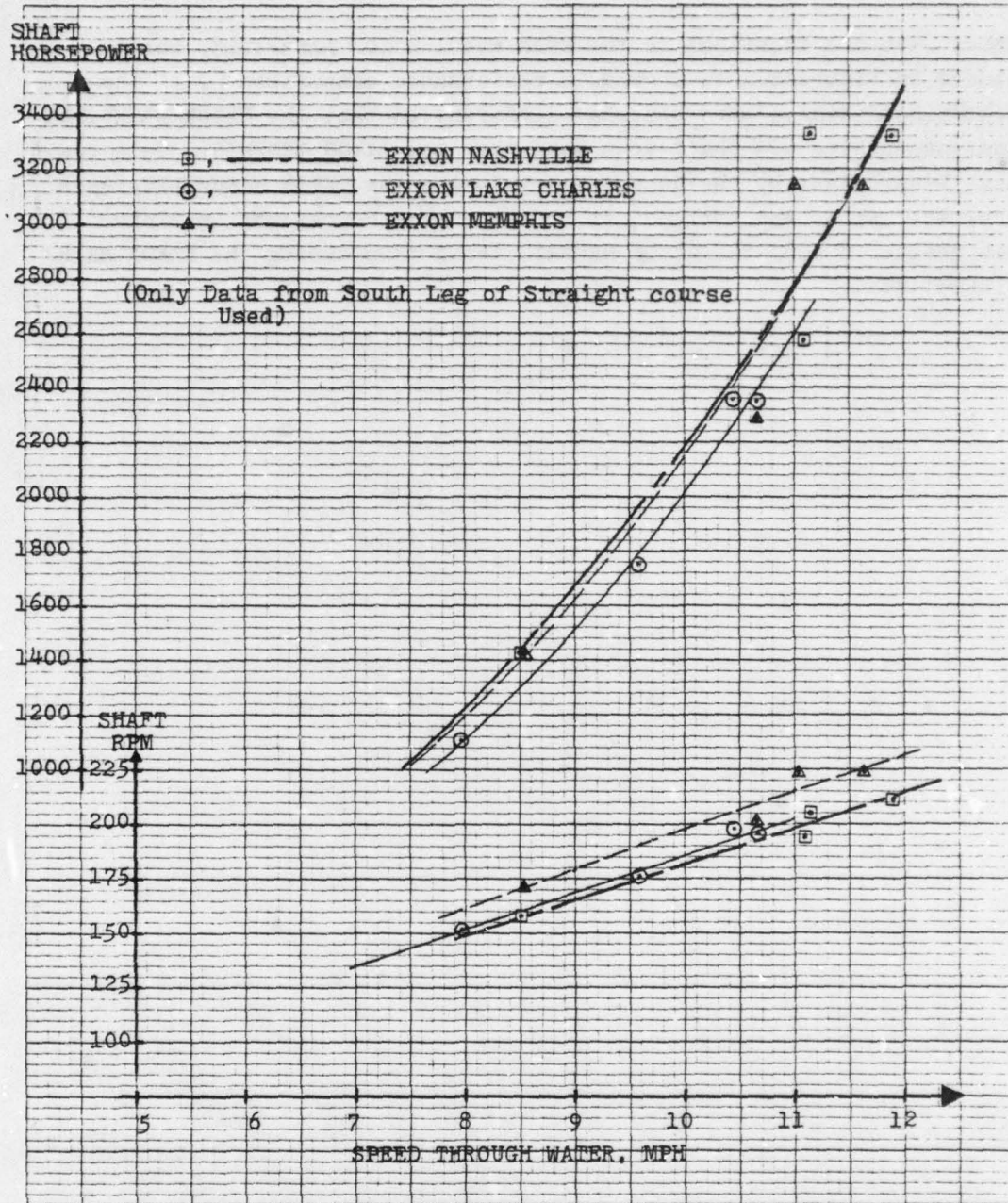
Figure 8.a Speed-Power Curves
