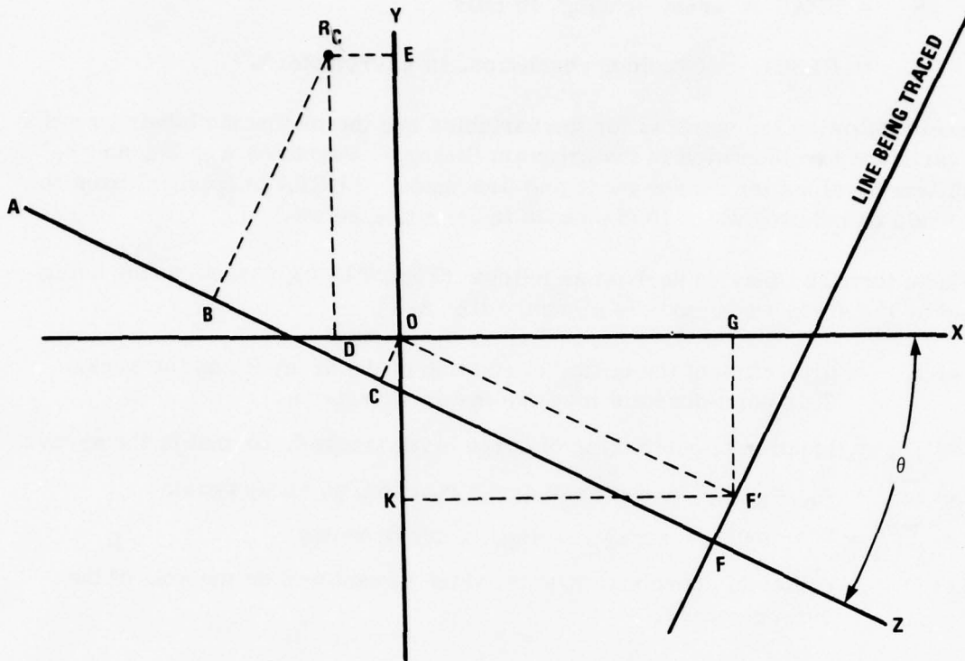
Figure 13. Geometry of computer correction algorithm.
