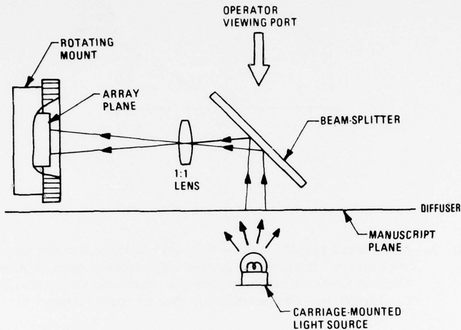
Figure 2. Configuration of a backlighting scanning array cursor.
