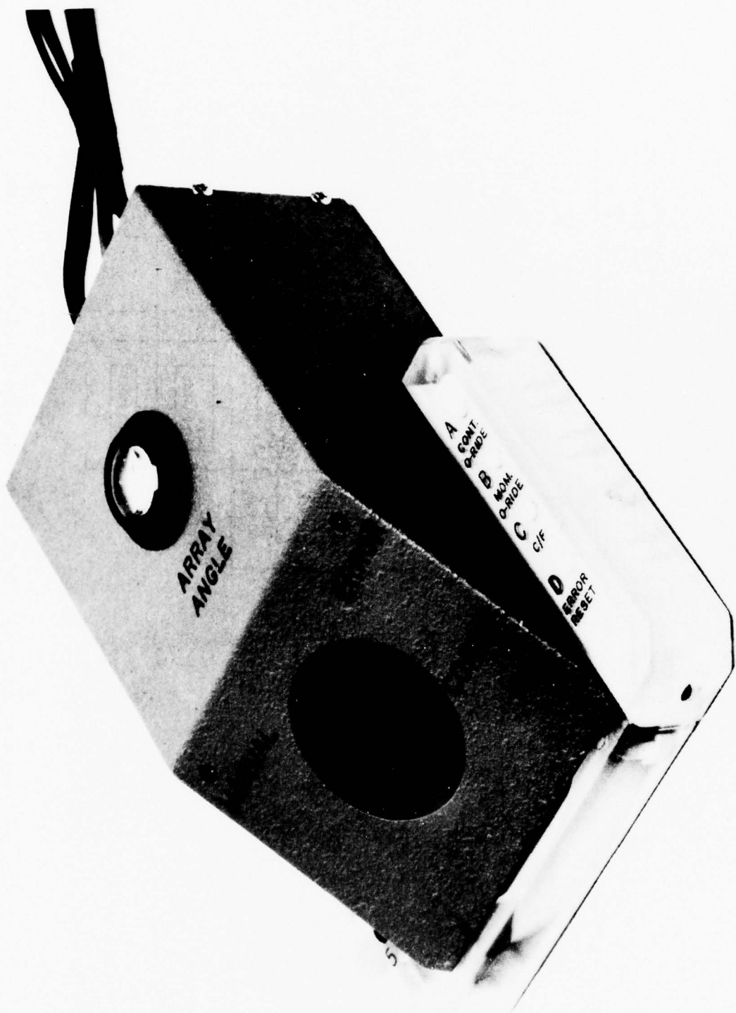
Figure 7. Photograph of aided-track scanning cursor. Scale approximately 1.25-to-1.
