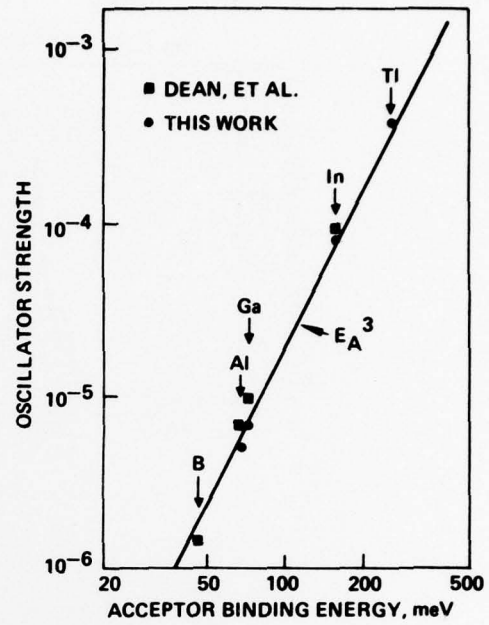
Figure 5. The total absolute oscillator strength for the lowest known transitions of an electron-hole pair bound to an acceptor. The data indicated by \blacksquare were taken from P.J. Dean, W.F. Flood, and G. Kaminsky (Phys. Rev. 163 , 721 (1967))
