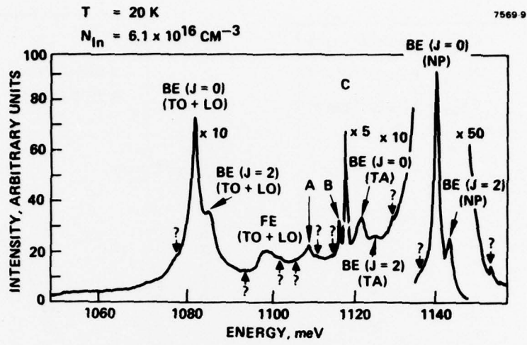
Figure 7. The luminescence from a Czochralski-grown Si:In sample. The lines labeled BE are due to an electron-hole pair bound to a neutral In. The lines labeled with A, B, C, and the lines labeled with ? are of unknown origin.
