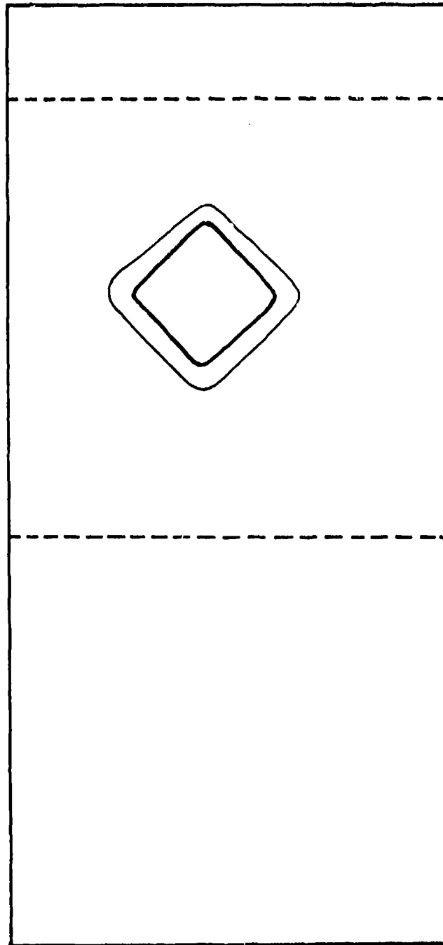
Fig. 6-19 Computer generated thermograph modeling diamond inclusion in graphite-epoxy laminate
