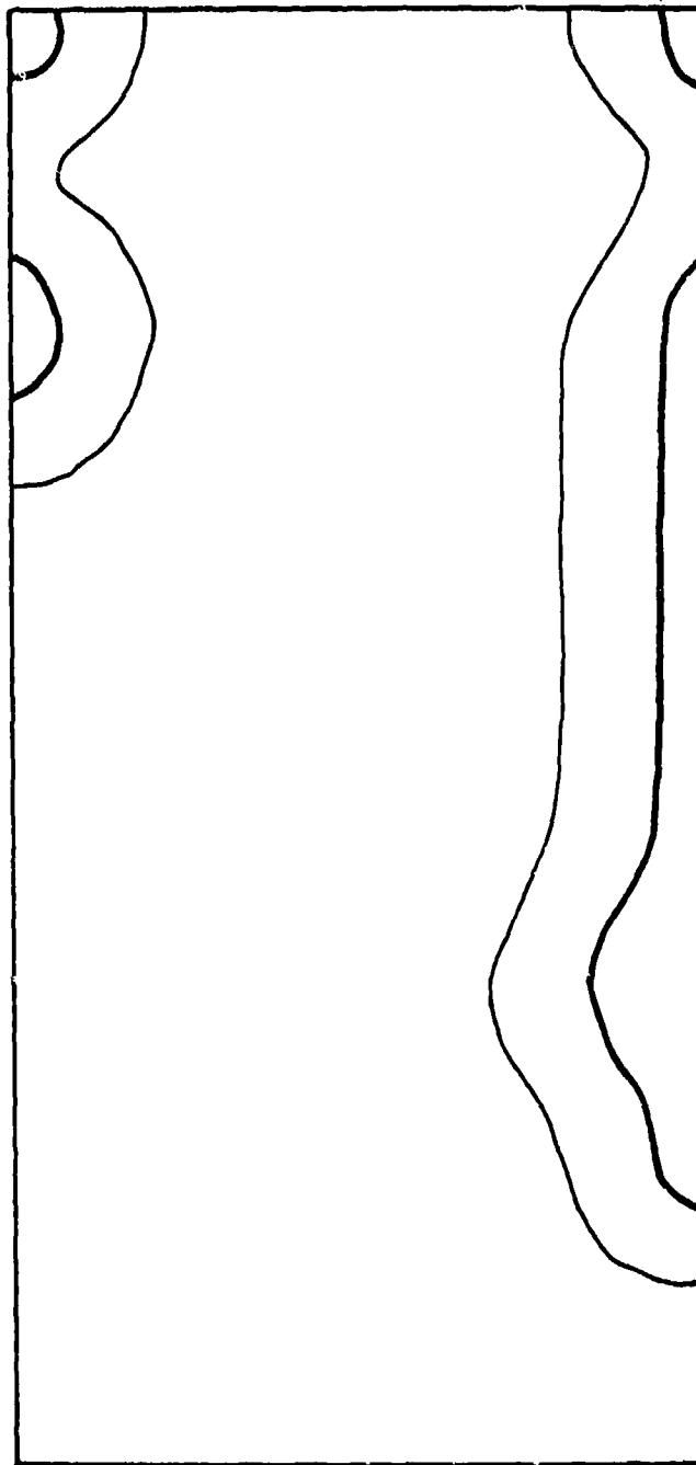
Fig. 6-9 Computer generated thermograph for type I specimen, modeling damage observed in Fig. 6-8
