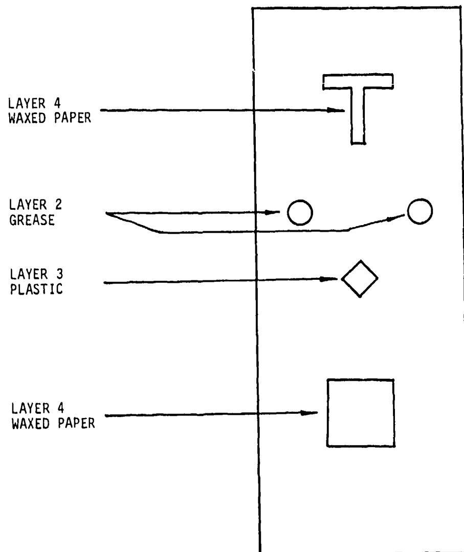
Fig. 6-12 Schematic diagram of intentionally manufactured flaws in graphite-epoxy laminate
