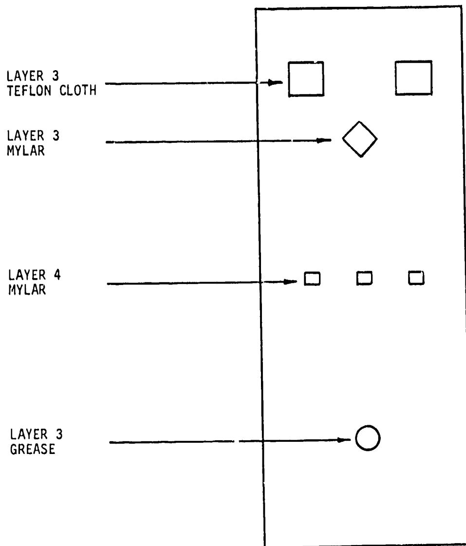
Fig. 6-20 Schematic diagram of intentionally manufactured flaws in second graphite-epoxy laminate
