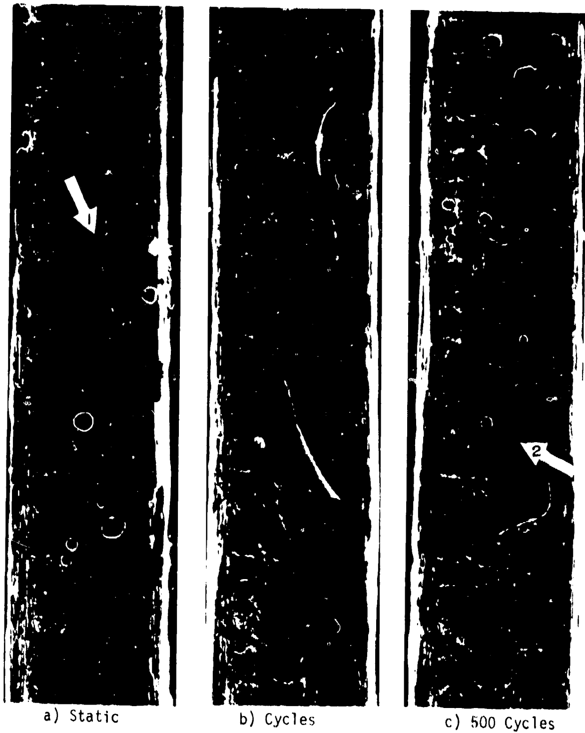
Fig. 3-11 Damage along the edge of a type II specimen at 393 MPa after a) static preload, b) 50 cycles, c) 500 cycles
