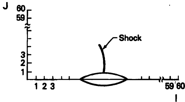
Figure 10. Supersonic-Subsonic Shocks.
