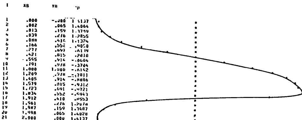
Figure 1. C_p on a Sphere at M = 1.2 (RAXBOD Solution).
