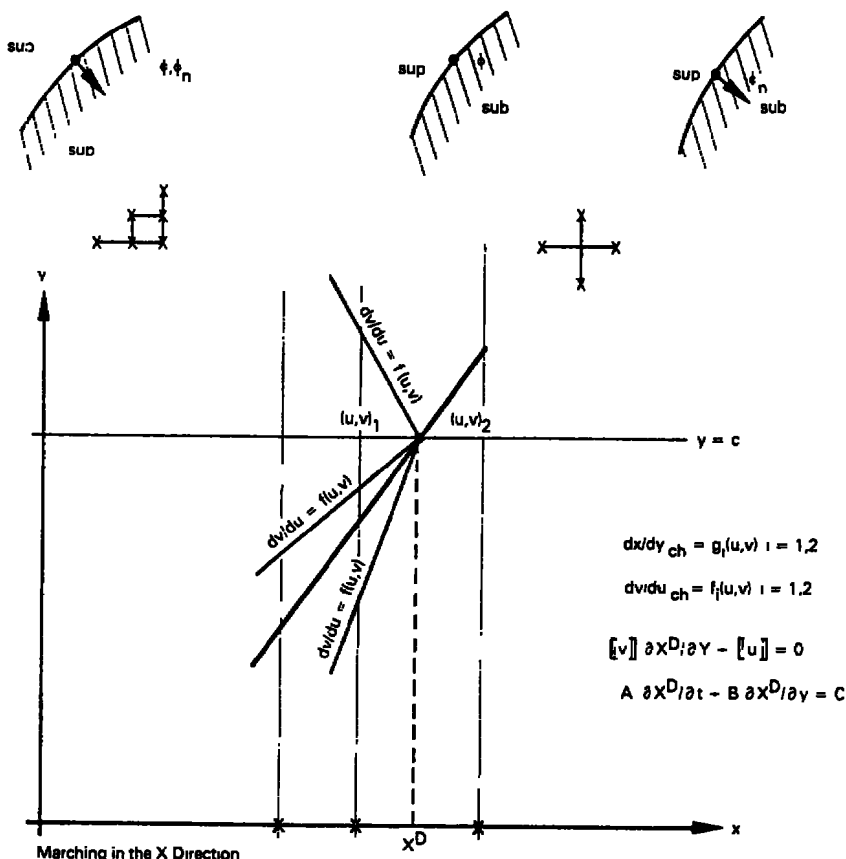
Sketch 2. Supersonic-Supersonic Shocks (Steady).
