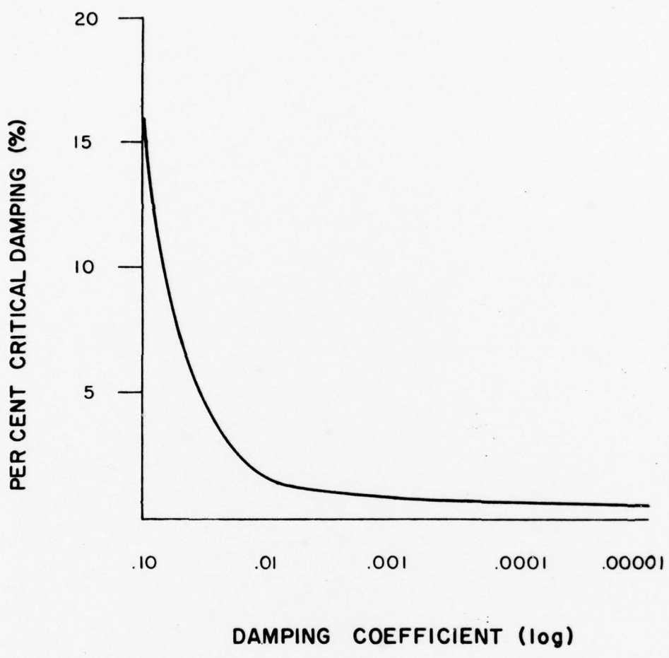
FIGURE IV-9. DAMPING RELATIONSHIPS FOR F3H STABILATOR
