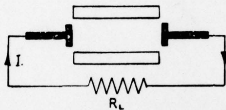
CONFIGURATION 1:- SIMPLE MHD GENERATOR - "B" FIELD SUPPLIED BY PERMANENT MAGNETS [1.4 TESLA - UBD = 12 VOLTS]
