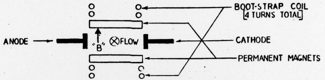
COMPONENT ARRANGEMENT - MHD GENERATOR
