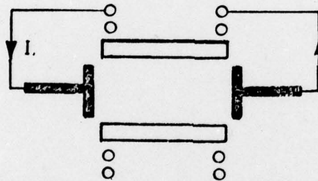
CONFIGURATION 3:- MHD GENERATOR - OUTPUT APPLIED TO BOOT-STRAP COIL TO INCREASE "B" FIELD
