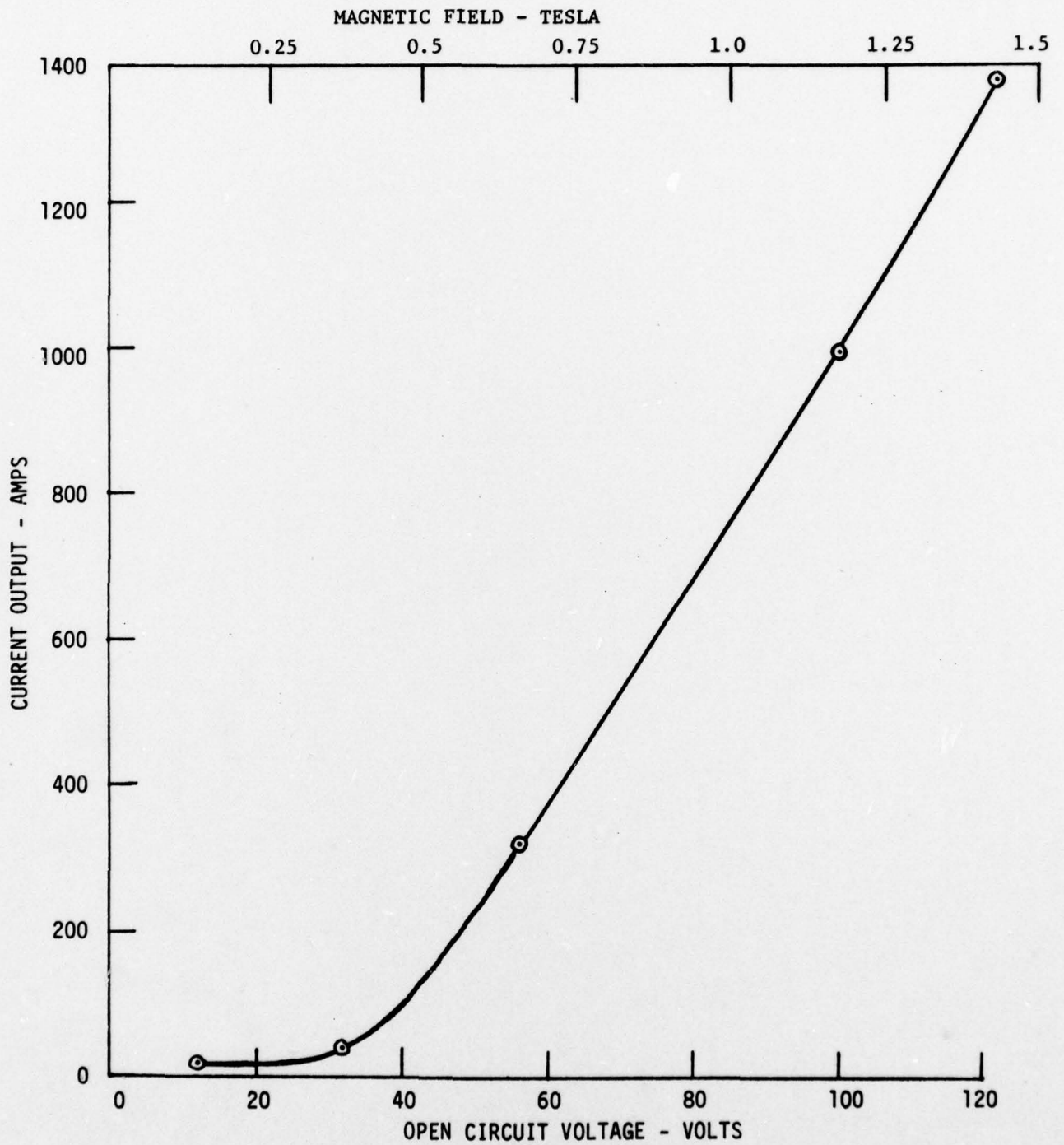
Figure 29. AMES II MHD CHANNEL CURRENT OUTPUT (50 mΩ LOAD) VERSUS OPEN CIRCUIT VOLTAGE. B FIELD SUPPLIED BY CAPACITOR BANK
