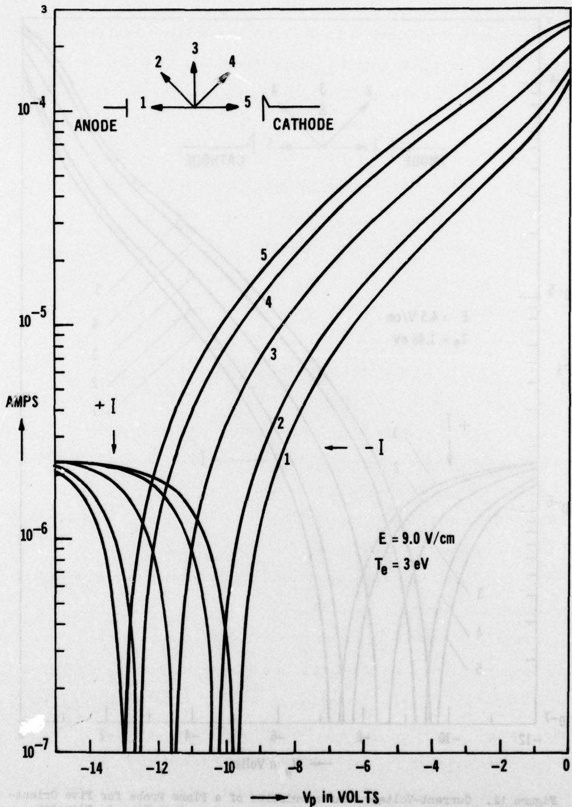
Figure 13. Current-Voltage Characteristics of a Plane Probe for Five Orientations when E = 9 V/cm, \eta = 10^{-6} and p = 0.14 Torr in Nitrogen
