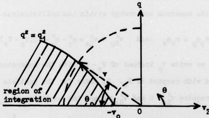
Figure 3. Spherical Velocity Space in the Retarding Region. If v < |v_0| , the integration region is nil. If v > |v_0| , the integration region lies between \theta = \pi - \theta_0 or q^2 = q_1^2 and \theta = \pi
