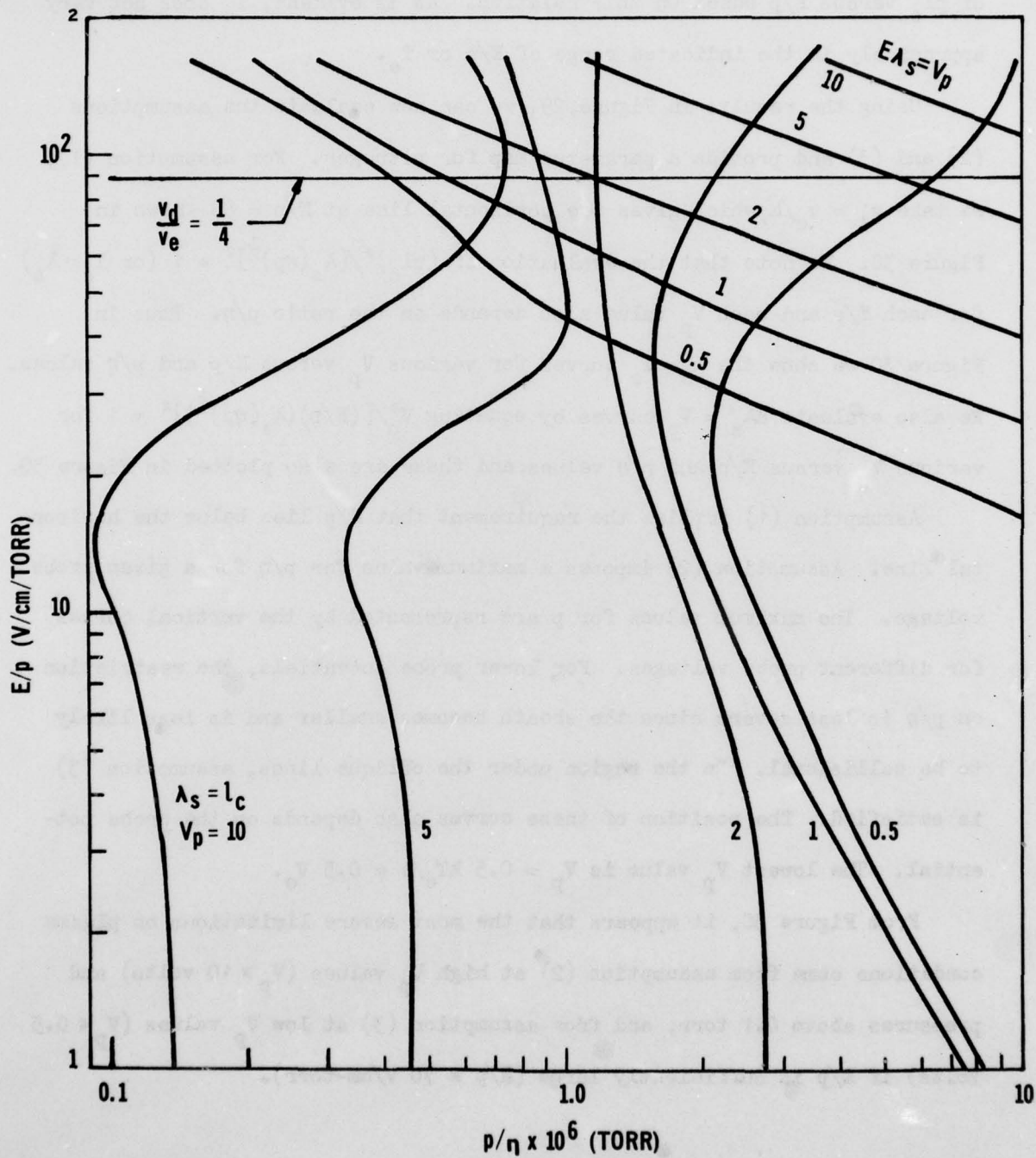
Figure 30. Parameter Map for Nitrogen Showing Various Limits on a E/p Versus p/η Plot
