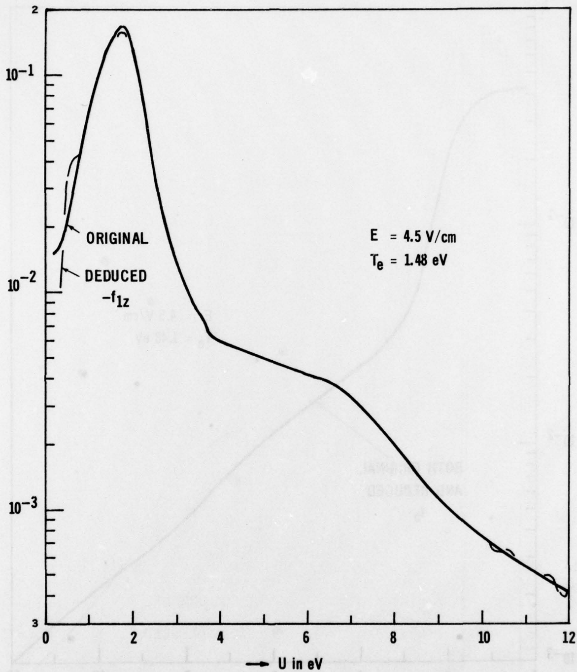
Figure 18. Comparison of Original f_{1z} with that Deduced from Program JTGF when E = 4.5 \text{ V/cm}
