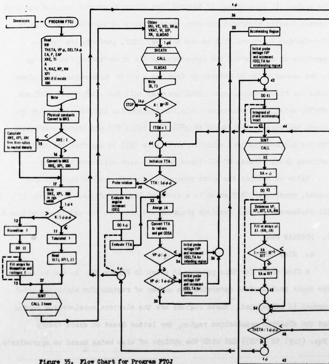
Figure 35. Flow Chart for Program FTOJ
