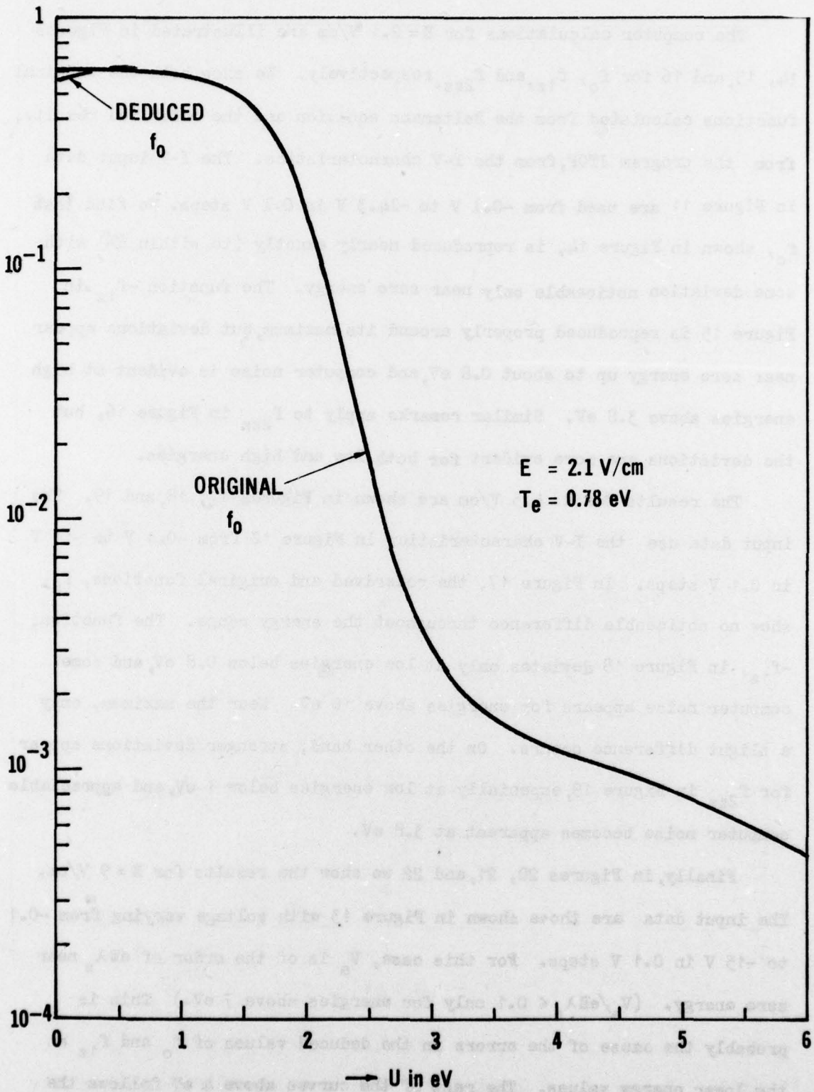
Figure 14. Comparison of Original f_0 with that Deduced from Program JTOF when E = 2.1 \text{ V/cm}
