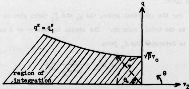
Figure 4. Spherical Velocity Space in the Accelerating Region. If v \leq |\sqrt{\beta}v_o| , the angle \theta varies from \pi/2 to \pi . If v > |\sqrt{\beta}v_o| , the angle \theta varies from \theta = \pi - \theta_o or q^2 = q_1^2 to \theta = \pi
