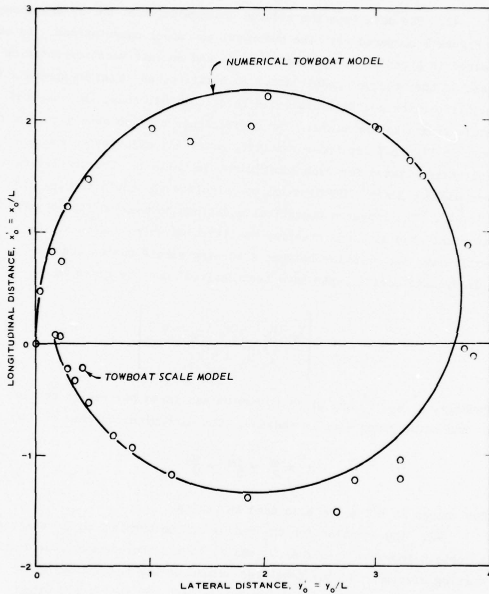
Figure 7. Physical and numerical model turning circle test comparison
