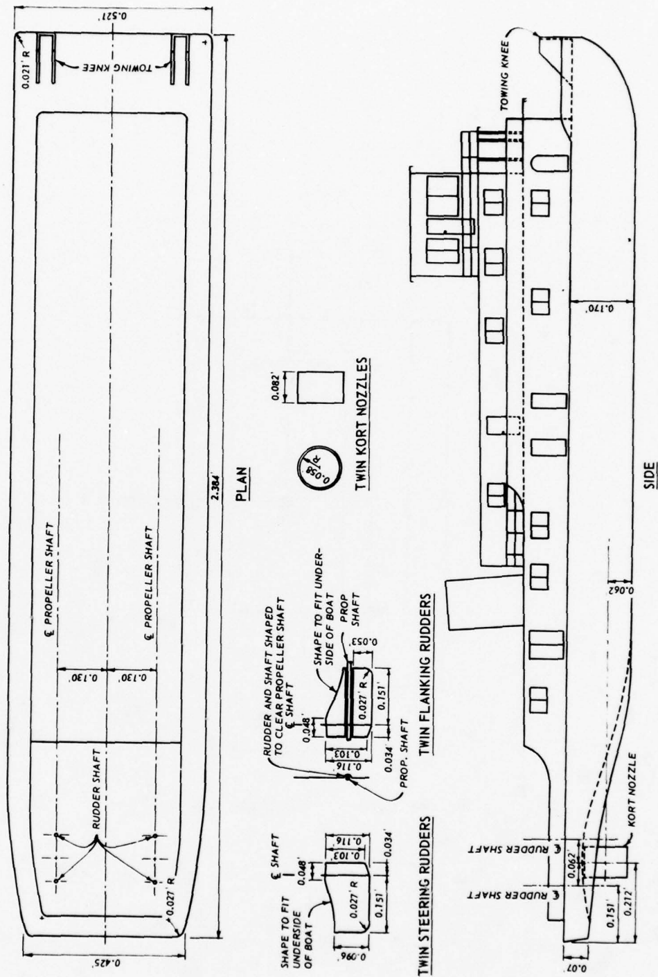
Figure 4. Model towboat characteristics
