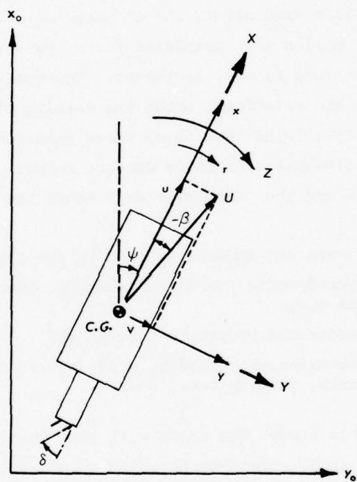
Figure 2. Coordinate axis of flotilla
