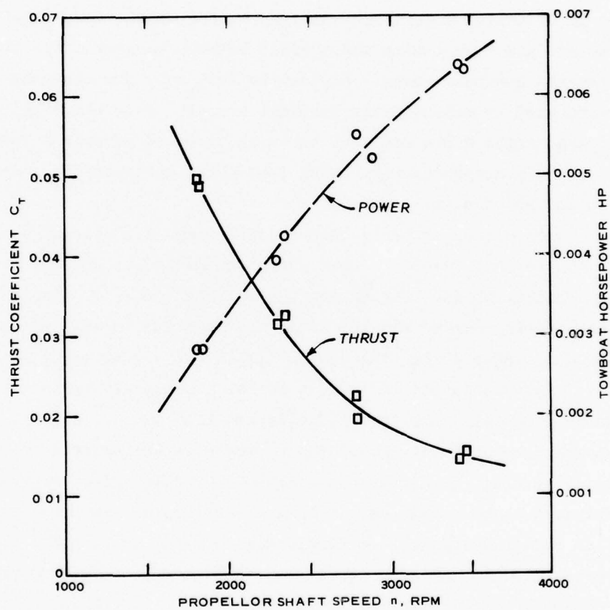
Figure 6. Model towboat propulsion characteristics
