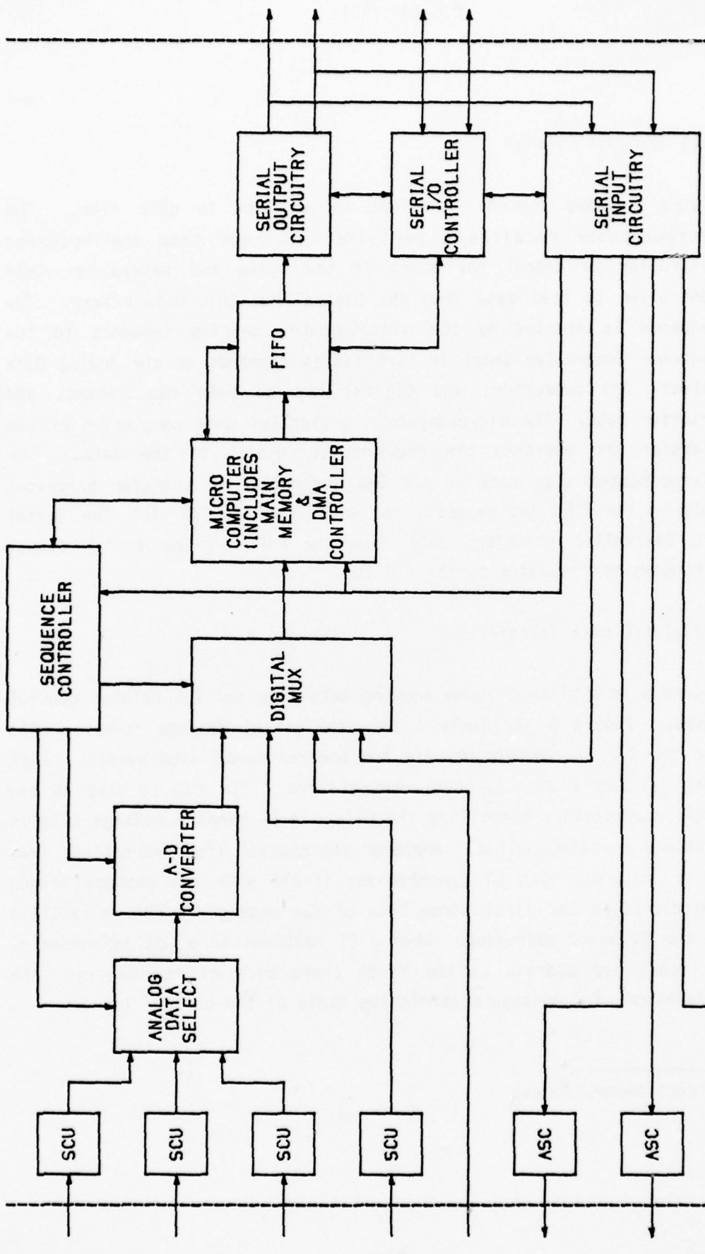
DATA TERMINAL (HALF) BLOCK DIAGRAM
