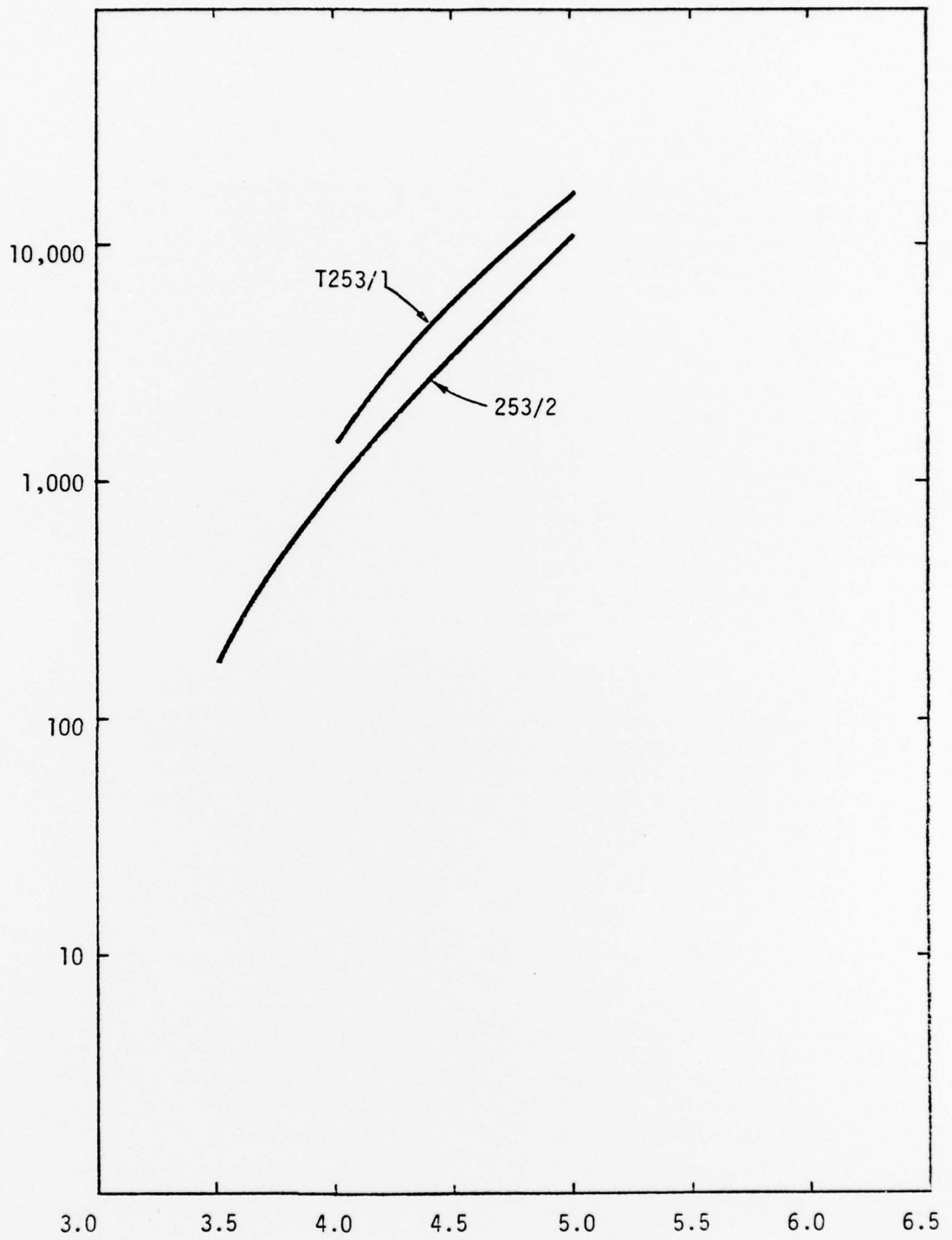
12 MM TRIPLE DIODE BRIGHTNESS GAIN VS. VOLTAGE
