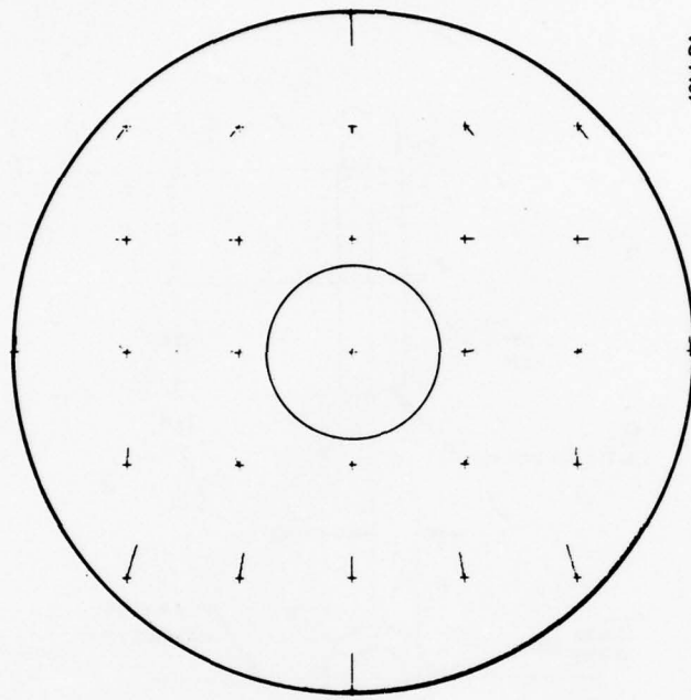
ANGULAR ERRORS ACROSS THE PUPIL FOR AXIAL FIELD POINT INNER CIRCLE REPRESENTS A 3 MM PUPIL
