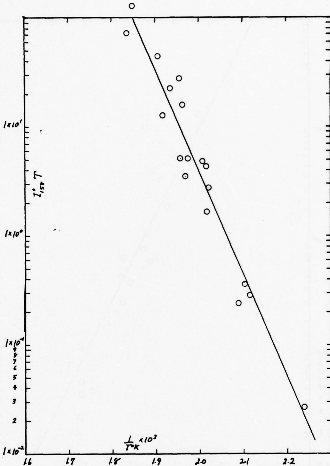
Figure 2: \log \frac{L_{158} T}{T^4} vs 1/T plot for the data of 2\text{BeCl}_2(\text{s}) = (\text{BeCl}_2)_2(\text{g}) , \Delta H_{158}^\circ = 44.5 \text{ kcal/mol.}
