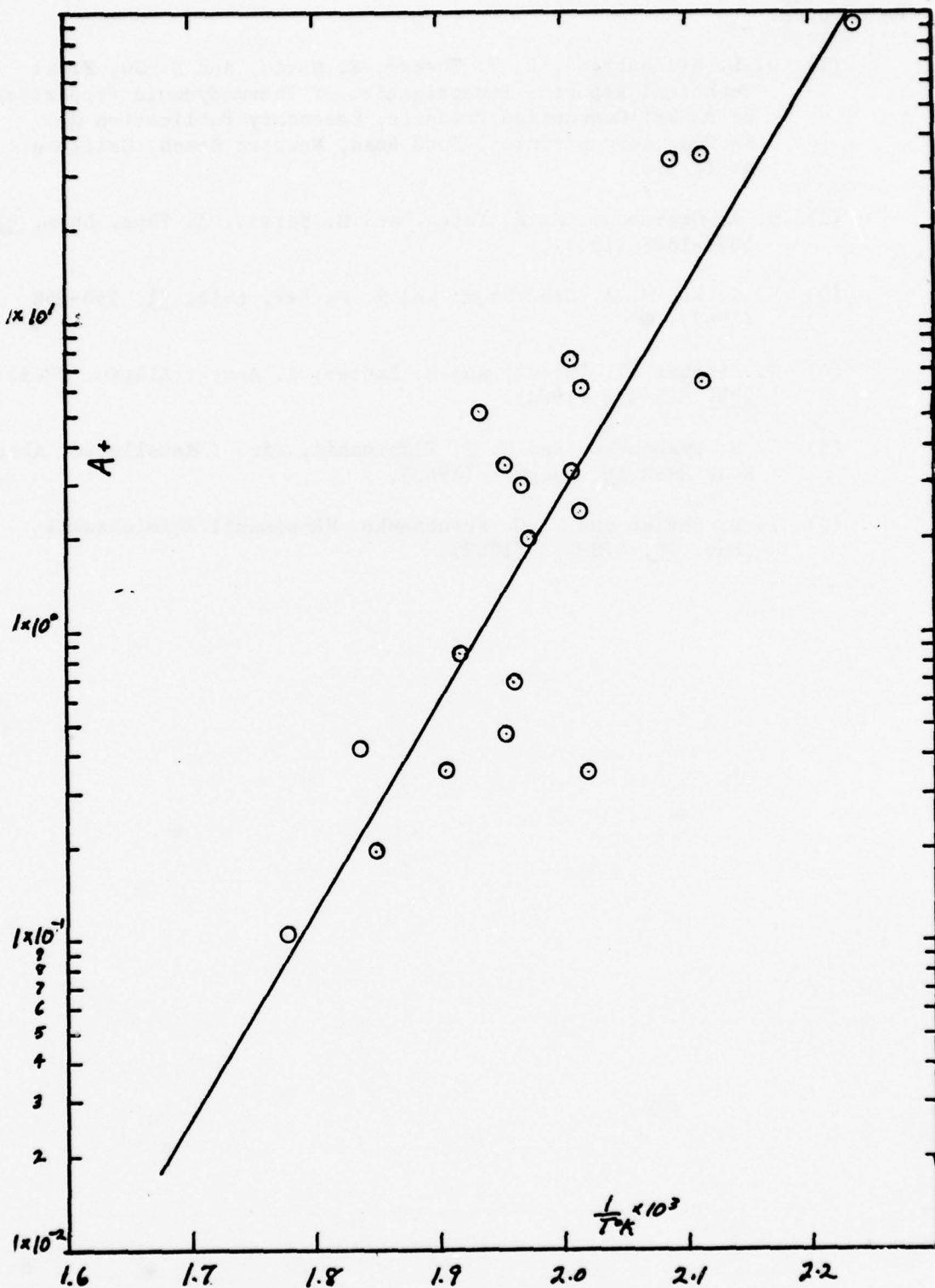
Figure 3: \log A_+ vs 1/T plot for the data of 2\text{BeCl}_2(\text{g}) = (\text{BeCl}_2)_2(\text{g}) , \Delta H_{513}^\circ = -30.7 kcal/mol.
