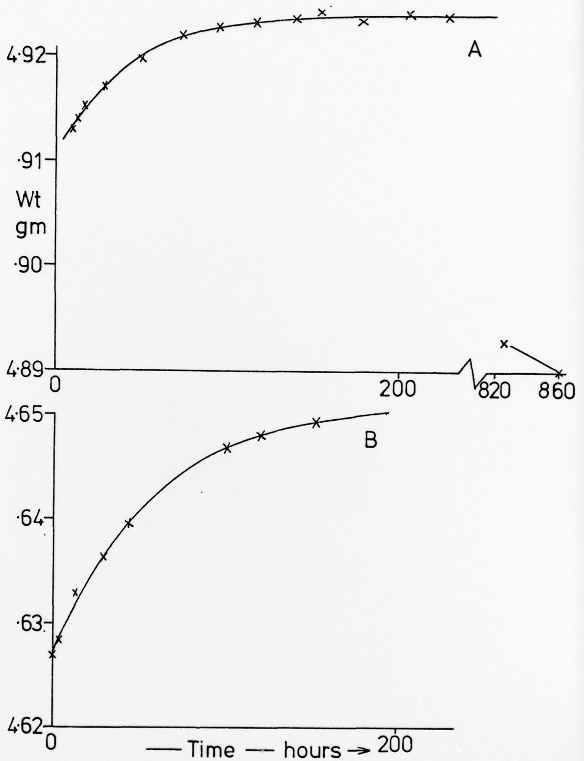
Figure 14. Weight of GRP against boiling time for specimens A & B
