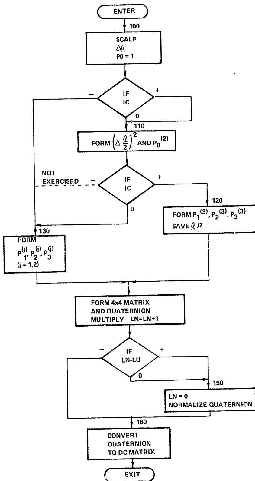
Figure 2-8. Flow Chart for 1st, 2nd, and 3rd Order Quaternion Update
