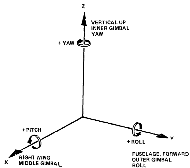
Figure 1-2. Aircraft and KT-73 Gimbal Axes
