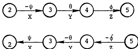
Figure A-13. Body to Local Vertical Transformations
