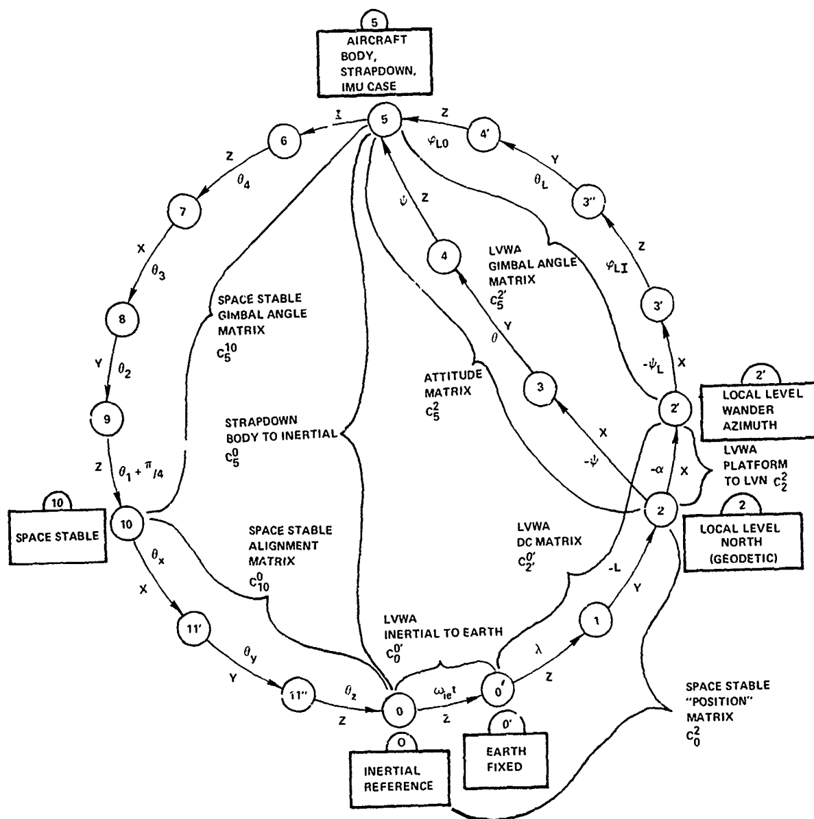
Figure 6-5. General Circle Diagram for SS, SD, LVWA INS Computations
