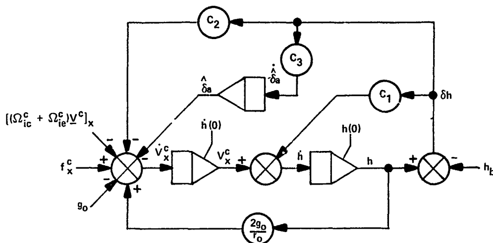
Figure 2-10. Third Order Damped Vertical Block Diagram
