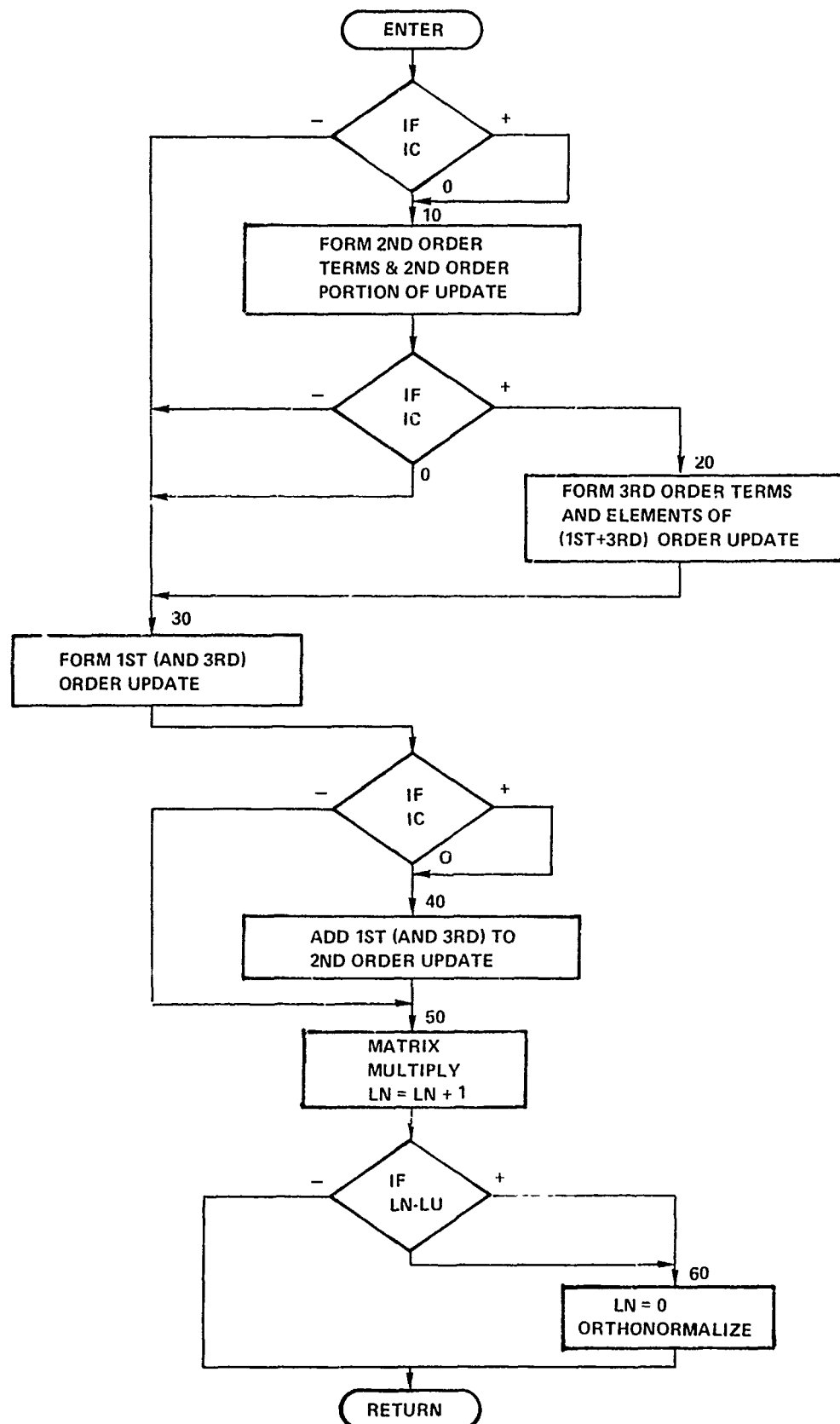
Figure 2-7. Flow Chart for 1st, 2nd or 3rd Order Direction Cosine Update Matrix
