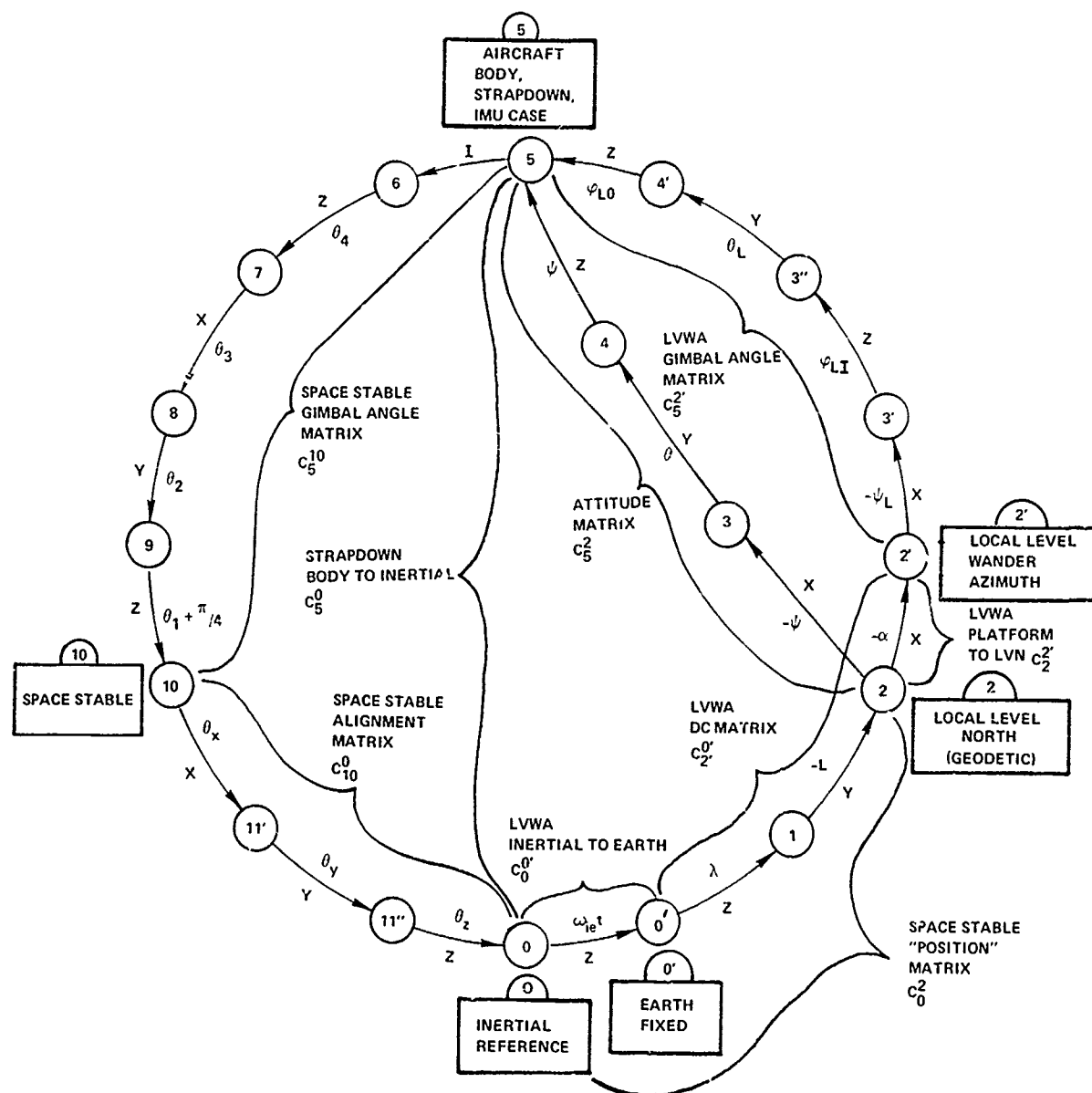
Figure A-9. General Circle Diagram for SS, SD, LVWA INS Computations
