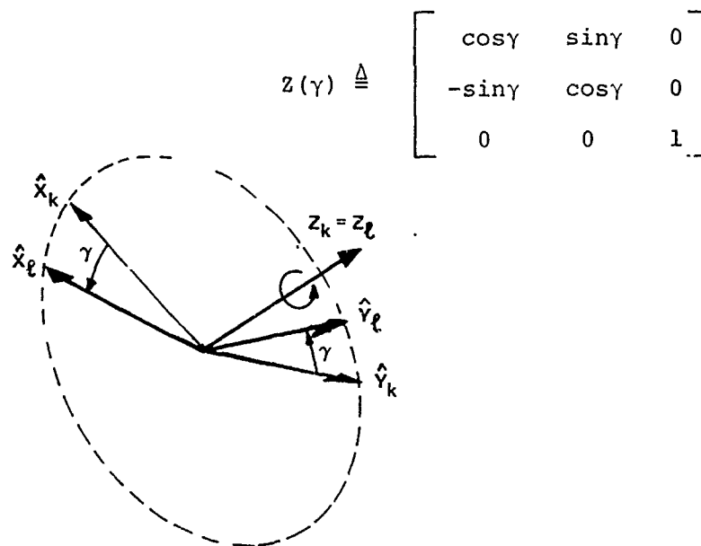
Figure A-5. Rotation About Z-axis
