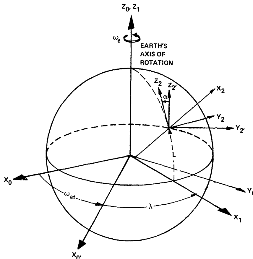
Figure 6-3. Frames Used in SPN/GEANS Computations
