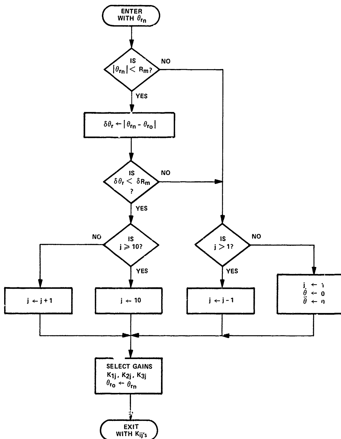
Figure 2-12. Attitude Filter Gain Select Logic for a Single Axis
