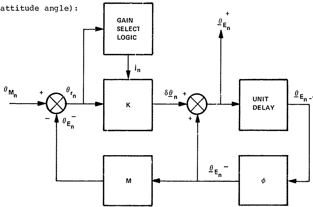
Figure 2-11. Attitude Predictor-Filter Block Diagram (Single Axis)
