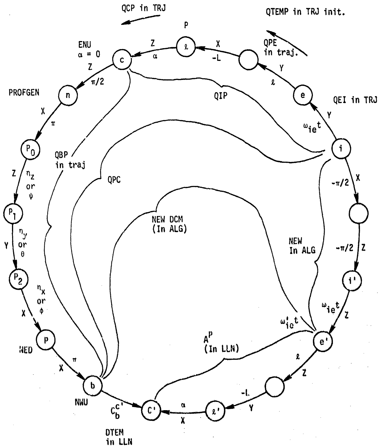
Figure B-3. INSS body-to-LVWA computational frame, C_b^{c'} (circle diagram).
