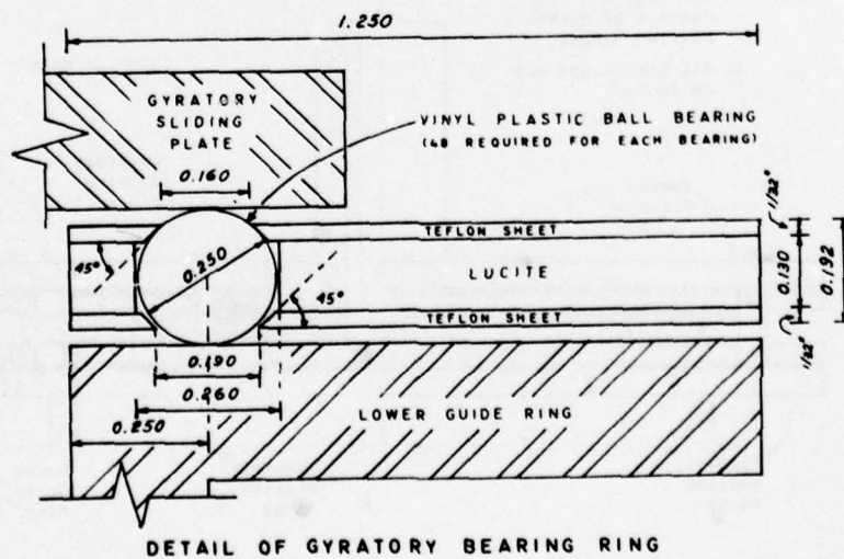
Fig. A6. Gyratory bearing (2 required)
