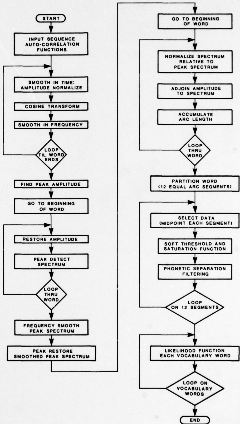
FIGURE 1A VOICE RECOGNITION PROGRAM FLOW DIAGRAM.
