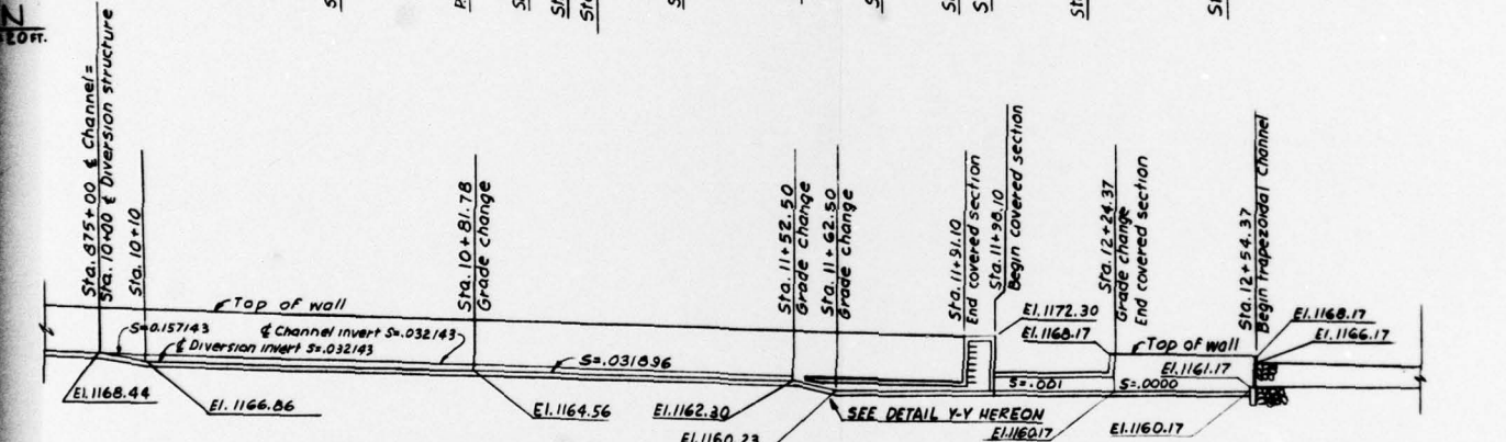
PROFILE - t DIVERSION CHANNEL SCALE: 1" = 20 FT.
