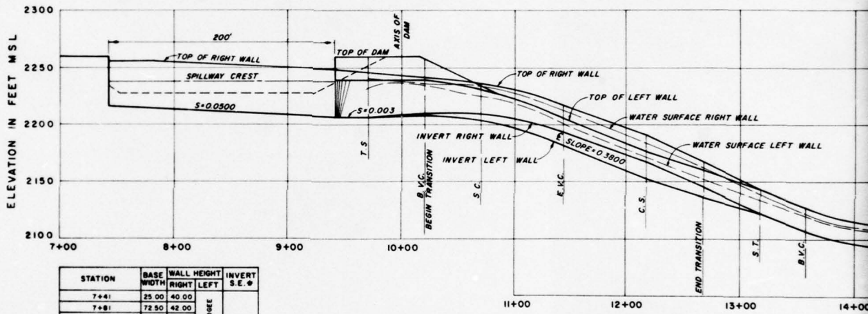
STATIONS ALONG CENTERLINE WATER-SURFACE PROFILES DISCHARGE 54,000 CFS
