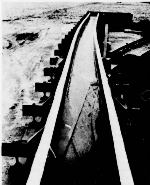
Photo A6. Looking downstream with diversion gate open, Q = 125 cfs
