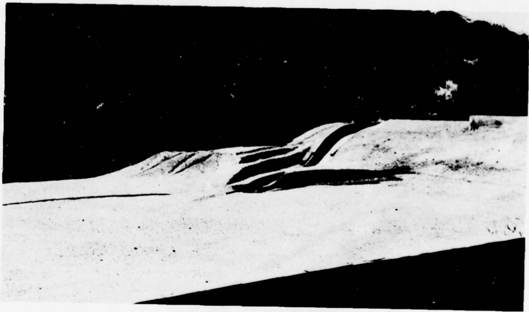
Photo 3. Final design, 1:48-scale model, general view of spillway chute and bucket
