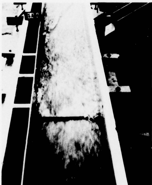
Photo A23. Looking downstream. 700 cfs in main channel, with 425 cfs flowing into the diversion structure with gate fully open. Balance passing down main channel. A heavy spray 15 ft high occurred at the entrance of diversion structure, evenly distributed across channel
