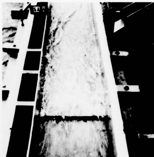
Photo A22. Looking downstream. 600 cfs in main channel, with 400 cfs flowing into the diversion structure with gate fully open. A heavy spray 15 ft high occurred at the entrance of the diversion structure with even distribution across channel
