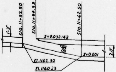
DETAIL Y-Y
