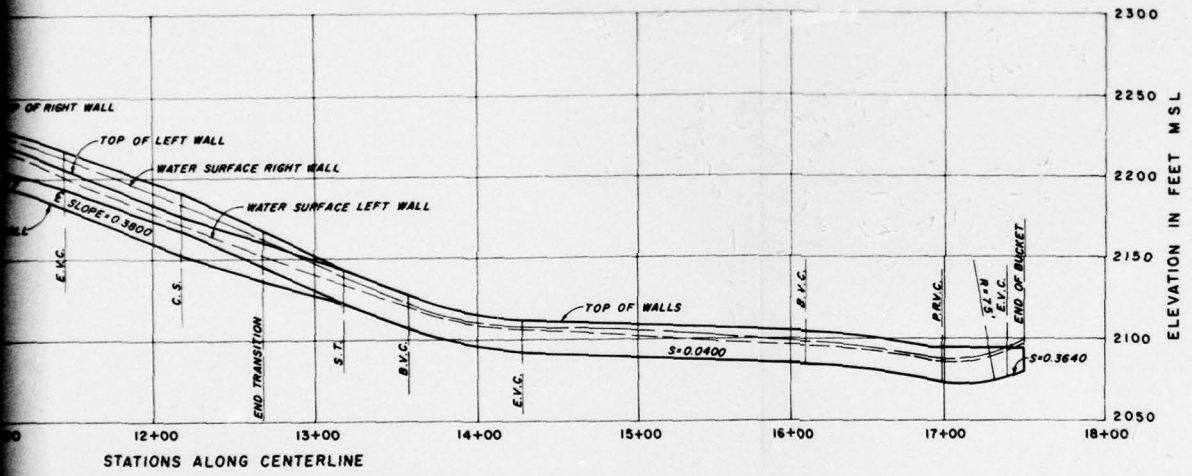
WATER-SURFACE PROFILES DISCHARGE 54,000 CFS
