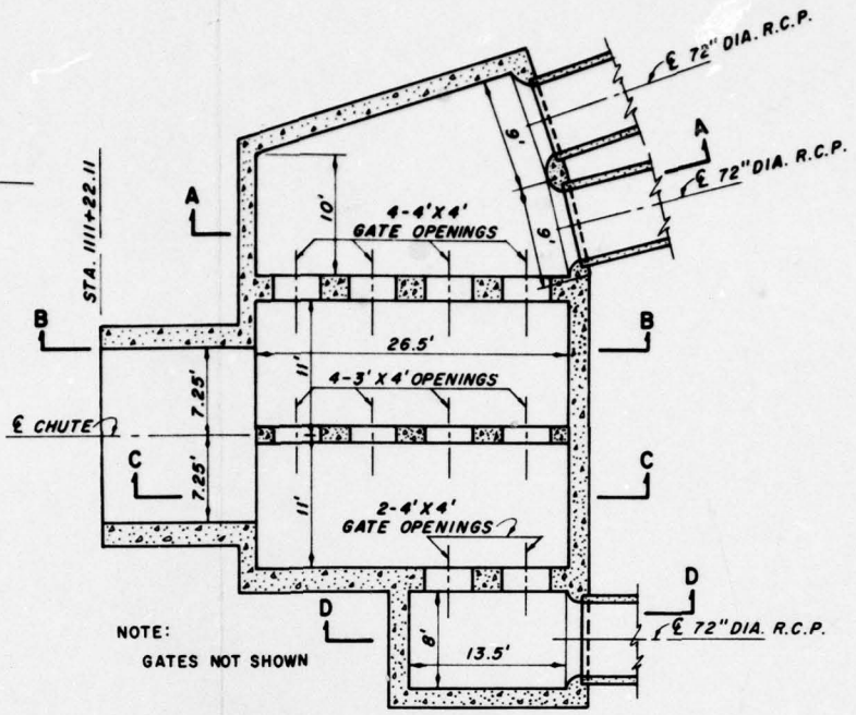
DIVERSION CHAMBER SECTIONAL PLAN
