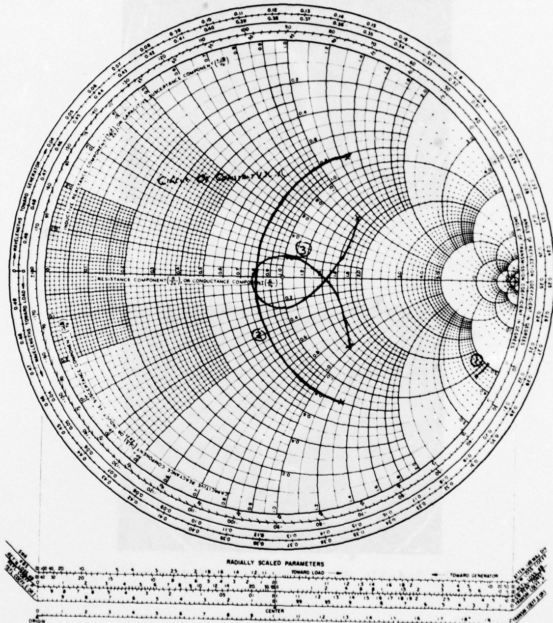
Figure 29 Matching of High Q Transducer
