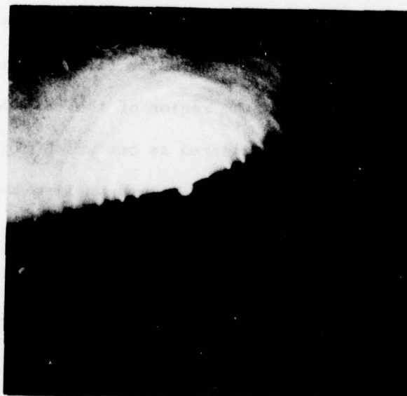
(b) Electron Diffraction Pattern for a 3 \mu\text{m} Thick ZnO Film Sputtered over 5 \mu\text{m} of Thermally Grown \text{SiO}_2
