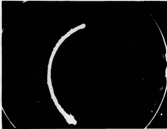
(a) 432-550 MHz Transducer Resonated with L_1
