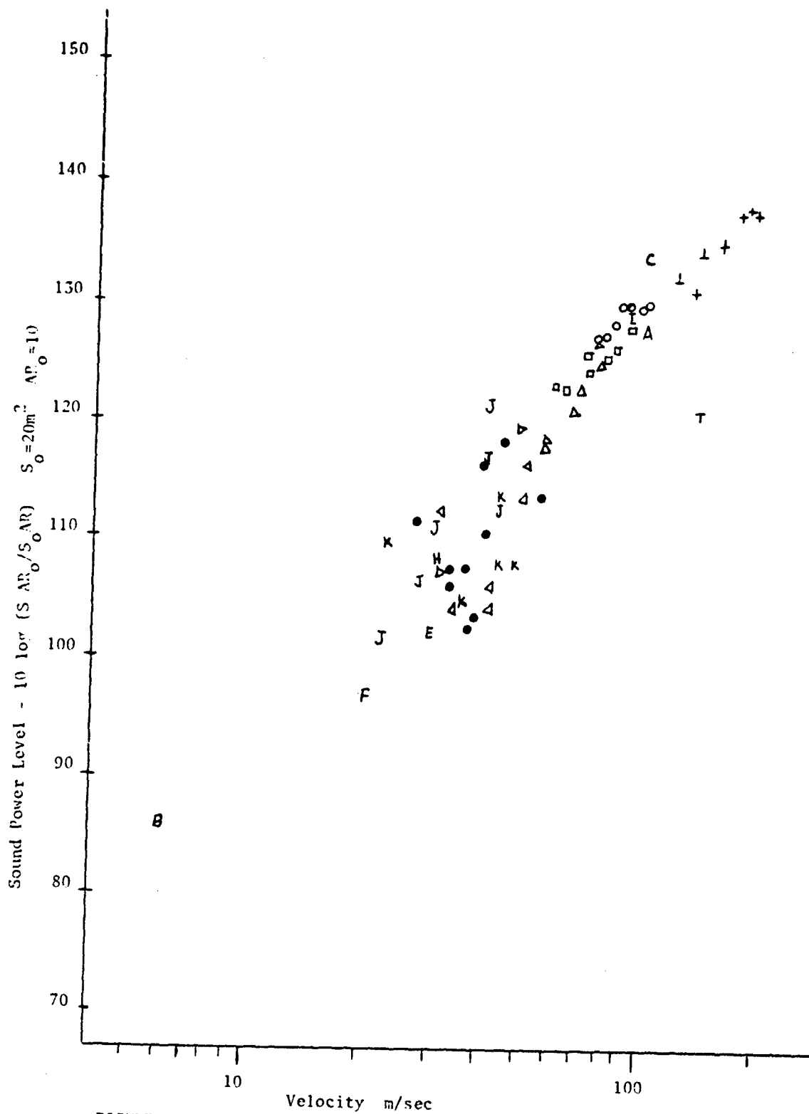
FIGURE 30 Acoustic Power Levels Normalized with S/AR
