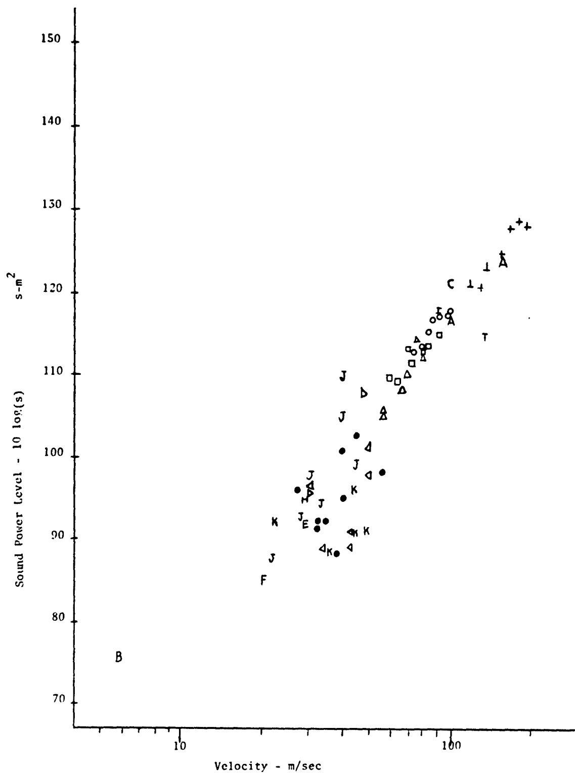
FIGURE 31 Acoustic Power Level Normalized with S 69
