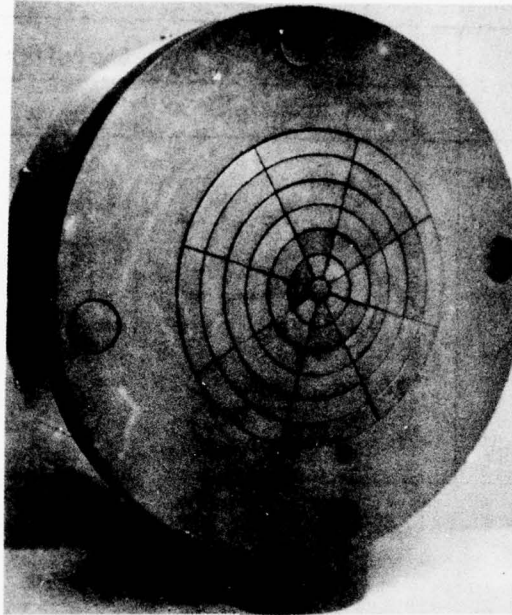
Figure 8. Graphite beam mapping calorimeter head.
