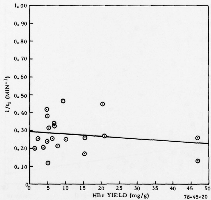
FIGURE 20. CORRELATION OF 1/t_1 VALUES WITH NONZERO HBr YIELDS
