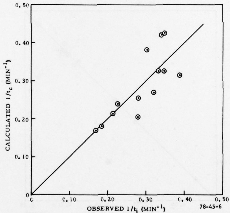
FIGURE 6. PANELS - COMPARISON OF CALCULATED AND OBSERVED 1/t_1 VALUES
