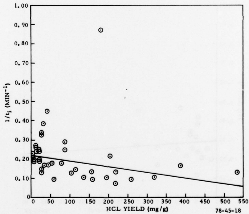
FIGURE 18. CORRELATION OF 1/t_1 VALUES WITH NONZERO HCL YIELDS
