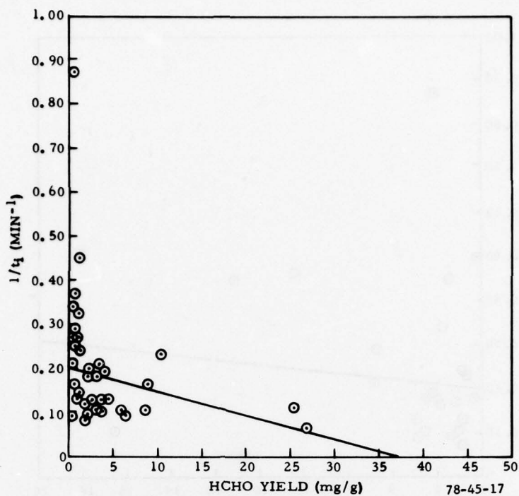
FIGURE 17. CORRELATION OF 1/t_1 VALUES WITH NONZERO HCHO YIELDS
