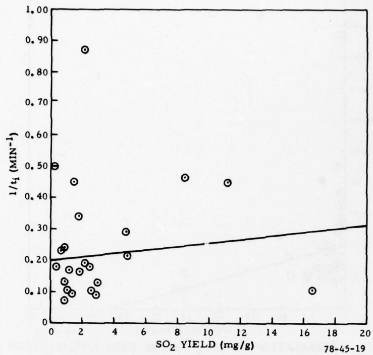
FIGURE 19. CORRELATION OF 1/t_1 VALUES WITH NONZERO SO 2 YIELDS
