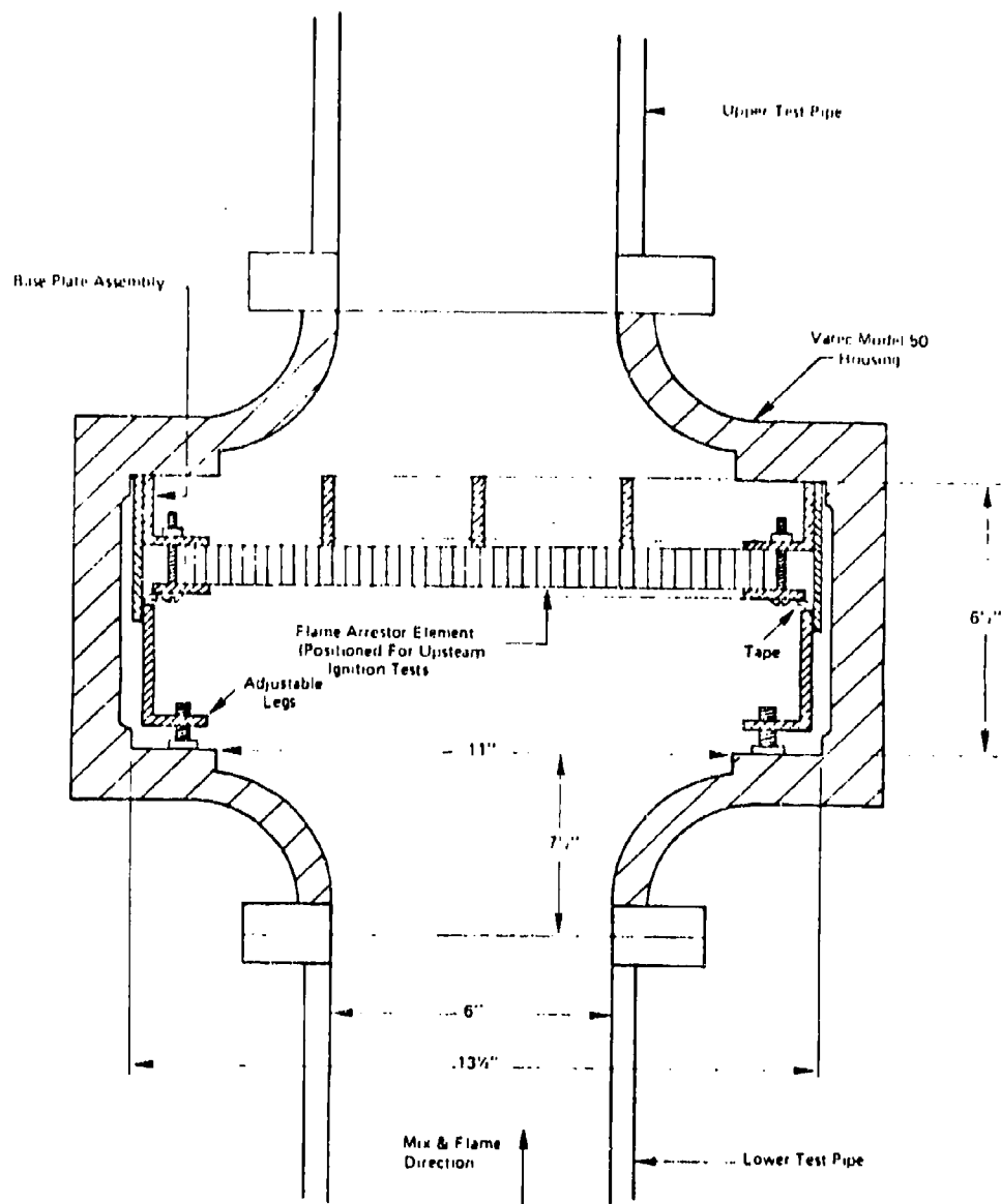
FIGURE 4 HOUSING FOR EXPERIMENTAL FLAME ARRESTORS
