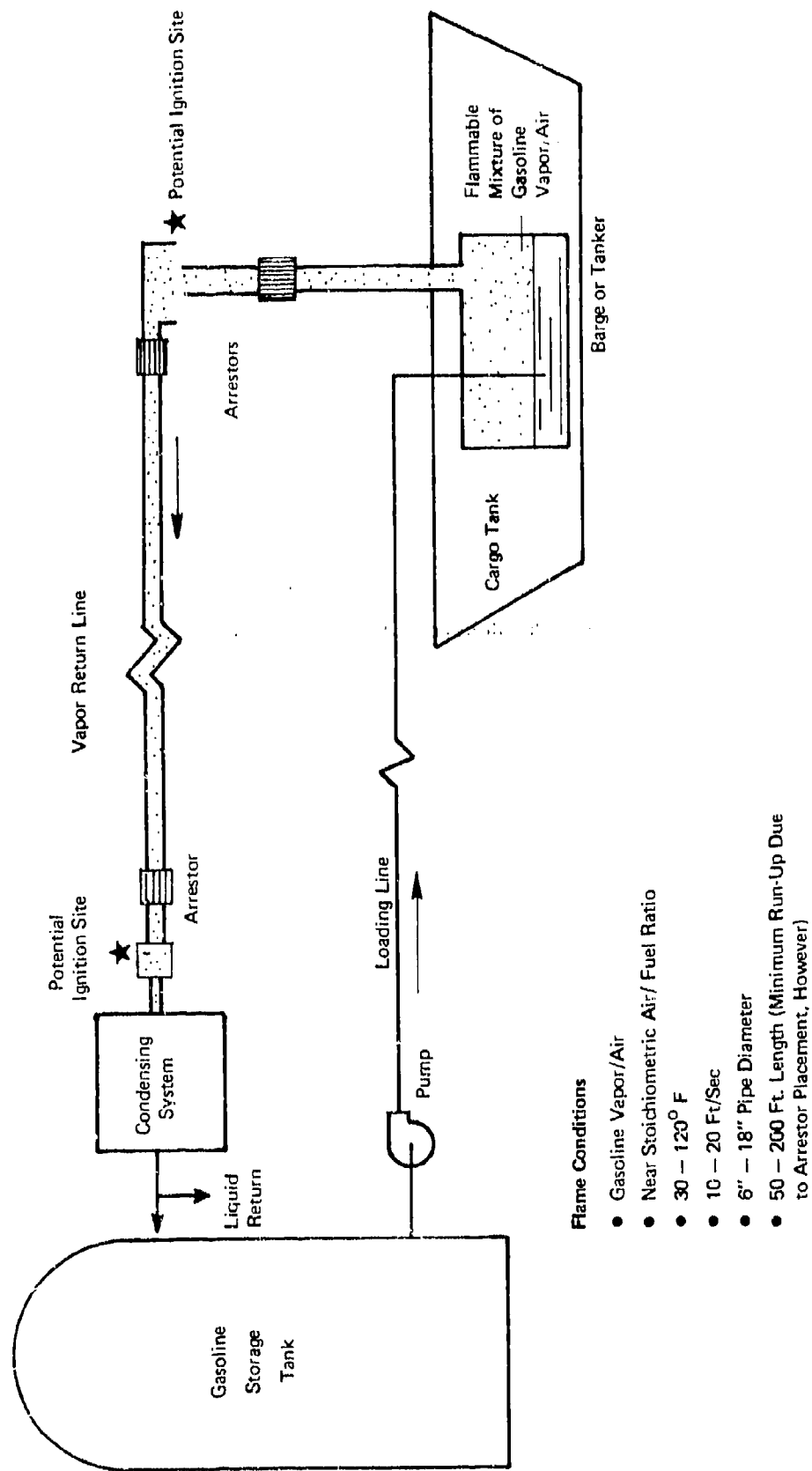
FIGURE 1: SCHEMATIC OF FLAME HAZARDS IN VAPOR RECOVERY SYSTEMS (LOADING TERMINAL)
