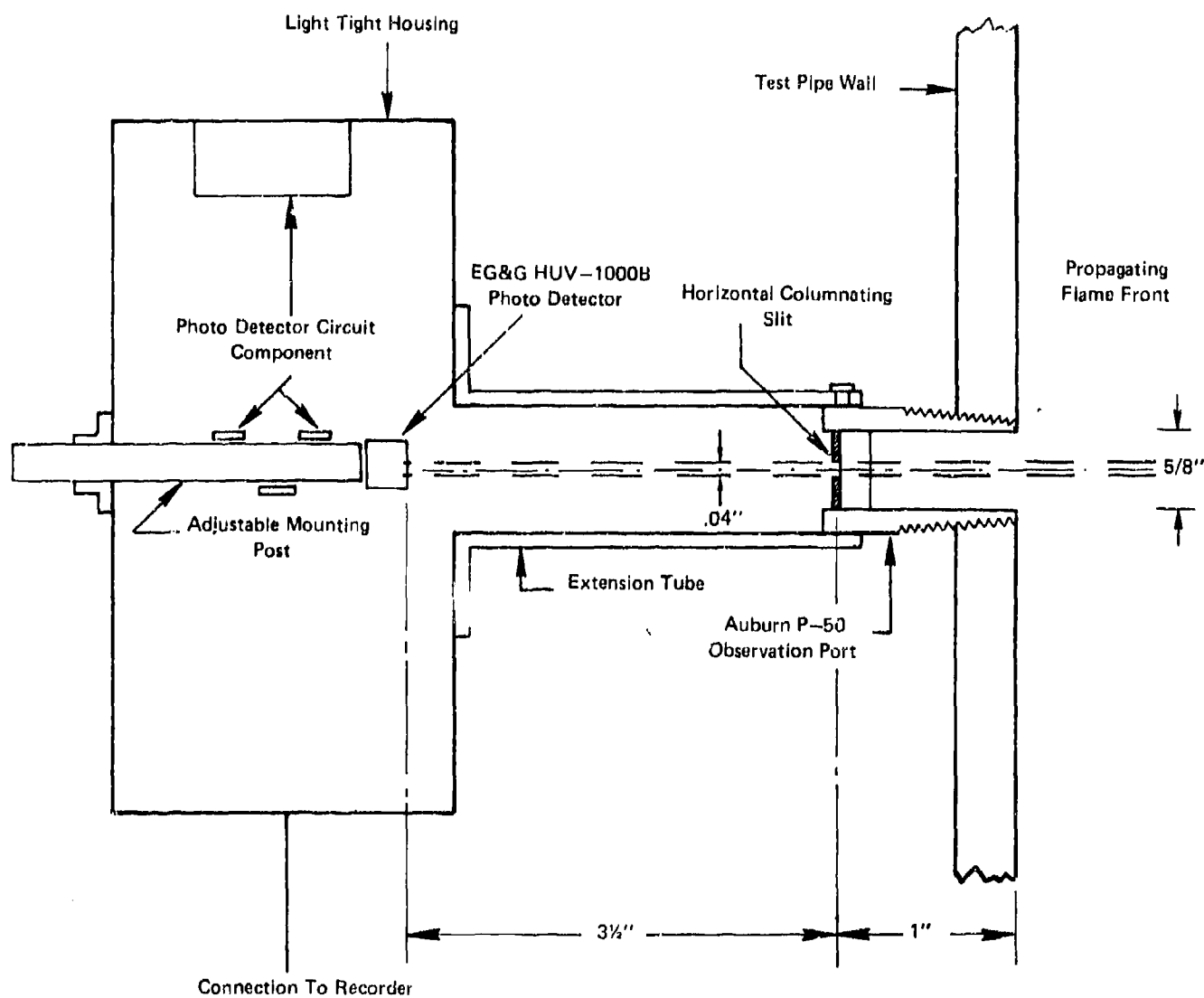
FIGURE 6 PHOTODETECTOR ARRANGEMENT
