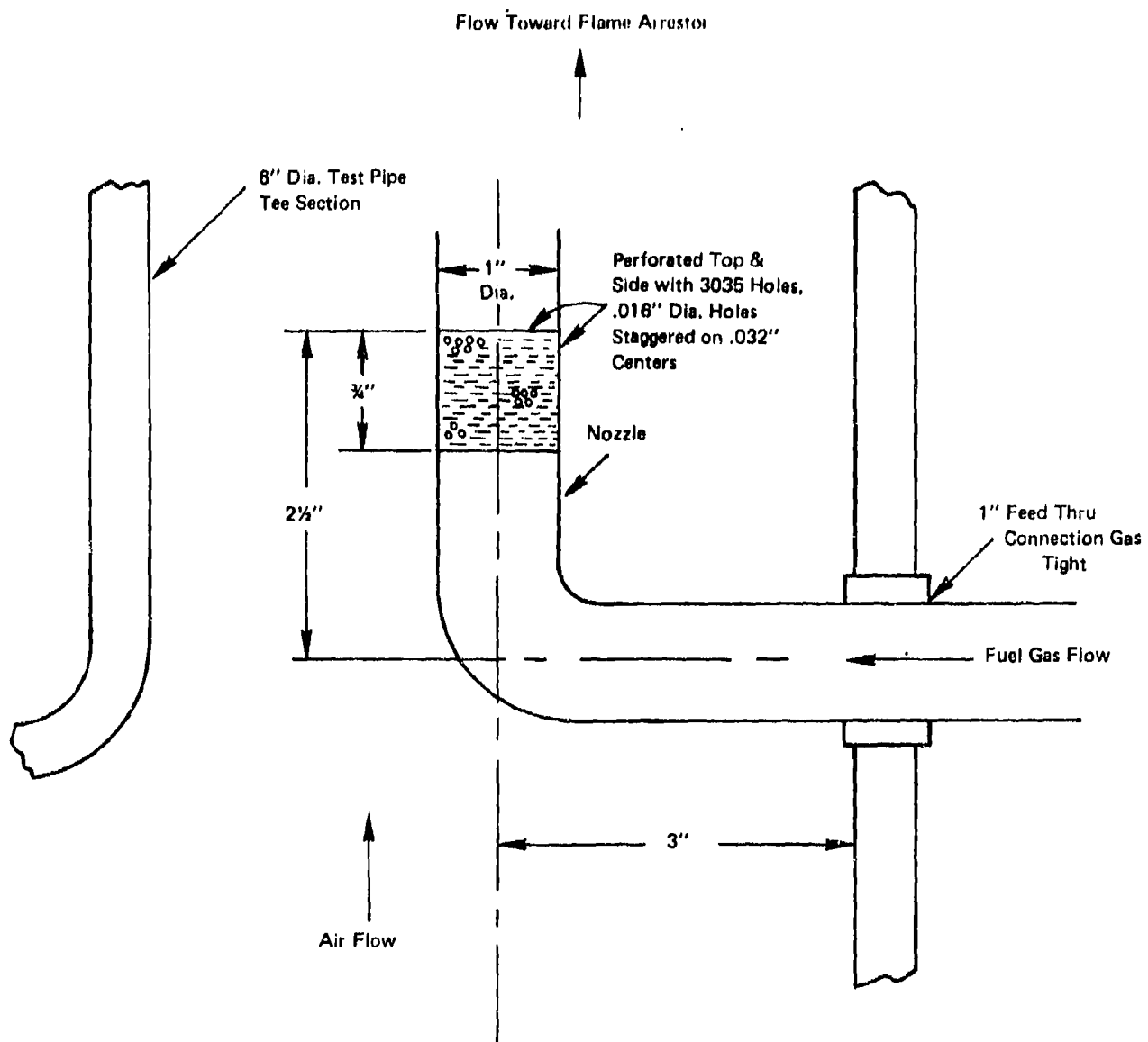
FIGURE 5 FUEL NOZZLE ARRANGEMENT
