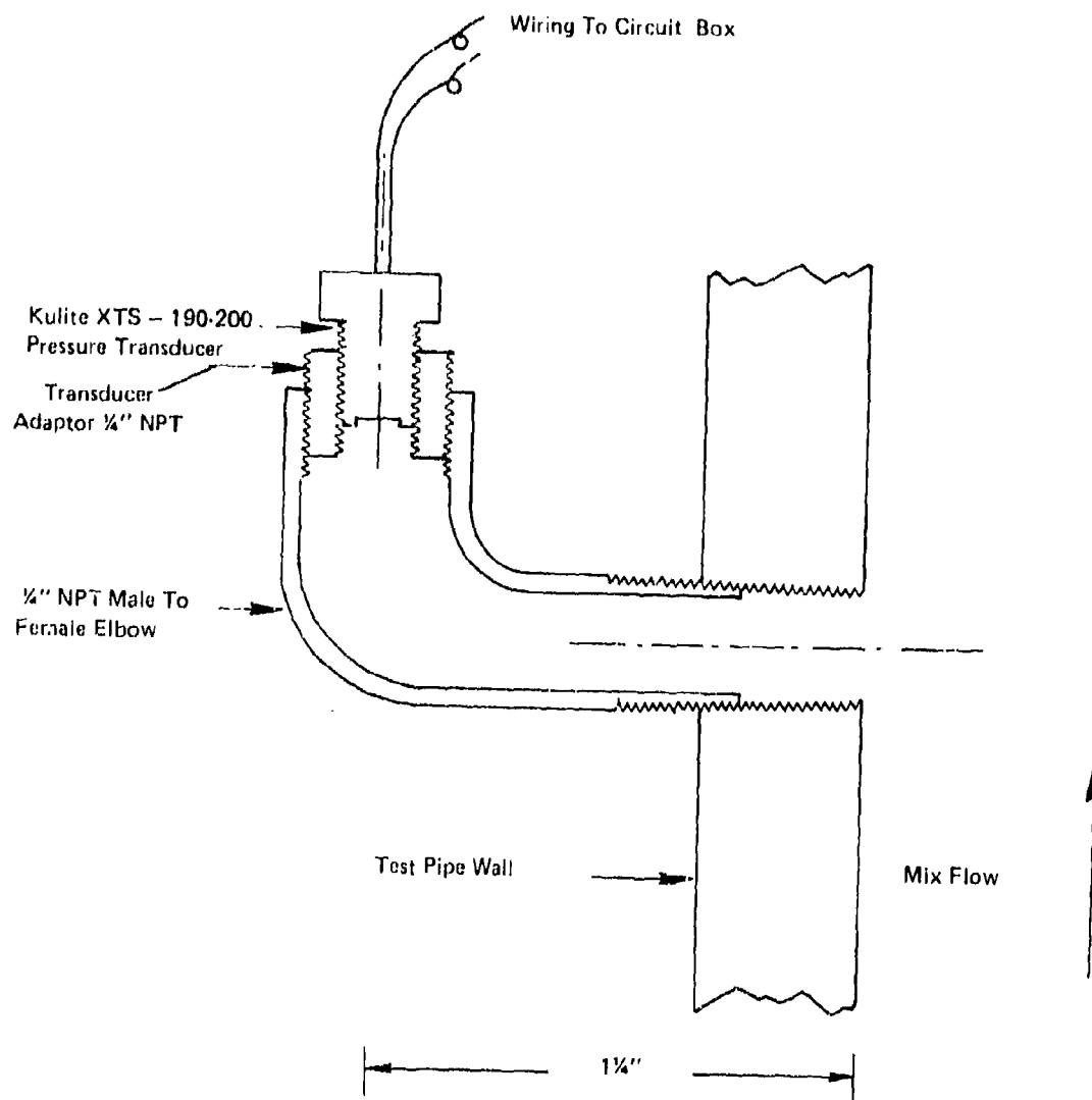
FIGURE 7 DETAIL OF PRESSURE TRANSDUCER MOUNTING
