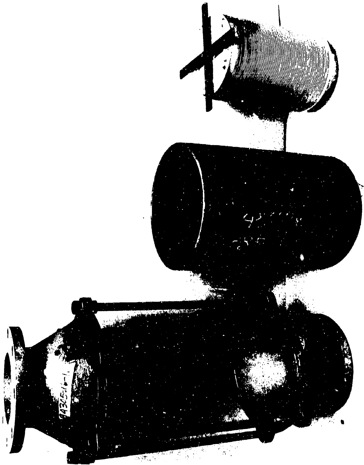
Figure 18: Parallel plate arrester, radial flow (Protectoseal, .031" gap)
