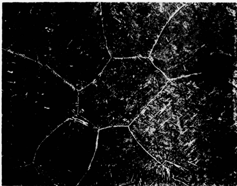
Fig 4 Alloy quenched from 1000°C showing as-solidified \beta grain size (x 100)
