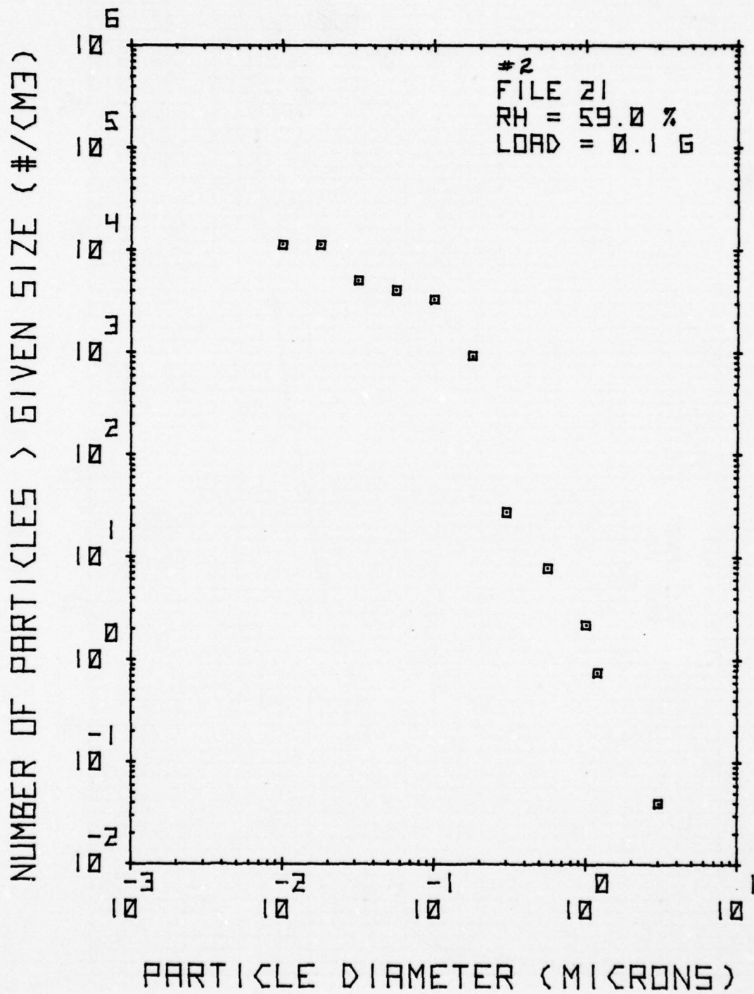
AEROSOL SPECTRUM FOR EXPERIMENT #2
