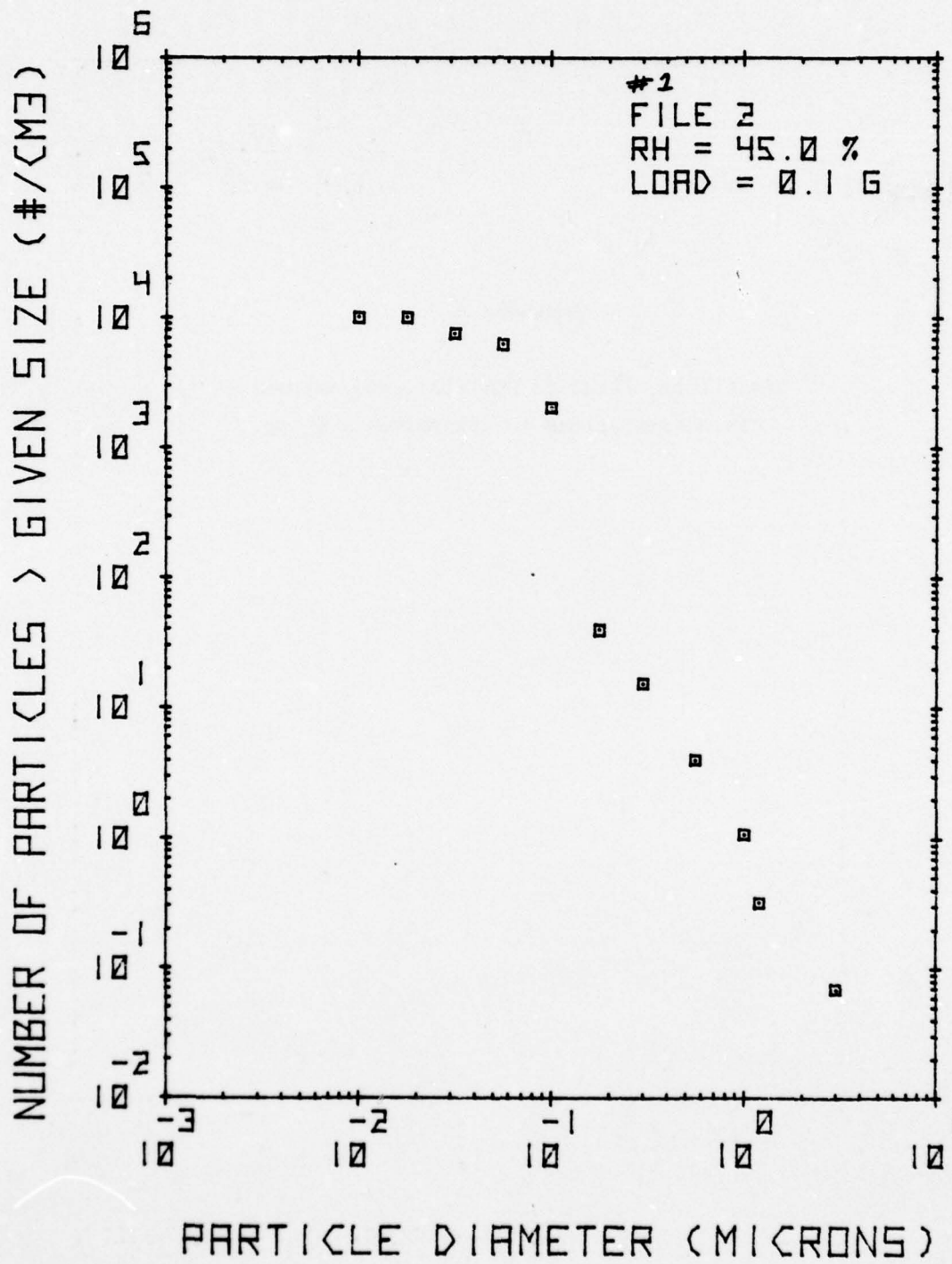
AEROSOL SPECTRUM FOR EXPERIMENT #1
