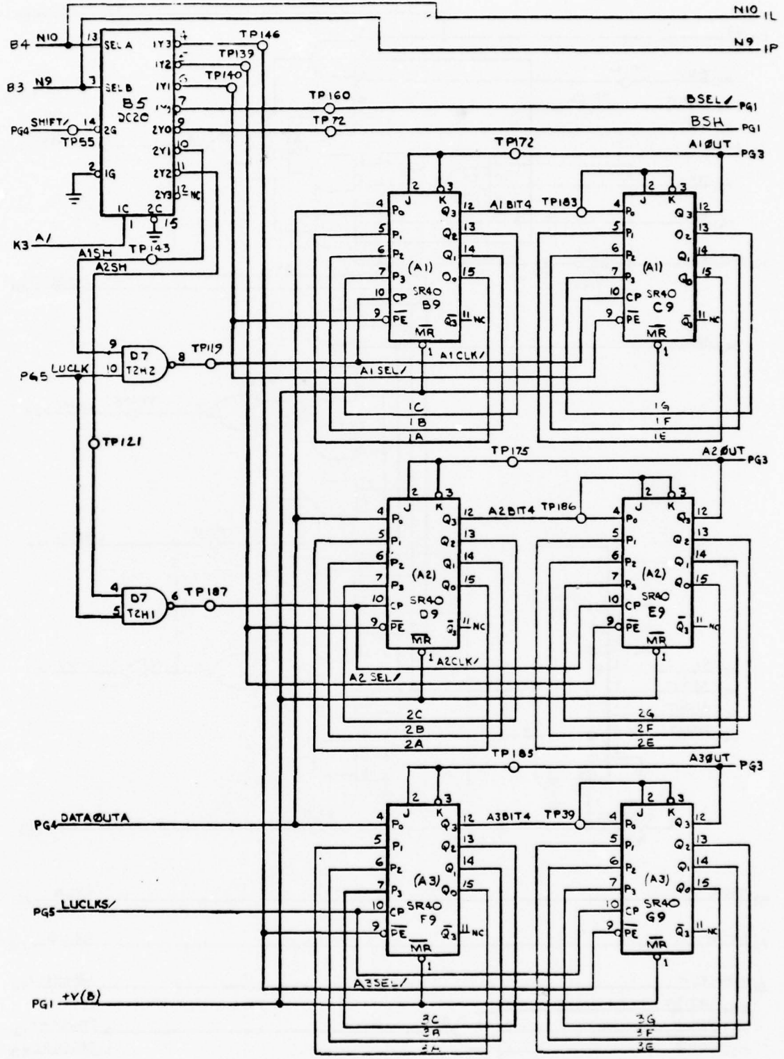
Figure 5-14. NCU and CIE MD2 Board Logic (Sheet 2 of 5)
