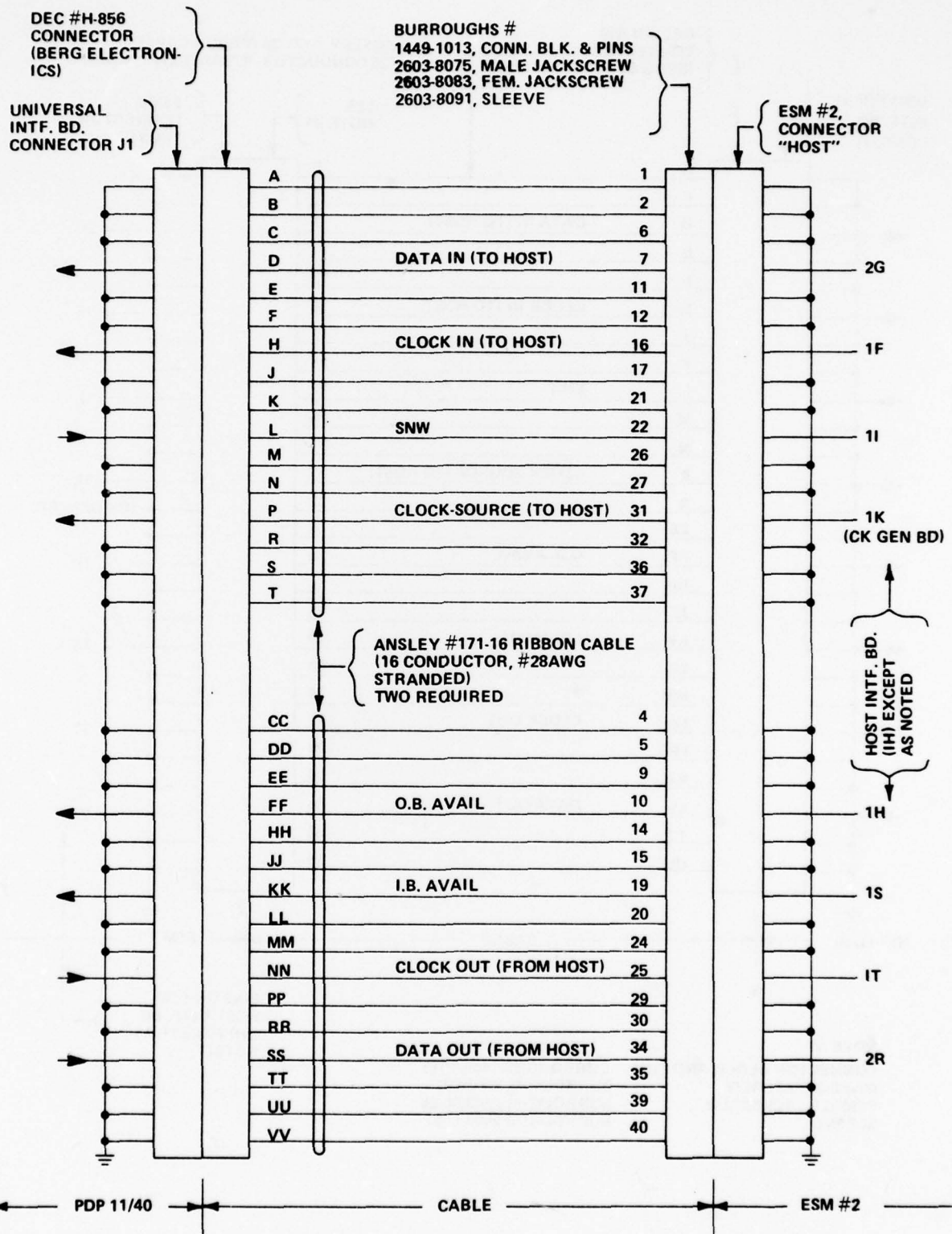
Figure 5-50. Cable, ESM No. 2 to Host No. 2
