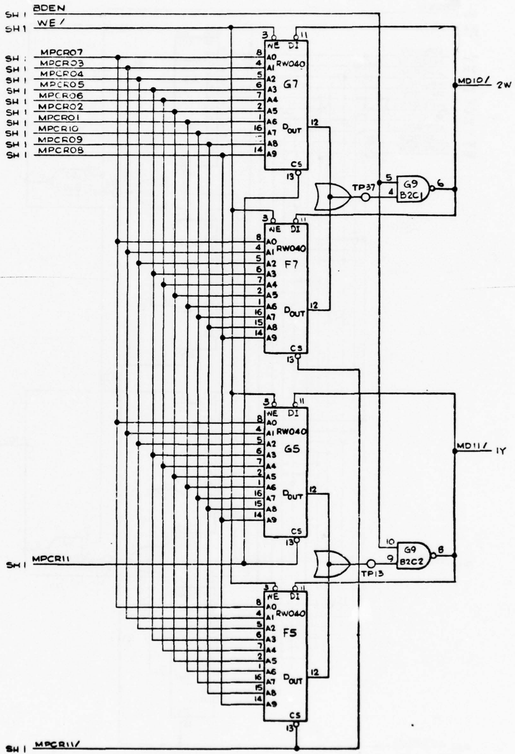
Figure 5-16. CIE Control Memory Logic (Sheet 6 of 7 Sheets)
