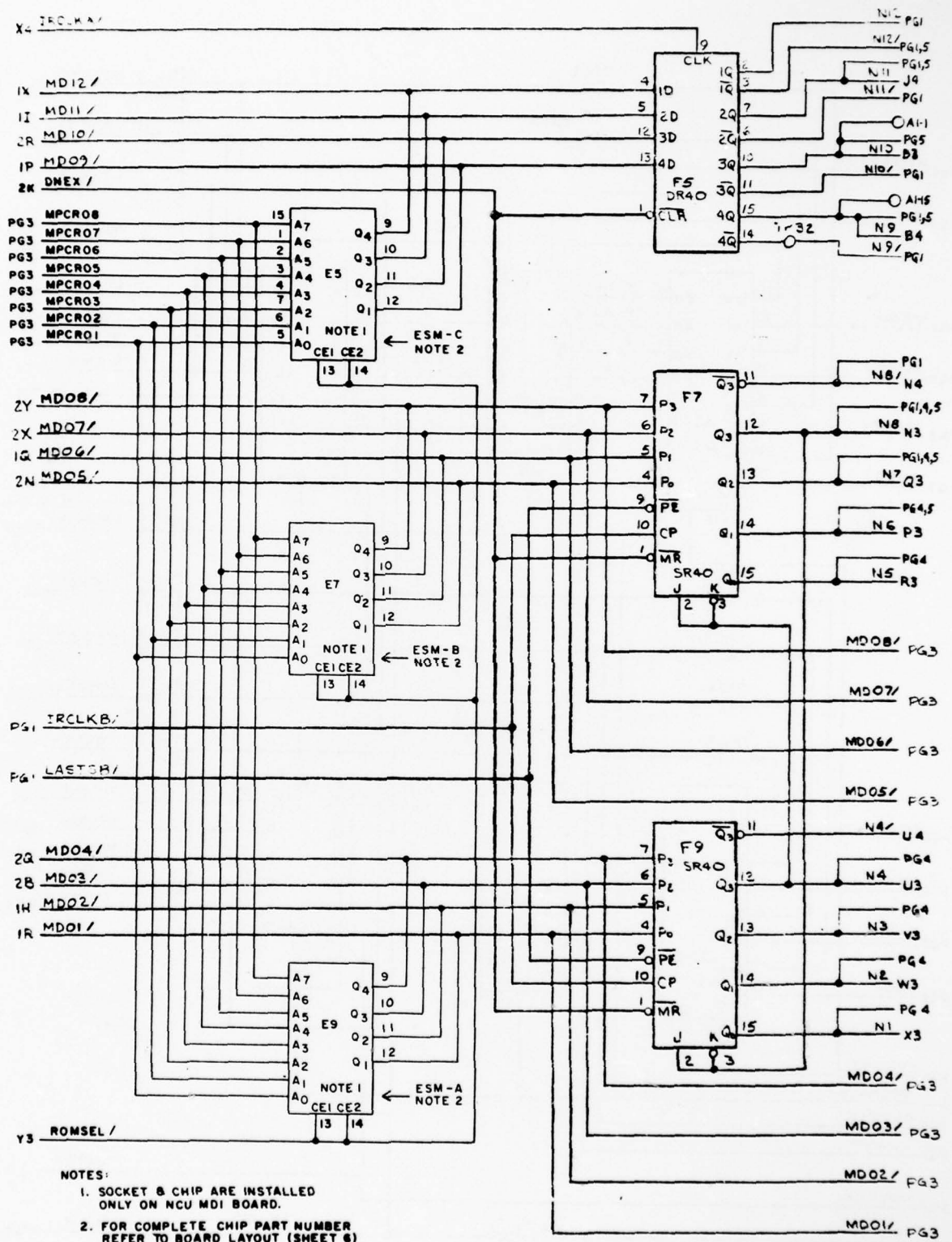
Figure 5-12. NCU and CIE MD1 Board Logic (Sheet 2 of 5)
