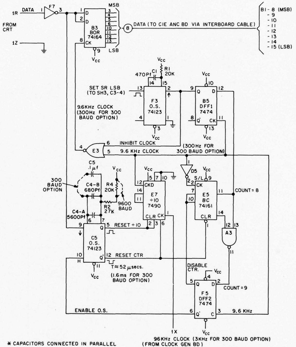
Figure 5-36. CRT Interface Board Buffer Logic (Sheet 1 of 3)
