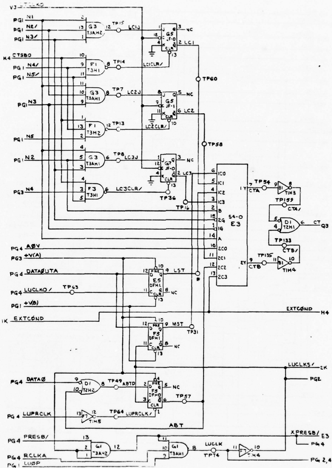
Figure 5-14. NCU and CIE MD2 Board Logic (Sheet 5 of 5)
