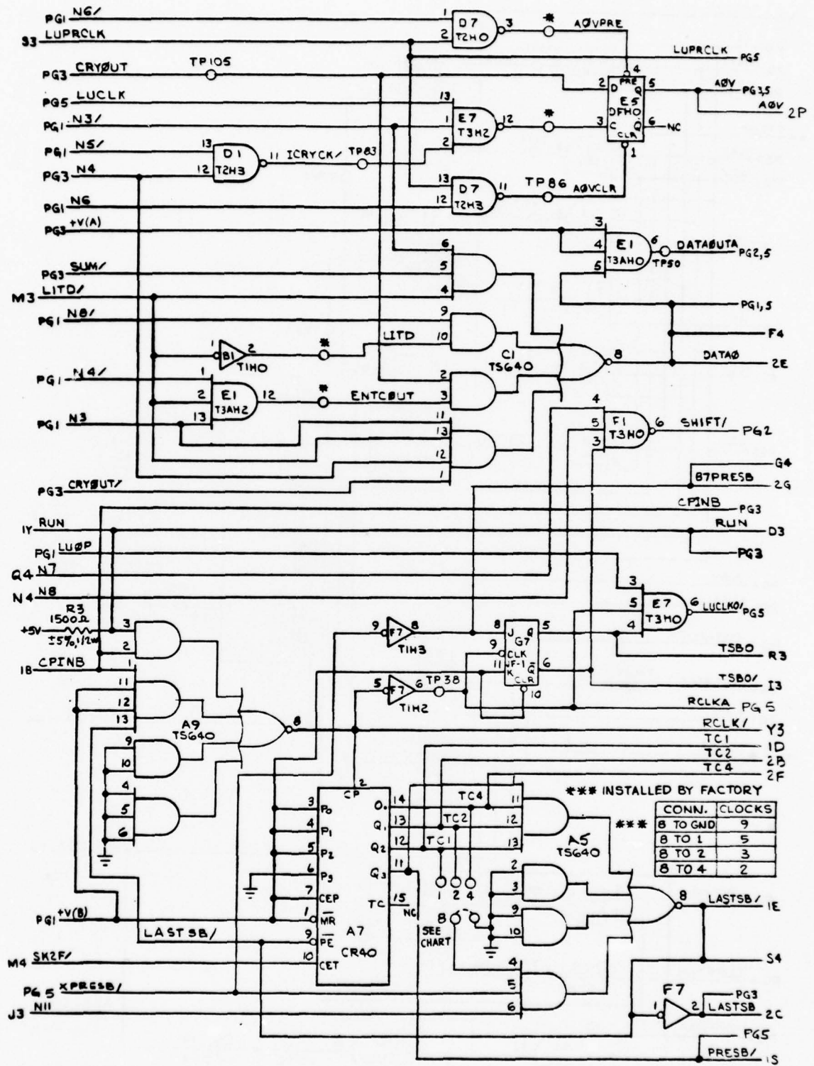
Figure 5-14. NCU and CIE MD2 Board Logic (Sheet 4 of 5)
