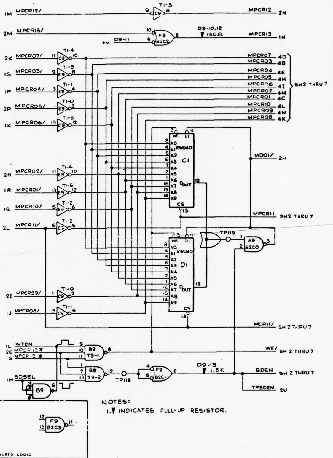
Figure 5-16. CIE Control Memory Logic (Sheet 1 of 7 Sheets)
