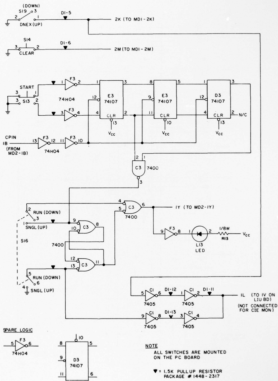
Figure 5-42. Monitor Board, Logic Diagram (Sheet 1 of 3)
