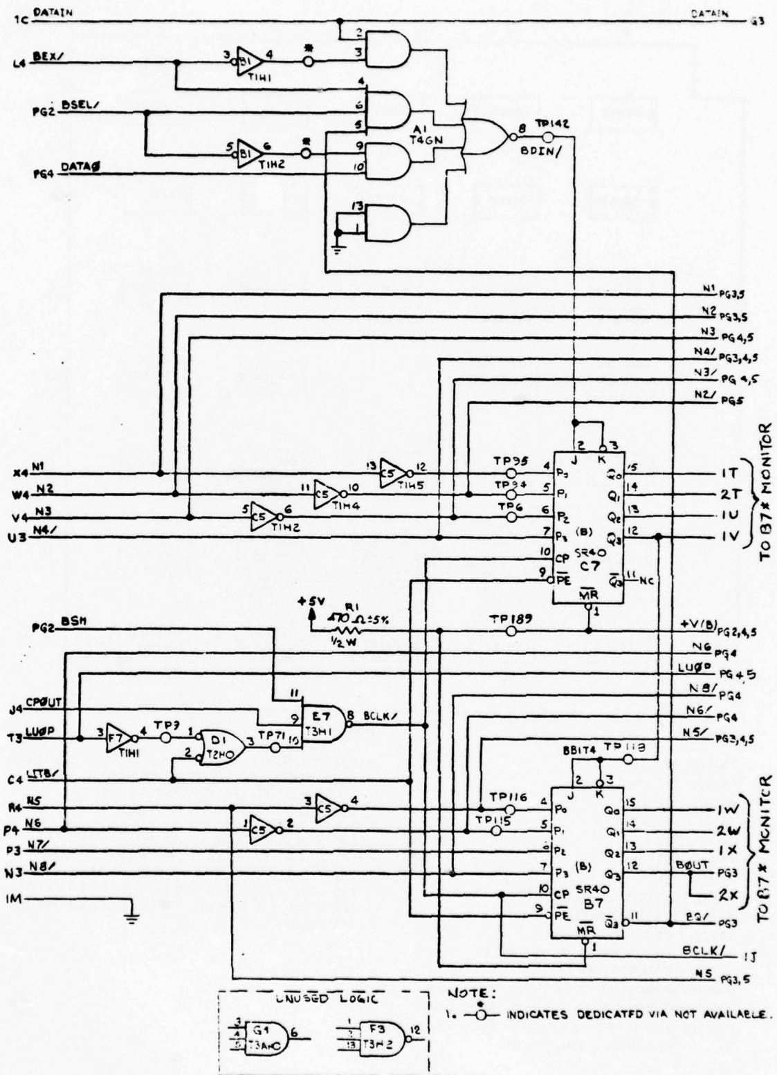
Figure 5-14. NCU and CIE MD2 Board Logic (Sheet 1 of 5)
