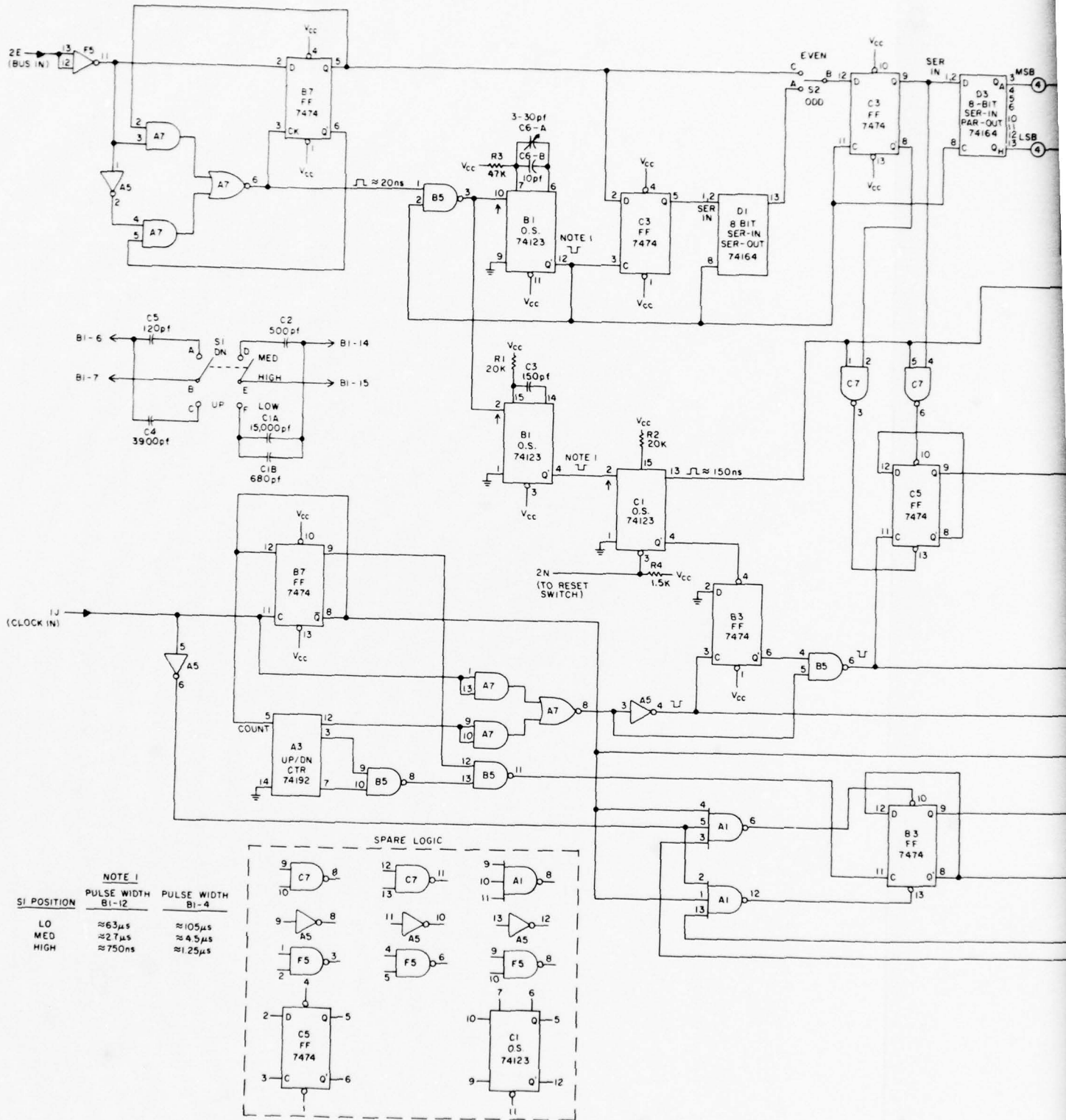
Figure 5- Logic I
