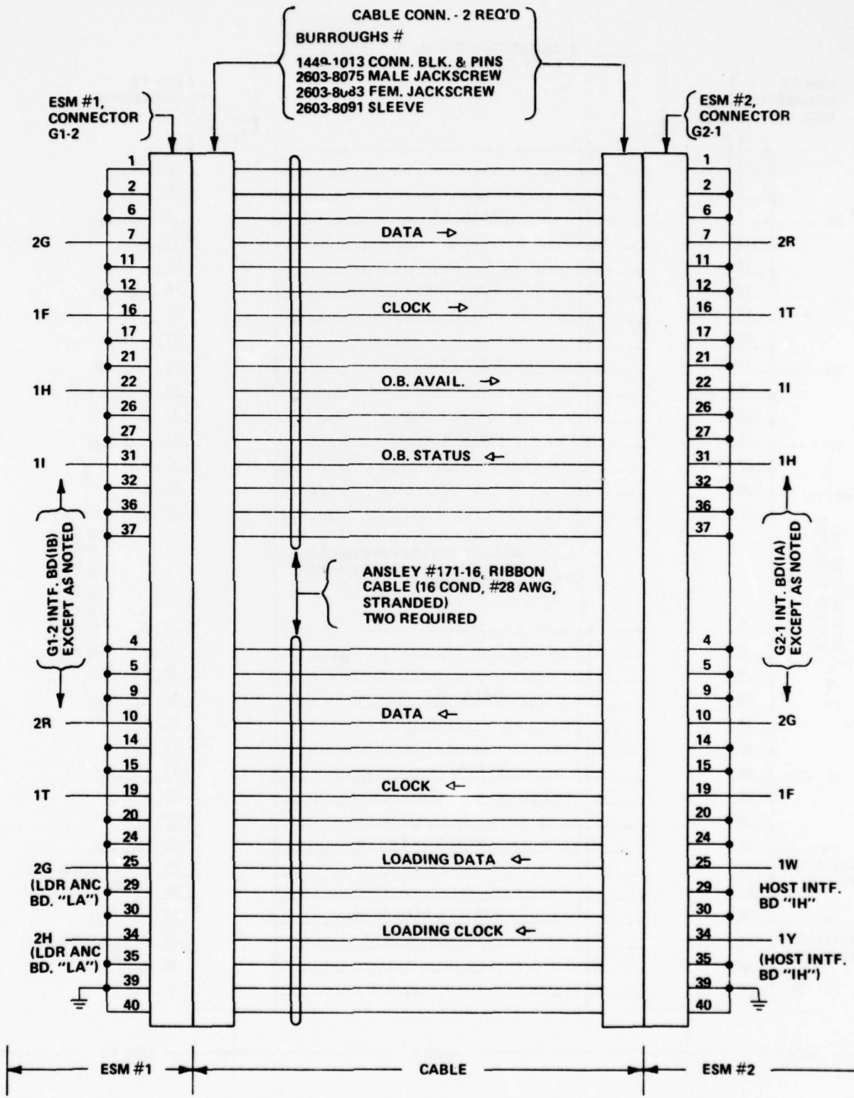
Figure 5-51. Cable, ESM No. 1 to ESM No. 2
