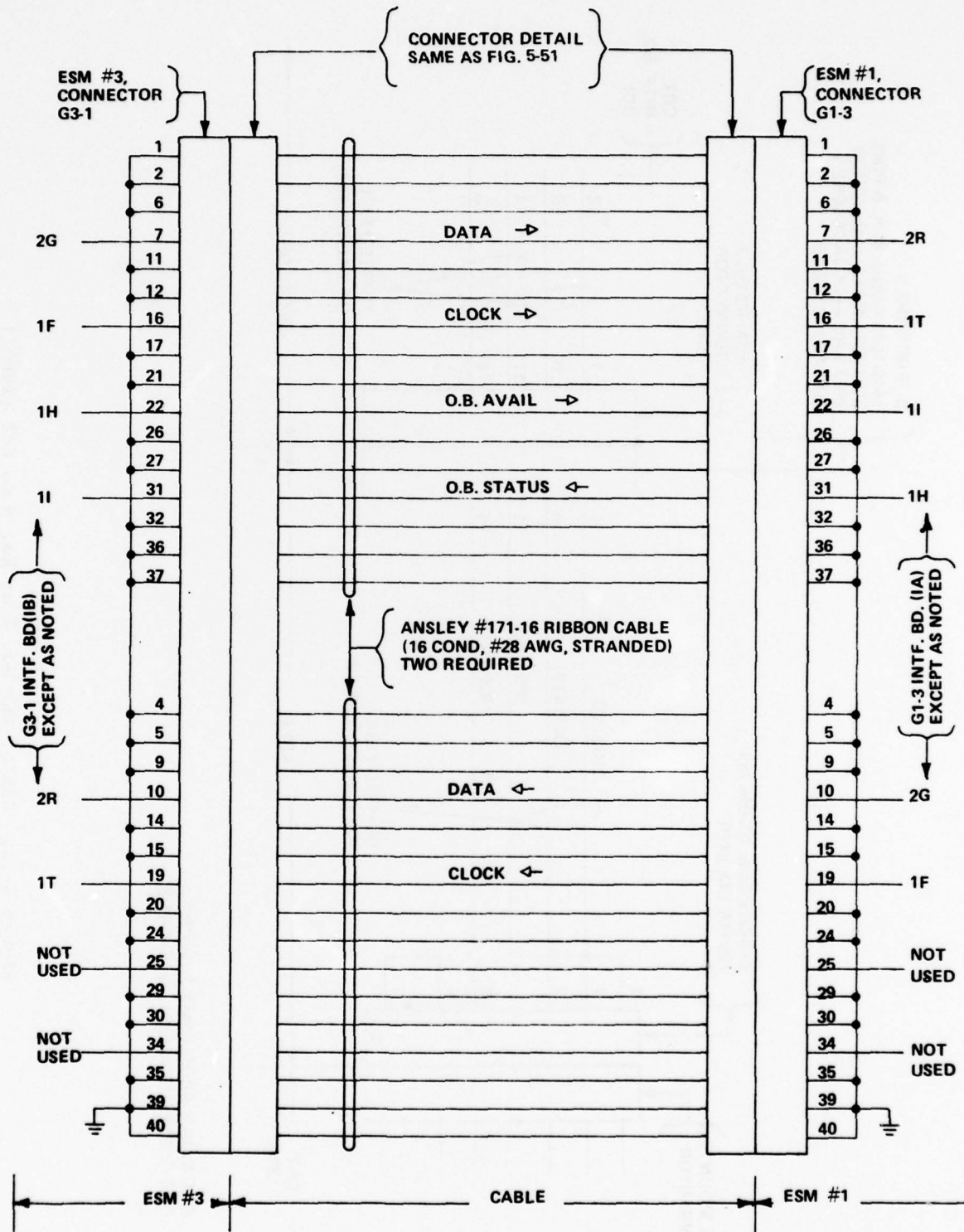
Figure 5-53. Cable, ESM No. 3 to ESM No. 1
