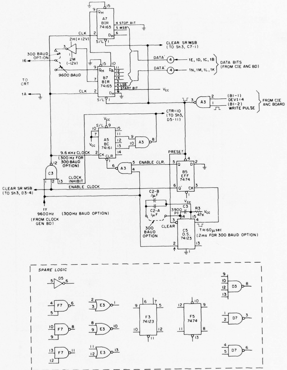
Figure 5-36. CRT Interface Board Buffer Logic (Sheet 2 of 3)
