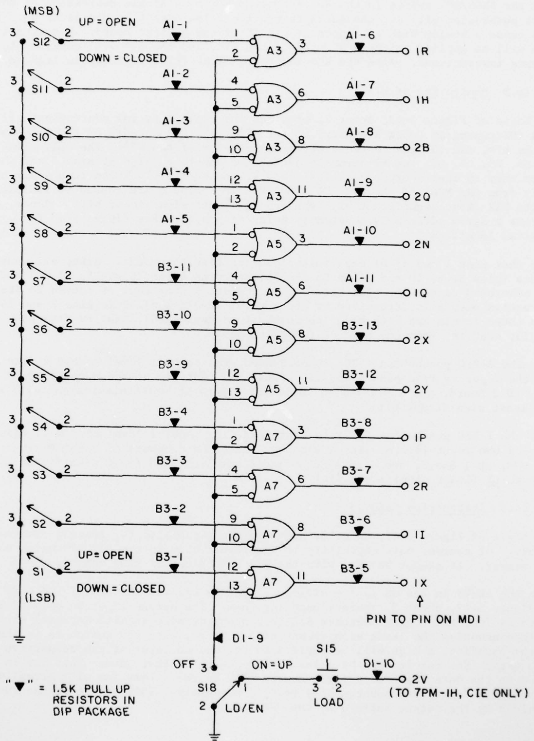
Figure 5-42. Monitor Board, Logic Diagram (Sheet 3 of 3)
