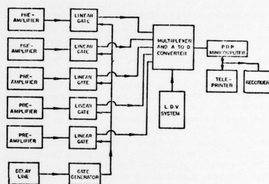
FIG.5 DATA ACQUISITION SYSTEM
