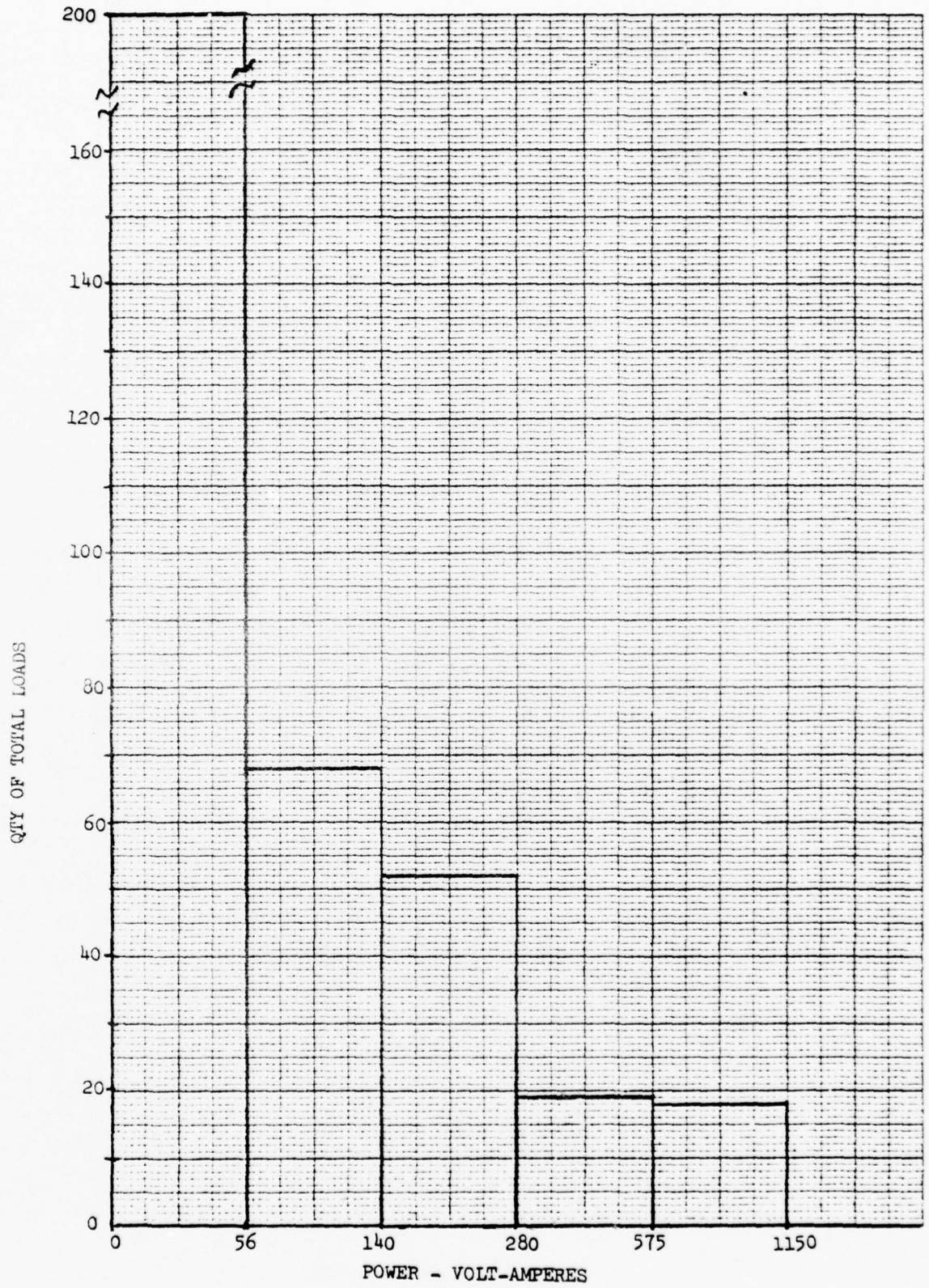
FIGURE 7 A-7 LOAD DISTRIBUTION VS REQUIRED POWER 299
