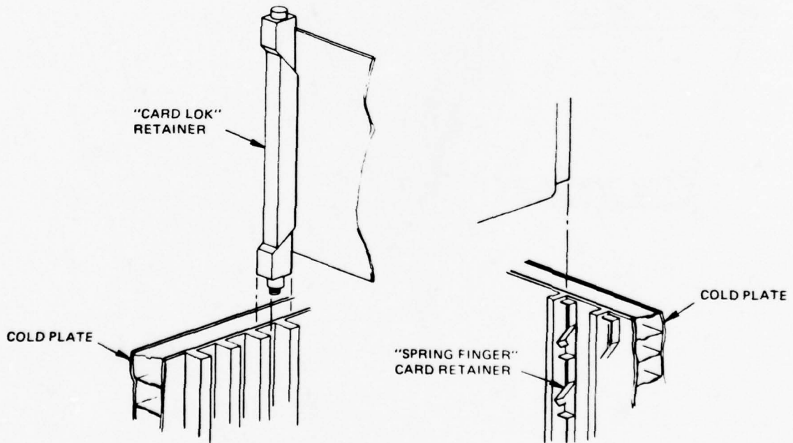
CONDUCTIVE COUPLING TO COLD PLATE
