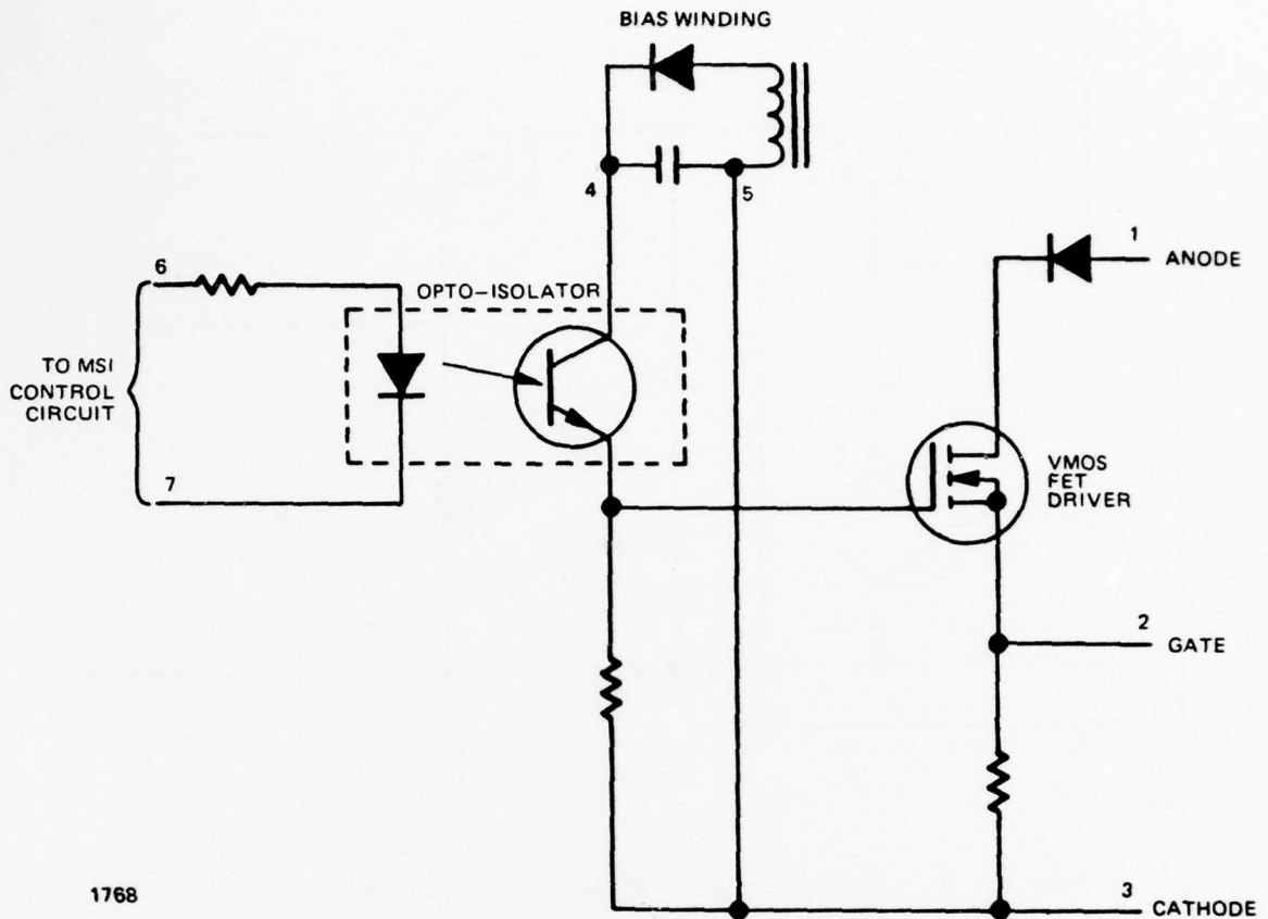
Figure 5. Recommended SCR Driver Circuit
