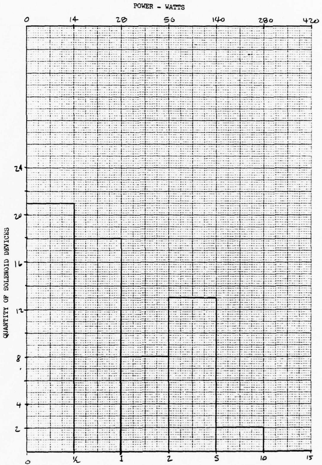
CURRENT - 28 VDC FIGURE 23 28VDC SOLENOID DEVICE LOAD DISTRIBUTION
