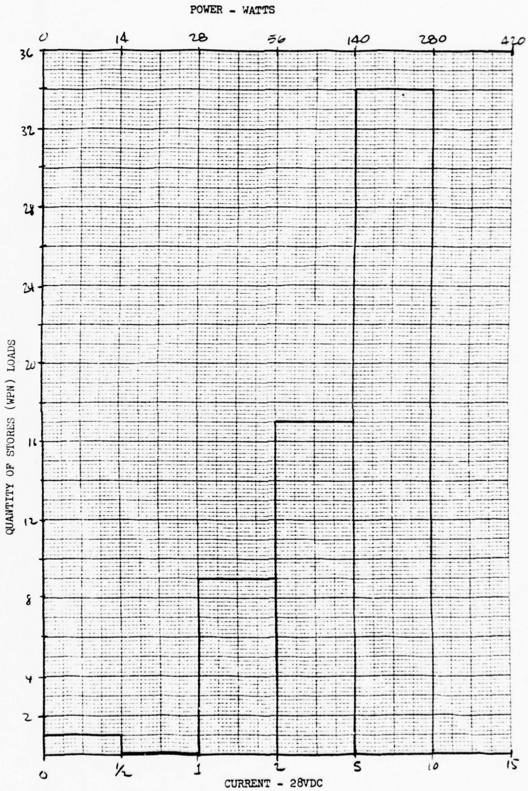
FIGURE 21 28VDC WEAPON LOAD DISTRIBUTION
