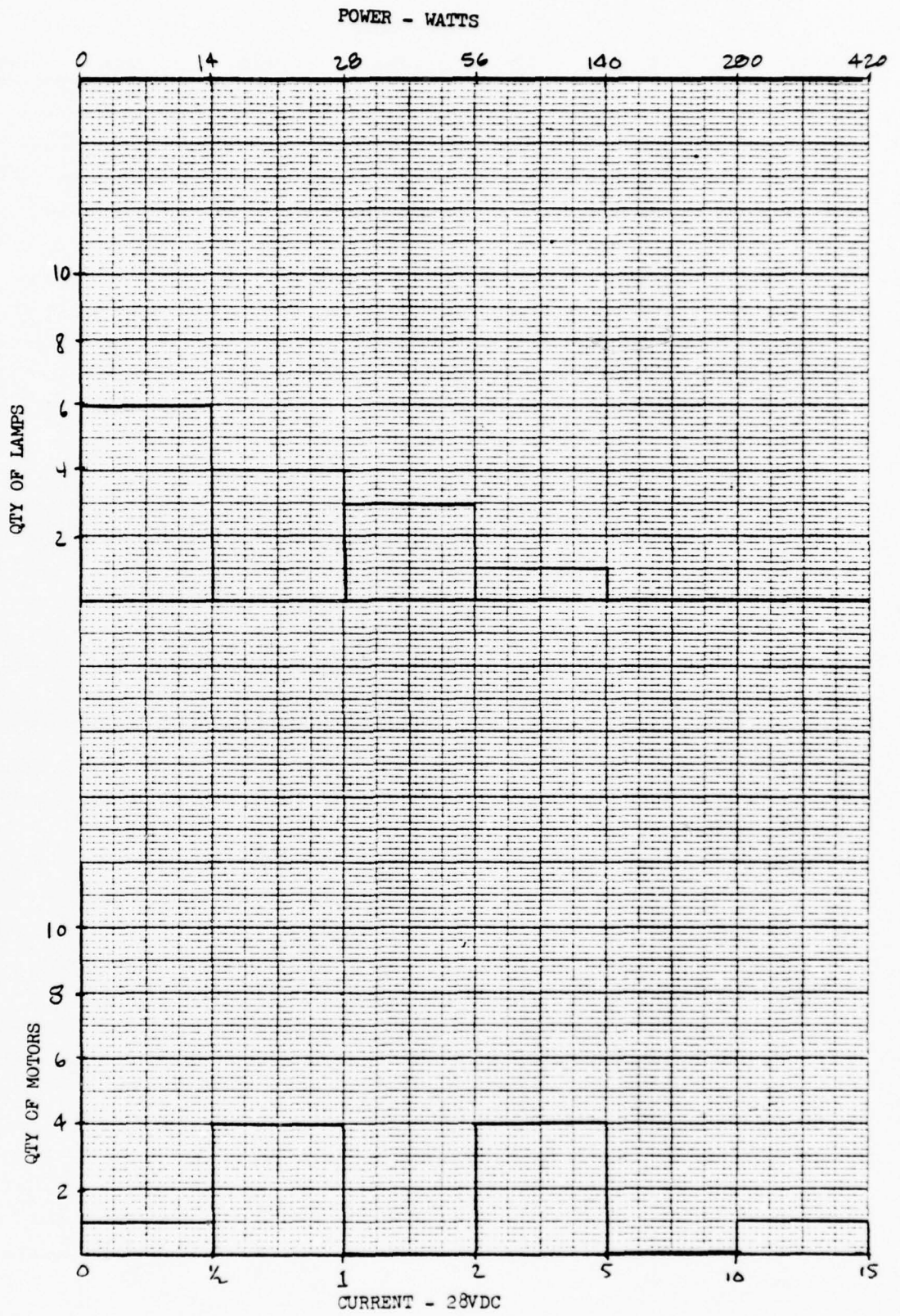
FIGURE 22 28VDC MOTOR AND LAMP LOAD DISTRIBUTION
