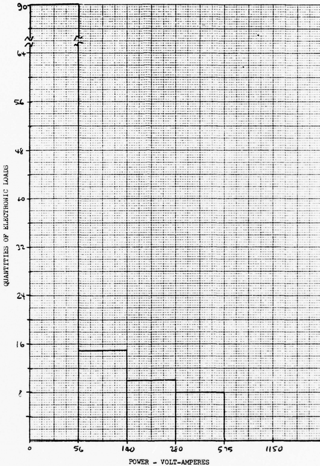
FIGURE 8 ELECTRONIC LRU LOAD DISTRIBUTION
