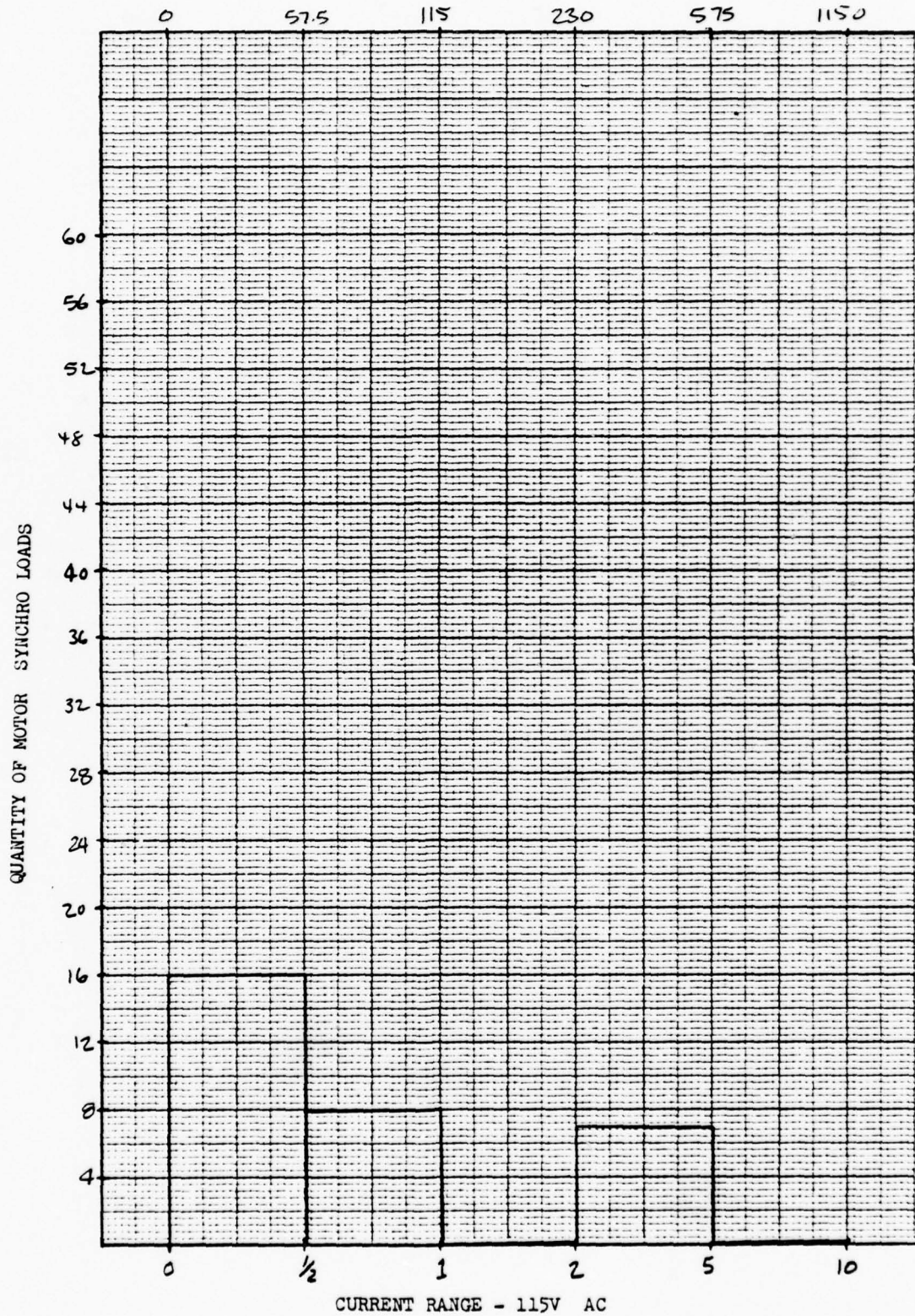
FIGURE 18 115VAC MOTOR LOAD DISTRIBUTION 311
