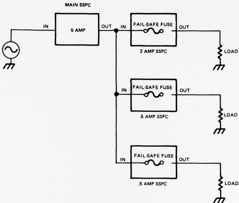
Figure 33. Cascading SSCP's for Protection of Several Small Loads
