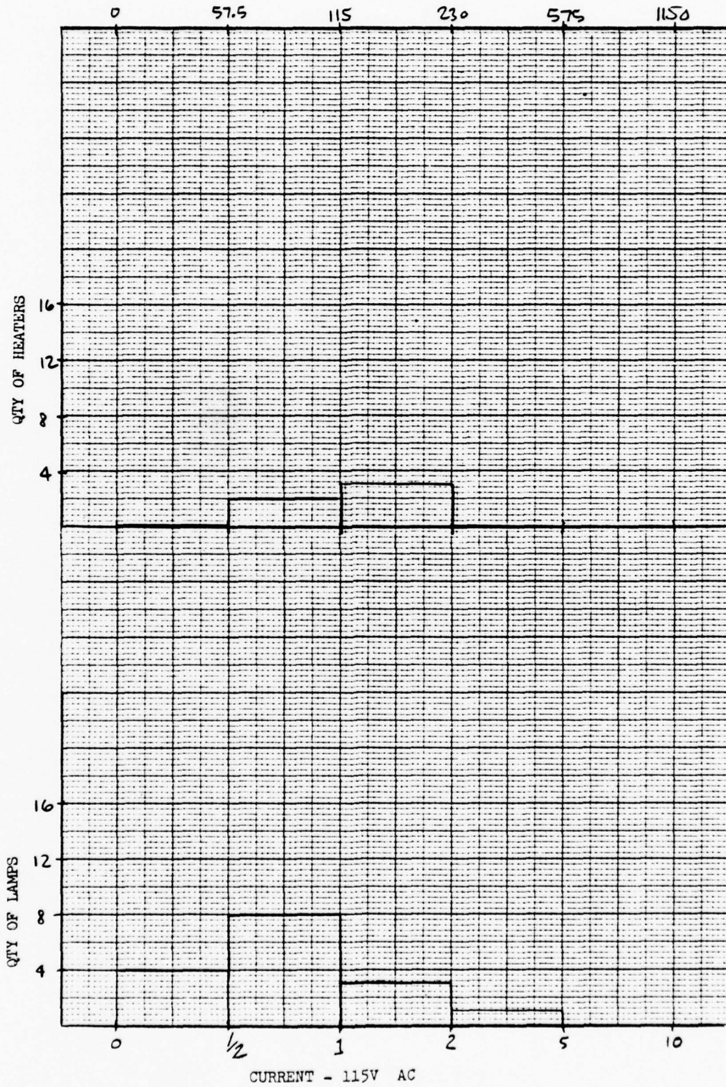
FIGURE 19 115VAC LAMP AND HEATER LOAD DISTRIBUTION 312
